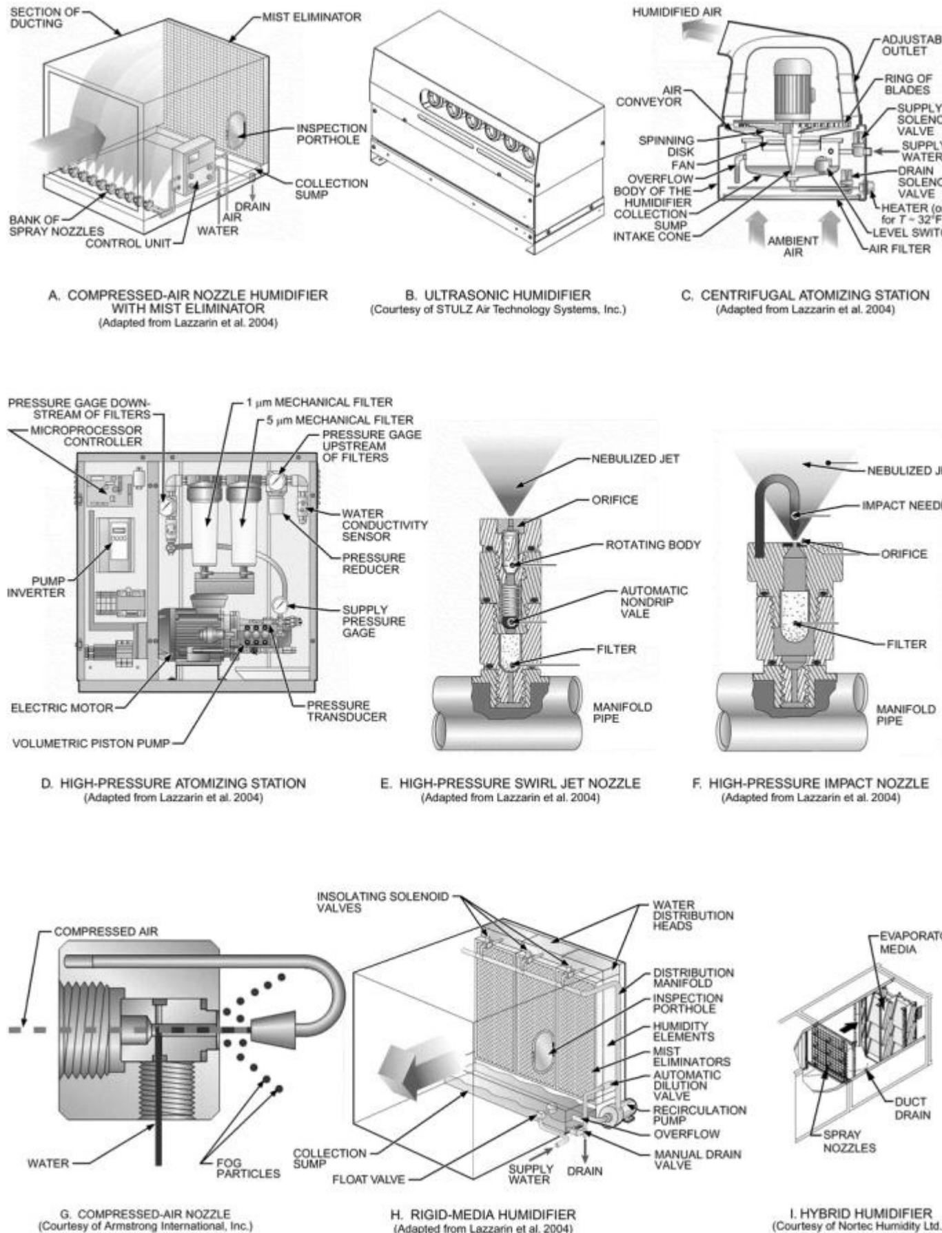
Figure 9. Industrial Adiabatic (Atomizing and Evaporative) Humidifiers
