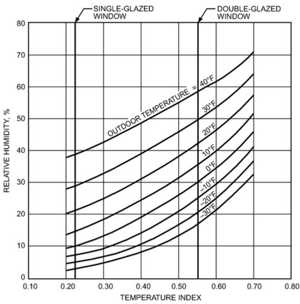
Figure 5. Limiting Relative Humidity for No Window Condensation
