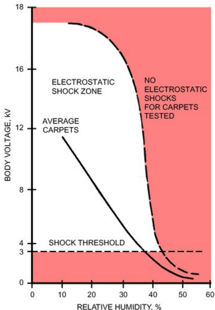
Figure 4. Effect of Relative Humidity on Static Electricity from Carpets
