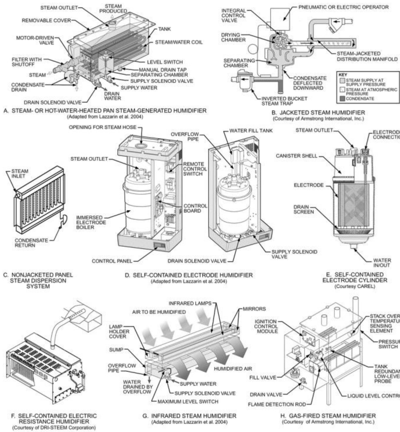
Figure 8. Industrial Isothermal (Steam) Humidifiers
