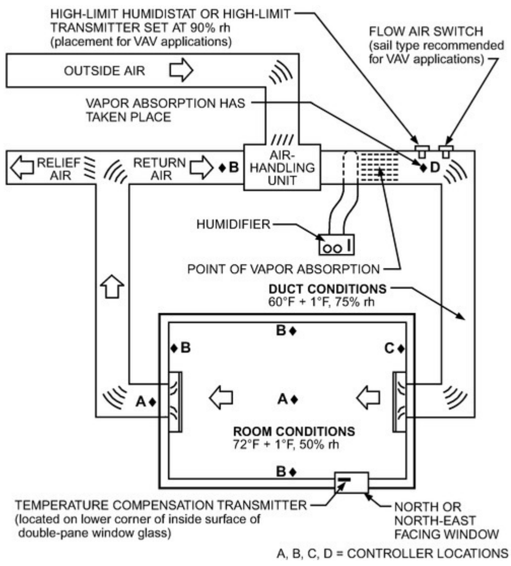
Figure 10. Recommended Humidity Controller Location
