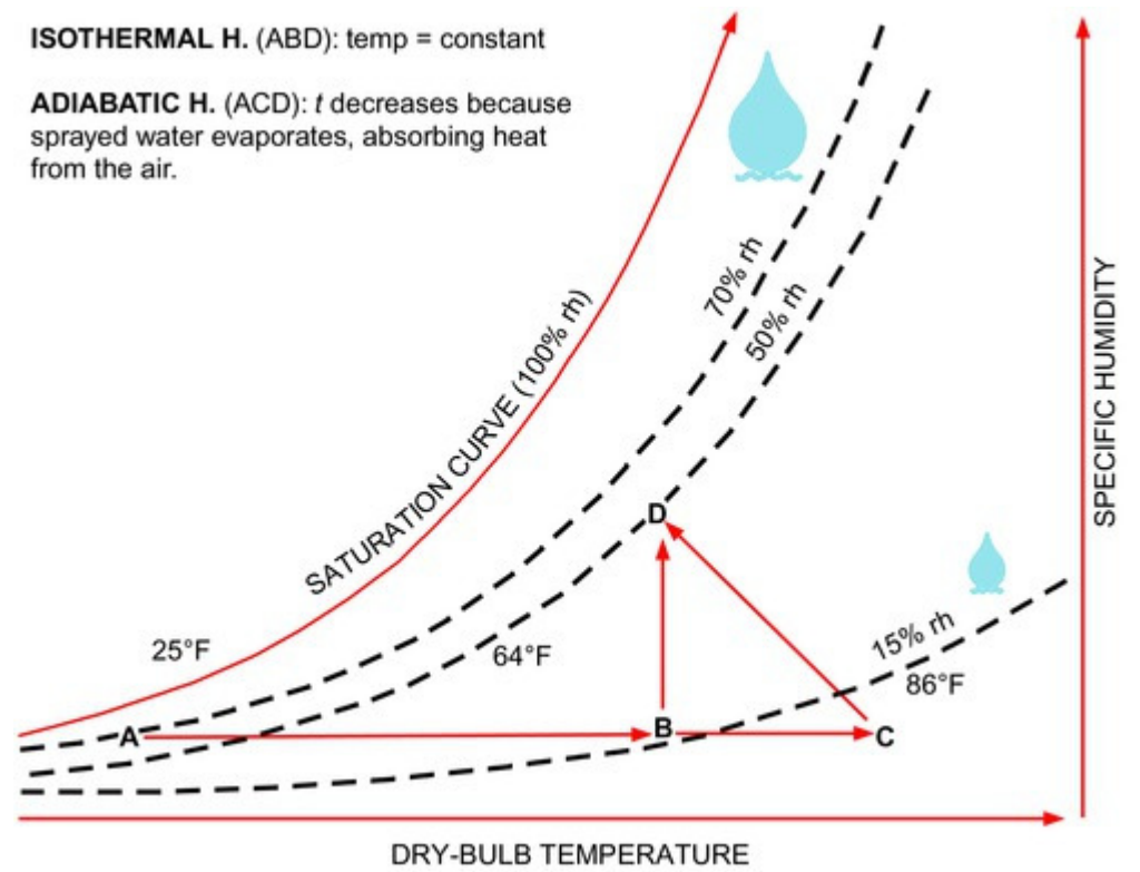
Figure 6. Adiabatic Versus Isothermal Humidification Process (Courtesy CAREL)
