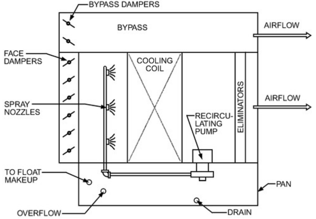
Figure 6. Sprayed-Coil System with Air Bypass
