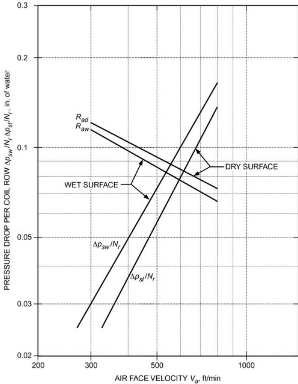
Figure 12. Typical Air-Side Application Rating Data Determined Experimentally for Cooling and Dehumidifying Water Coils
