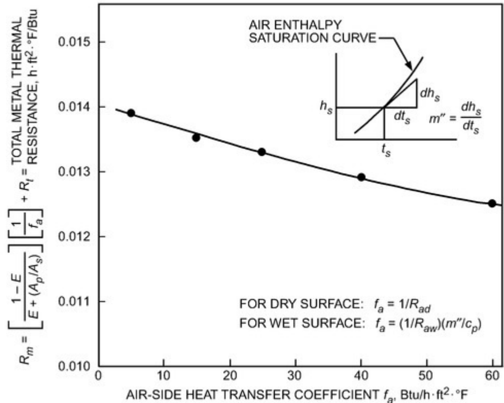
Figure 11. Typical Total Metal Thermal Resistance of Fin and Tube Assembly
