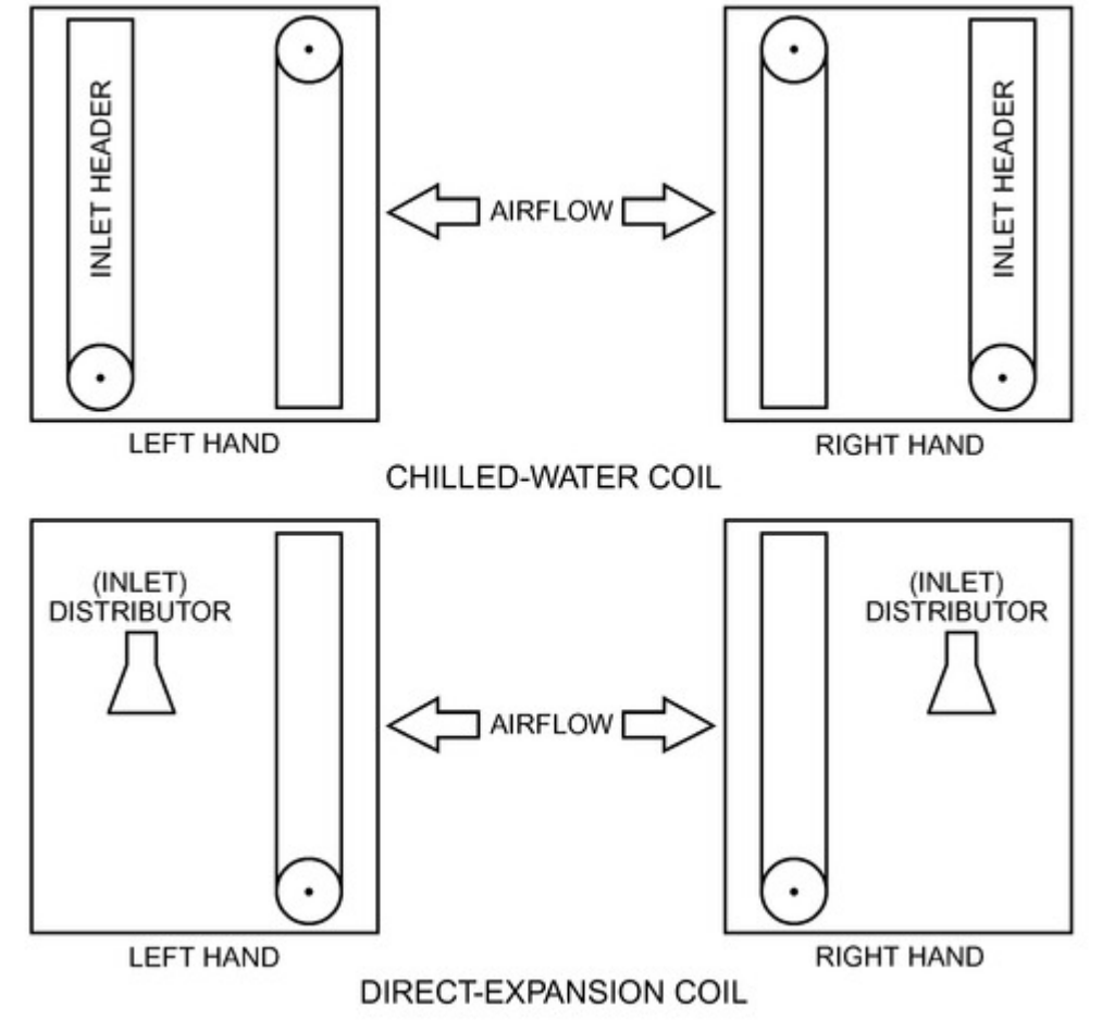
Figure 3. Typical Coil Hand Designation
