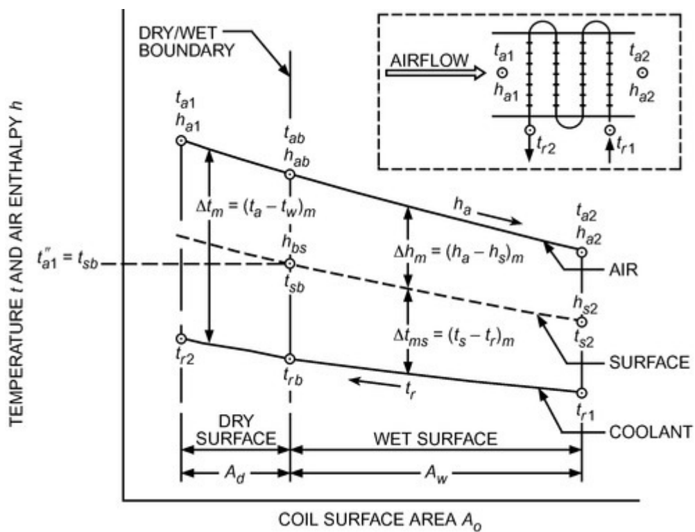
Figure 9. Thermal Diagram for General Case When Coil Surface Operates Partially Dry
