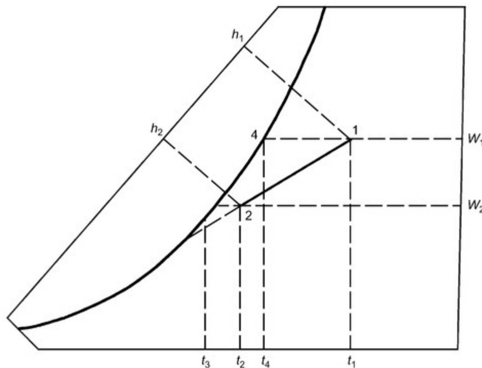
Figure 13. Psychrometric Performance of Cooling and Dehumidifying Coil
