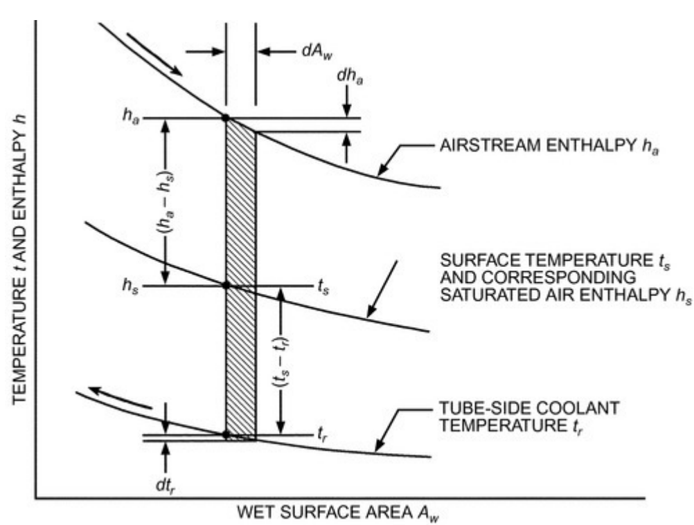
Figure 7. Two-Component Driving Force Between Dehumidifying Air and Coolant
