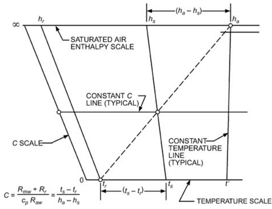
Figure 8. Surface Temperature Chart
