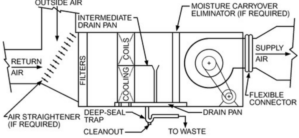
Figure 4. Typical Arrangement of Cooling Coil Assembly in Built-Up or Packaged Central Station Air Handler
