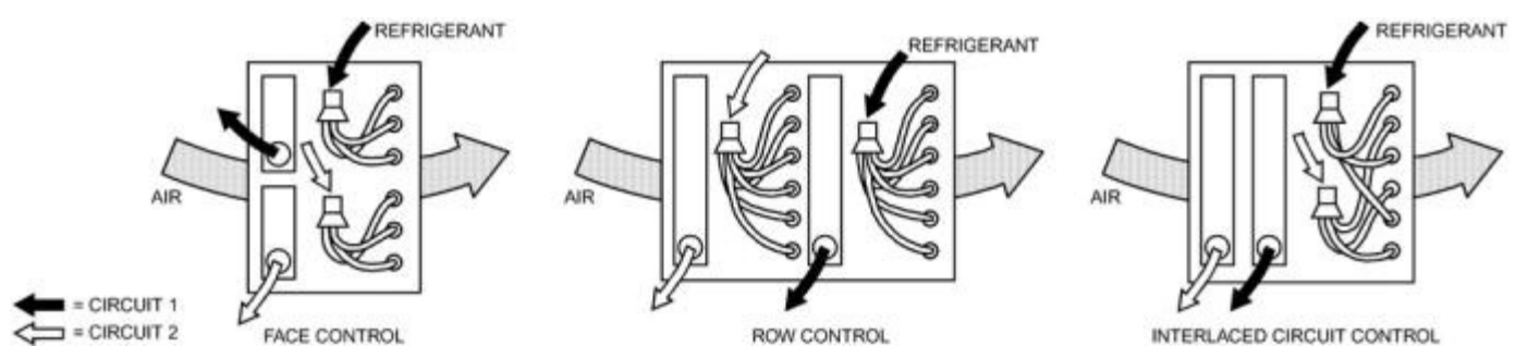
Figure 2. Arrangements for Coils with Multiple Thermostatic Expansion Valves
