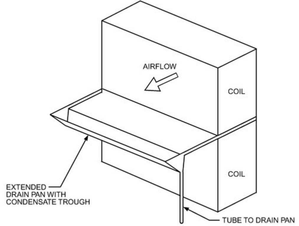
Figure 5. Coil Bank Arrangement with Intermediate Condensate Pan
