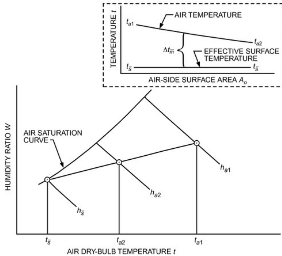
Figure 10. Leaving-Air Dry-Bulb Temperature Determination for Air-Cooling and Dehumidifying Coils
