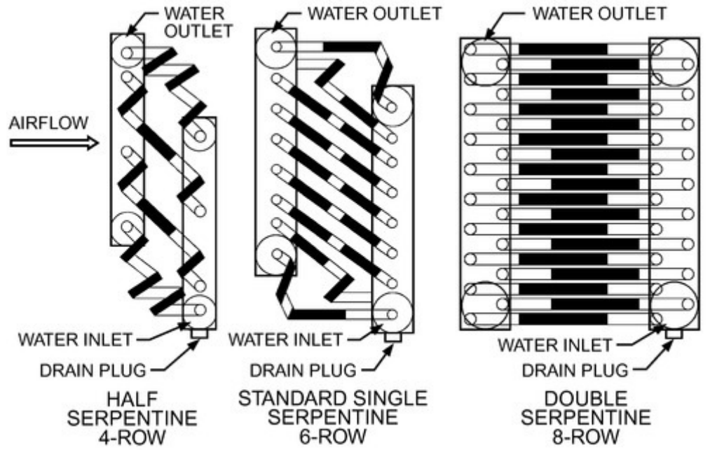
Figure 1. Typical Water Circuit Arrangements
