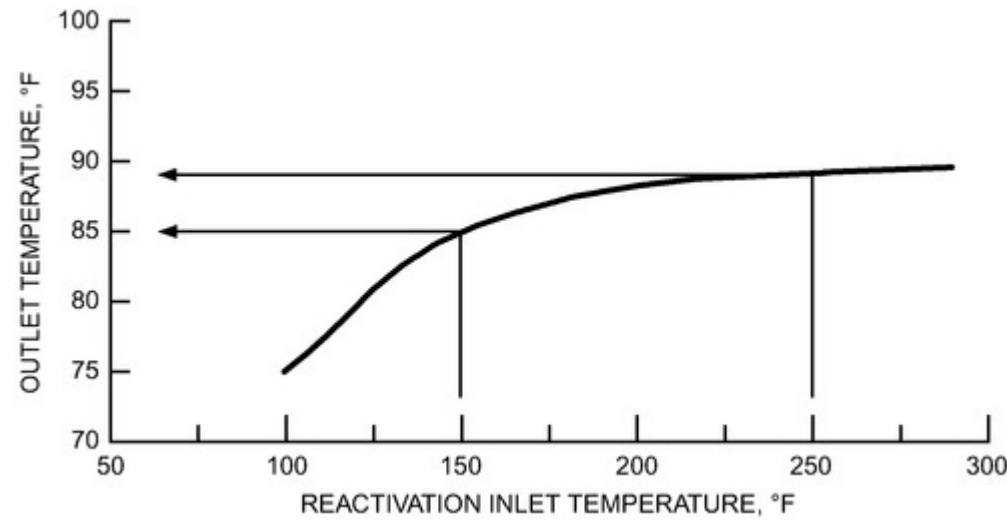
Figure 12. Effect of Changes in Reactivation Air Inlet Temperature on Dehumidifier Outlet Temperature
