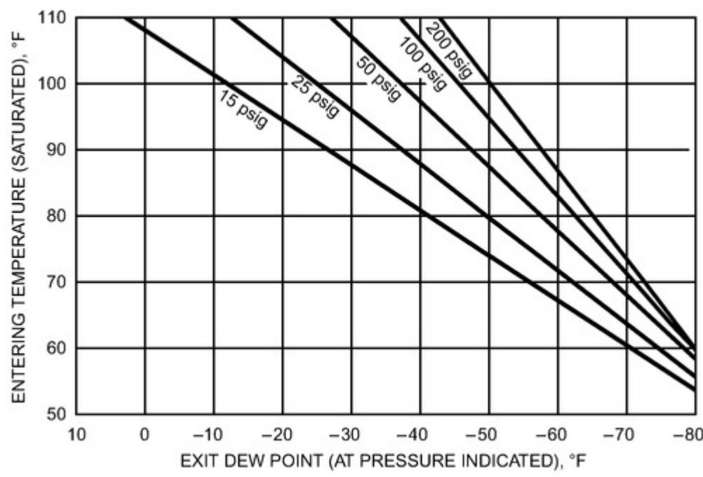
Figure 17. Typical Performance Data for Solid Desiccant Dryers at Elevated Pressures
