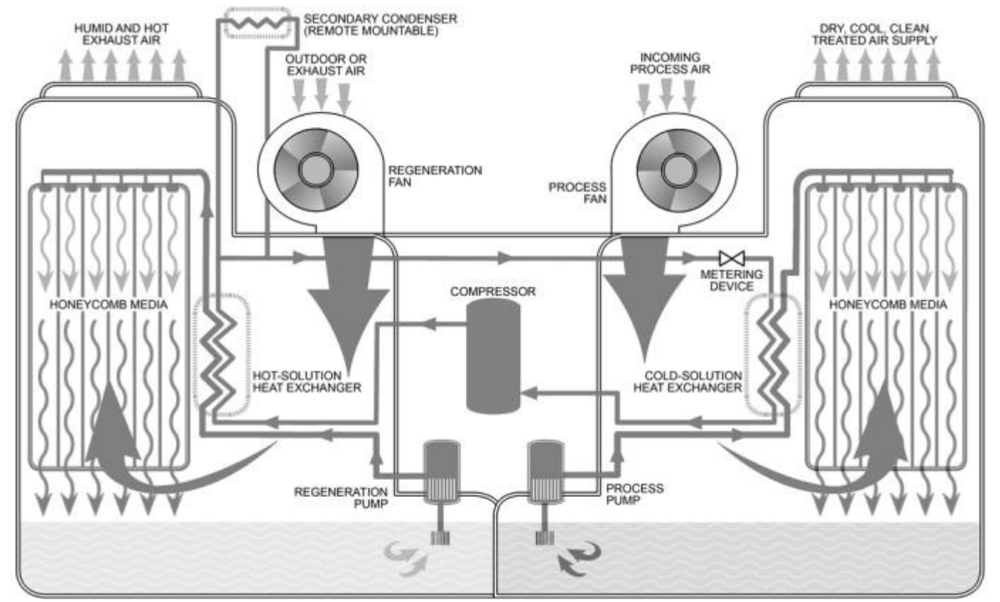
Figure 3. Flow Diagram for Liquid-Absorbent Unit with Onboard Refrigeration System
