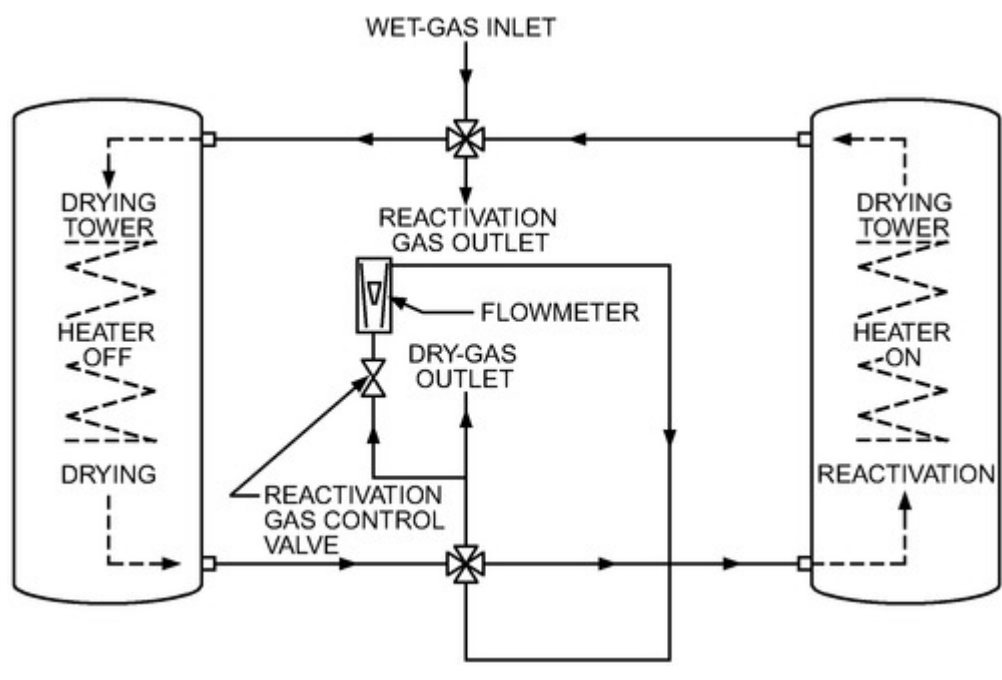
Figure 18. Typical Adsorption Dryer for Elevated Pressures
