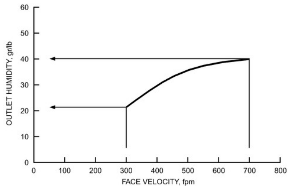
Figure 8. Effect of Changes in Process Air Velocity on Dehumidifier Outlet Moisture
