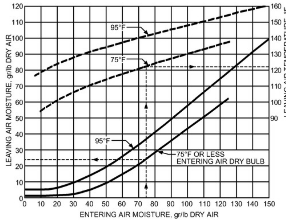
Figure 13. Typical Performance Data for Rotary Solid Desiccant Dehumidifier 2.4 EQUIPMENT RATINGS
