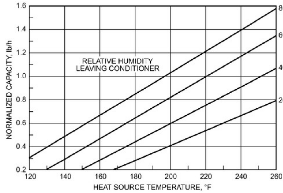
Figure 6. Liquid Desiccant Regenerator Capacity
