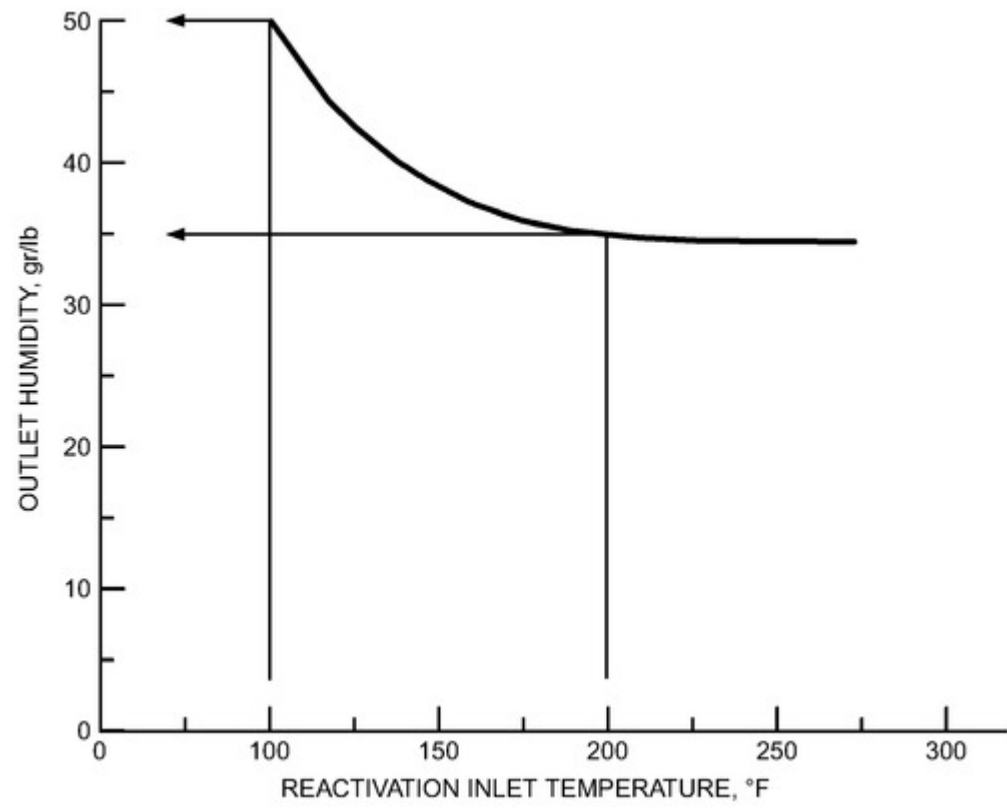
Figure 10. Effect of Changes in Reactivation Air Inlet Temperature on Dehumidifier Outlet Moisture
