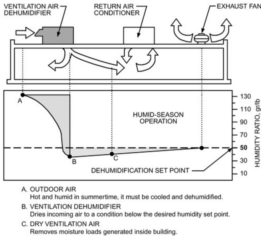
Figure 15. Predrying Ventilation Air to Dehumidify a Commercial Building (Harriman et al. 2001)
