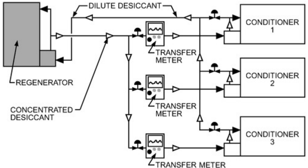
Figure 5. Liquid Desiccant System with Multiple Conditioners
