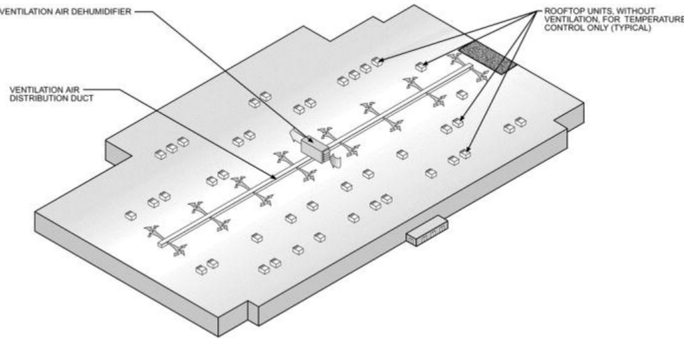
Figure 16. Typical Rooftop Arrangement for Drying Ventilation Air Centrally, Removing Moisture Load from Cooling Units (Harriman et al. 2001)
