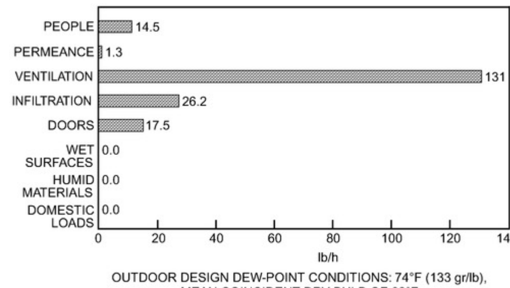
Figure 14. Typical Peak Moisture Loads for Medium-Sized Retail Store in Atlanta, Georgia (Harriman et al. 2001)
