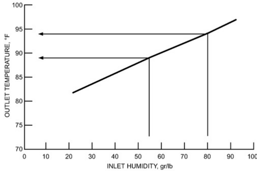
Figure 11. Effect of Changes in Process Air Inlet Moisture on Dehumidifier Outlet Temperature
