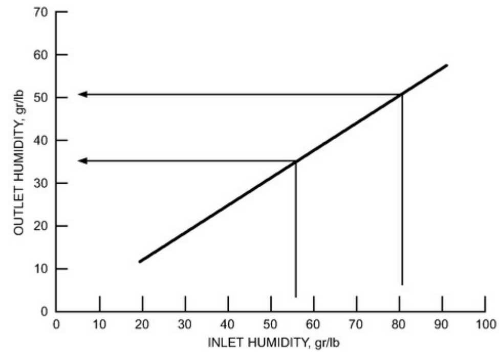
Figure 9. Effect of Changes in Process Air Inlet Moisture on Dehumidifier Outlet Moisture
