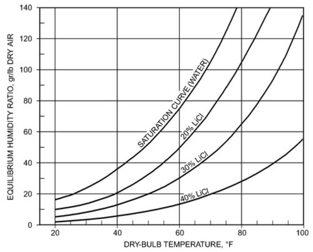
Figure 4. Lithium Chloride Equilibrium
