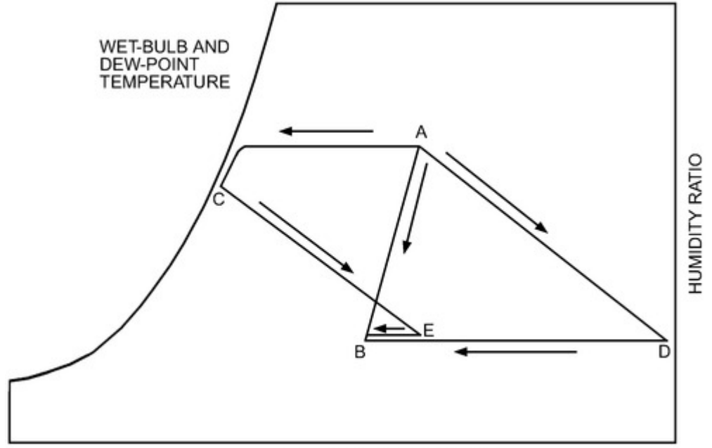
Figure 1. Methods of Dehumidification
