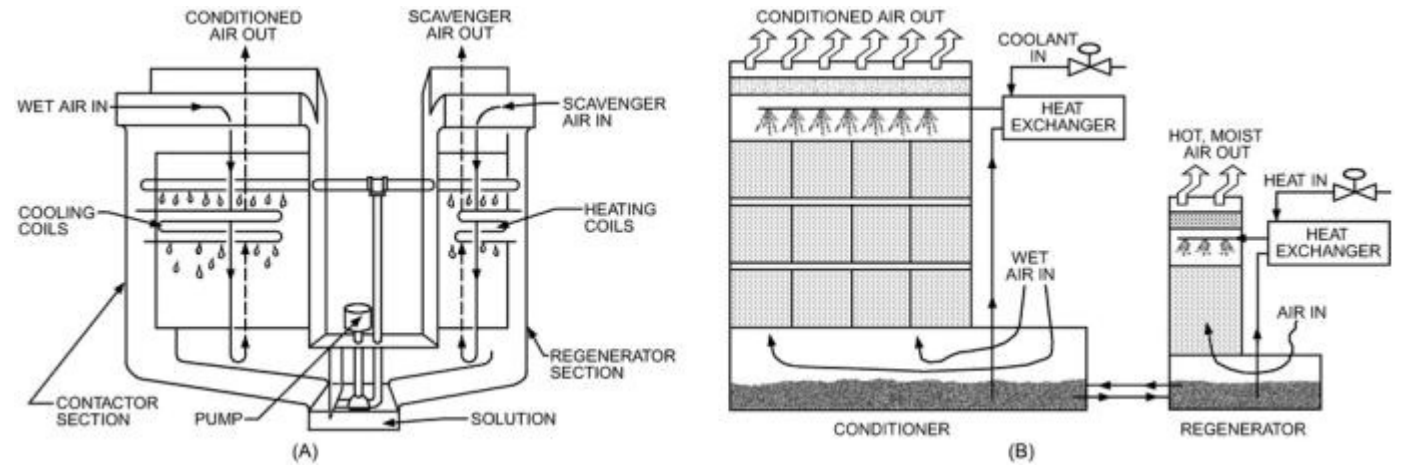
Figure 2. Flow Diagram for Liquid-Absorbent Dehumidifier (A) Without and (B) With Extended Surface Contact Medium
