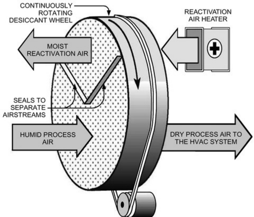
Figure 7. Typical Rotary Dehumidification Wheel
