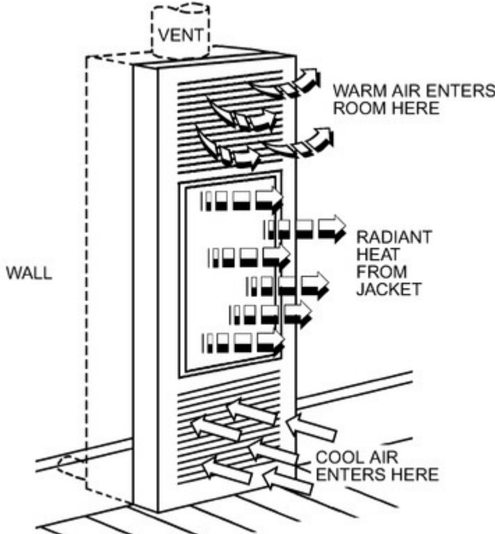
Figure 2. Wall Furnace
