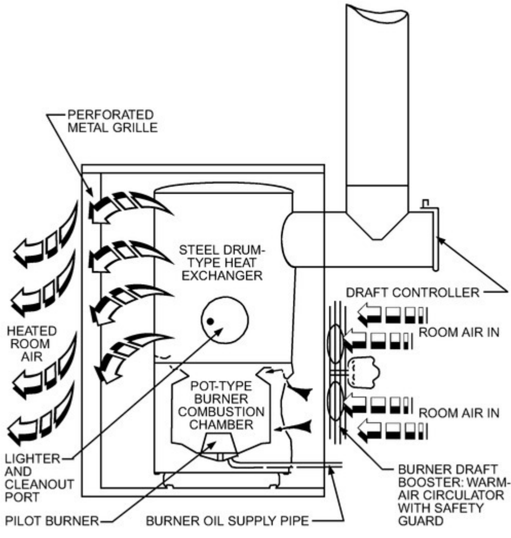
Figure 4. Oil-Fueled Heater with Vaporizing Pot-Type Burner
