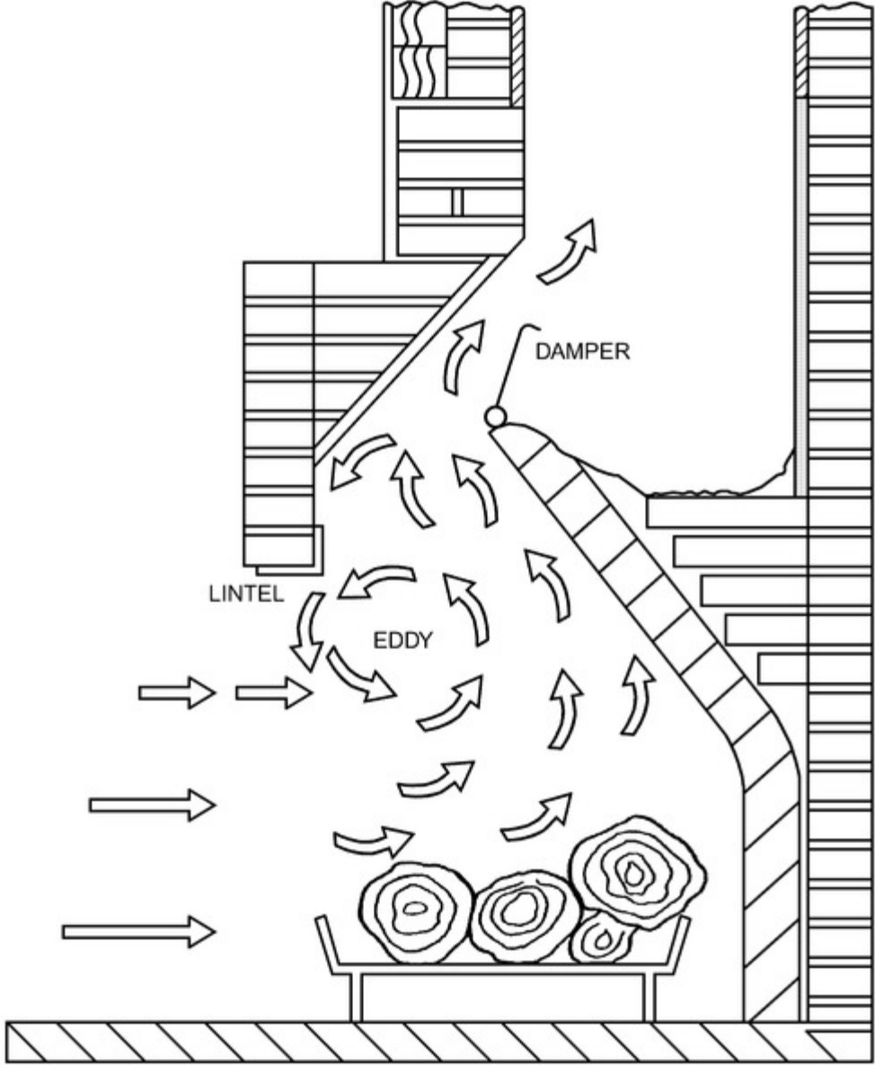
Figure 18. Eddy Formation
