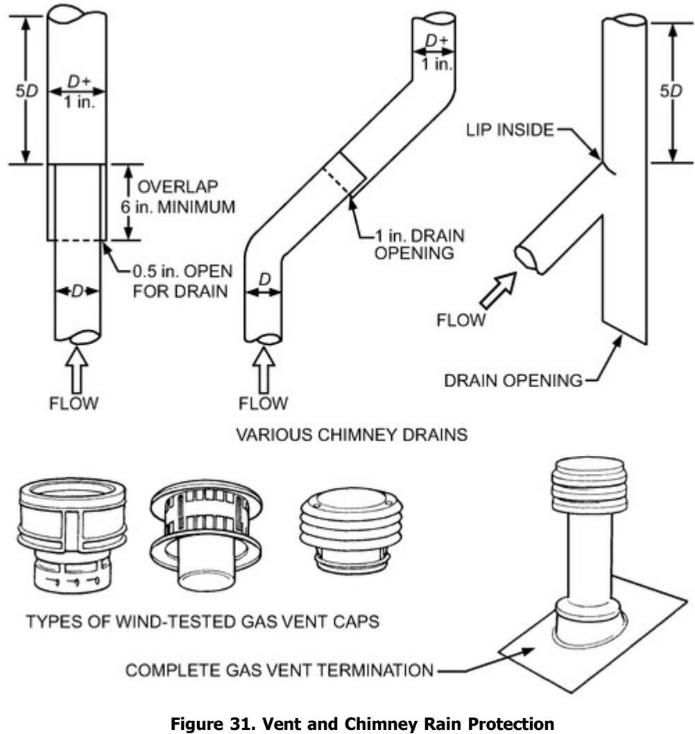
Figure 31. Vent and Chimney Rain Protection
