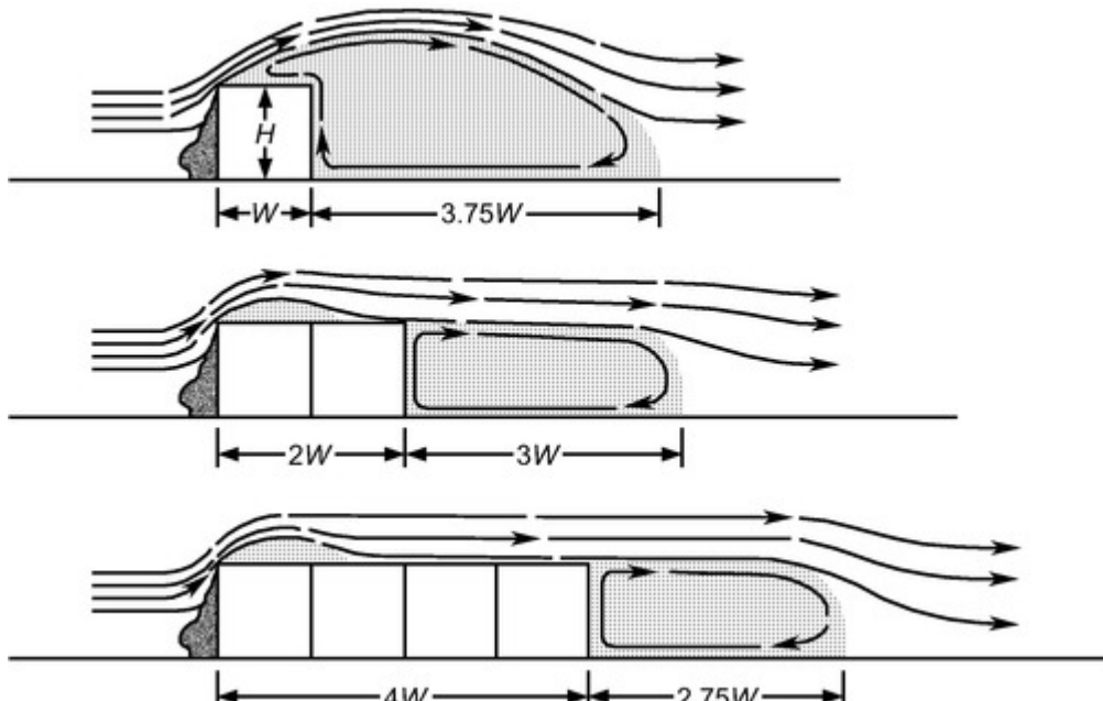
Figure 30. Eddy and Wake Zones for Low, Wide Buildings
