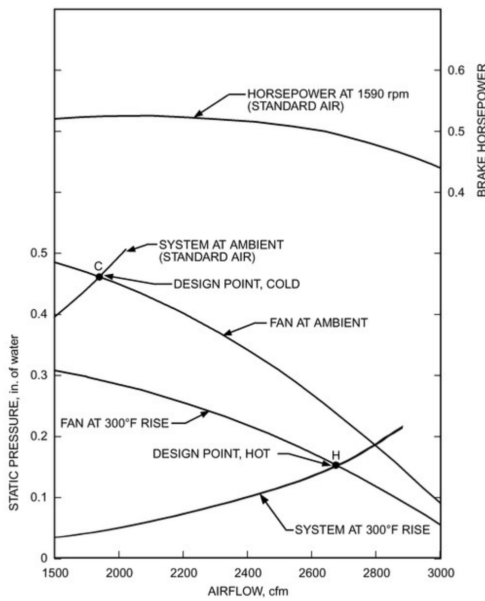
Figure 17. Typical Fan Operating Data and System Curves
