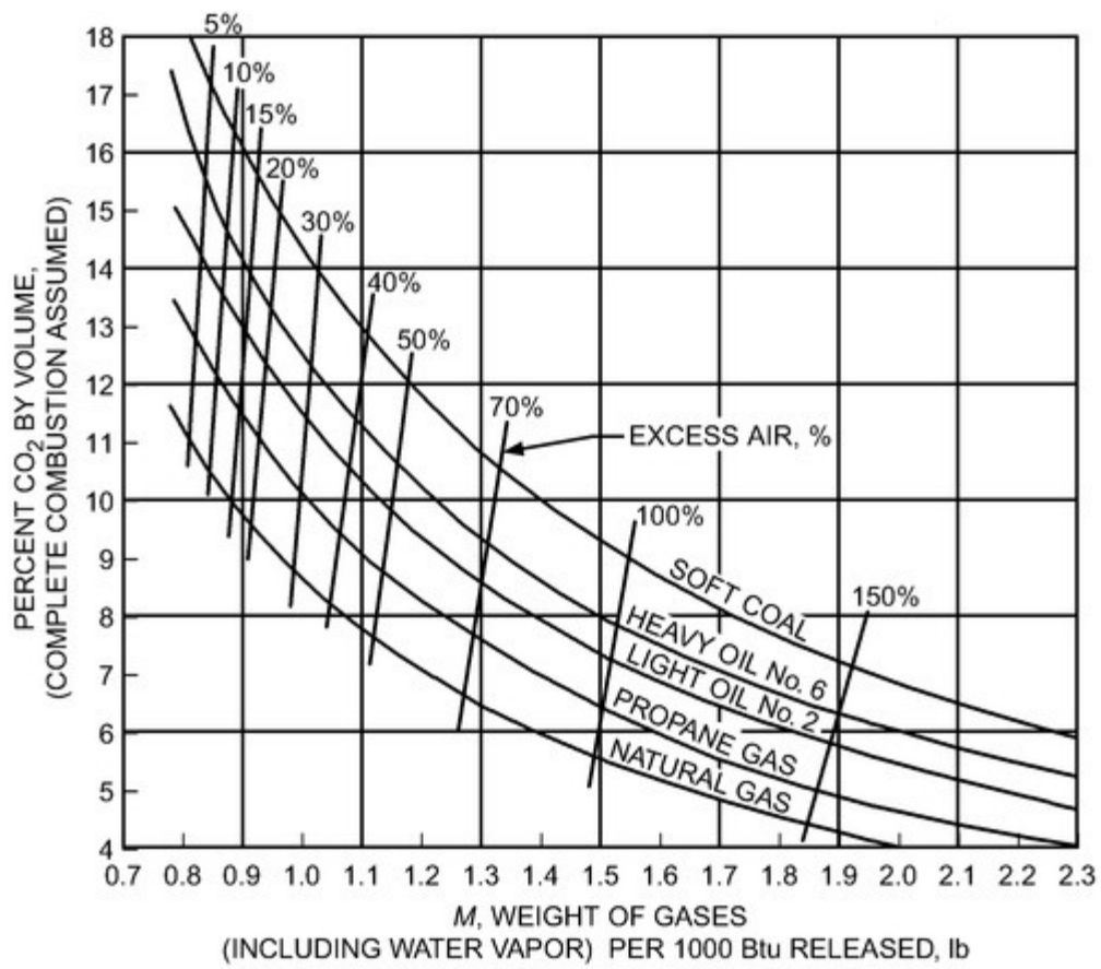
Figure 1. Graphical Evaluation of Rate of Vent Gas Flow from Percent CO 2 and Fuel Rate
