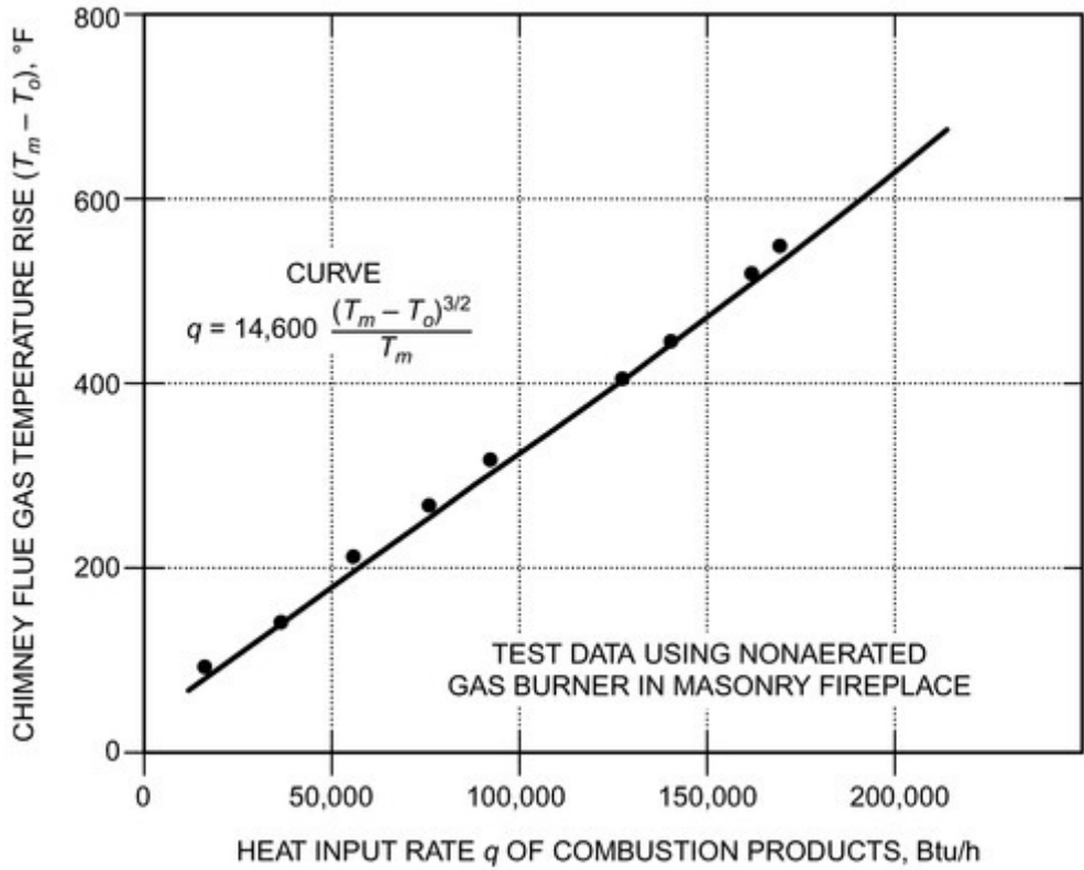
Figure 22. Variation of Chimney Flue Gas Temperature with Heat Input Rate of Combustion Products
