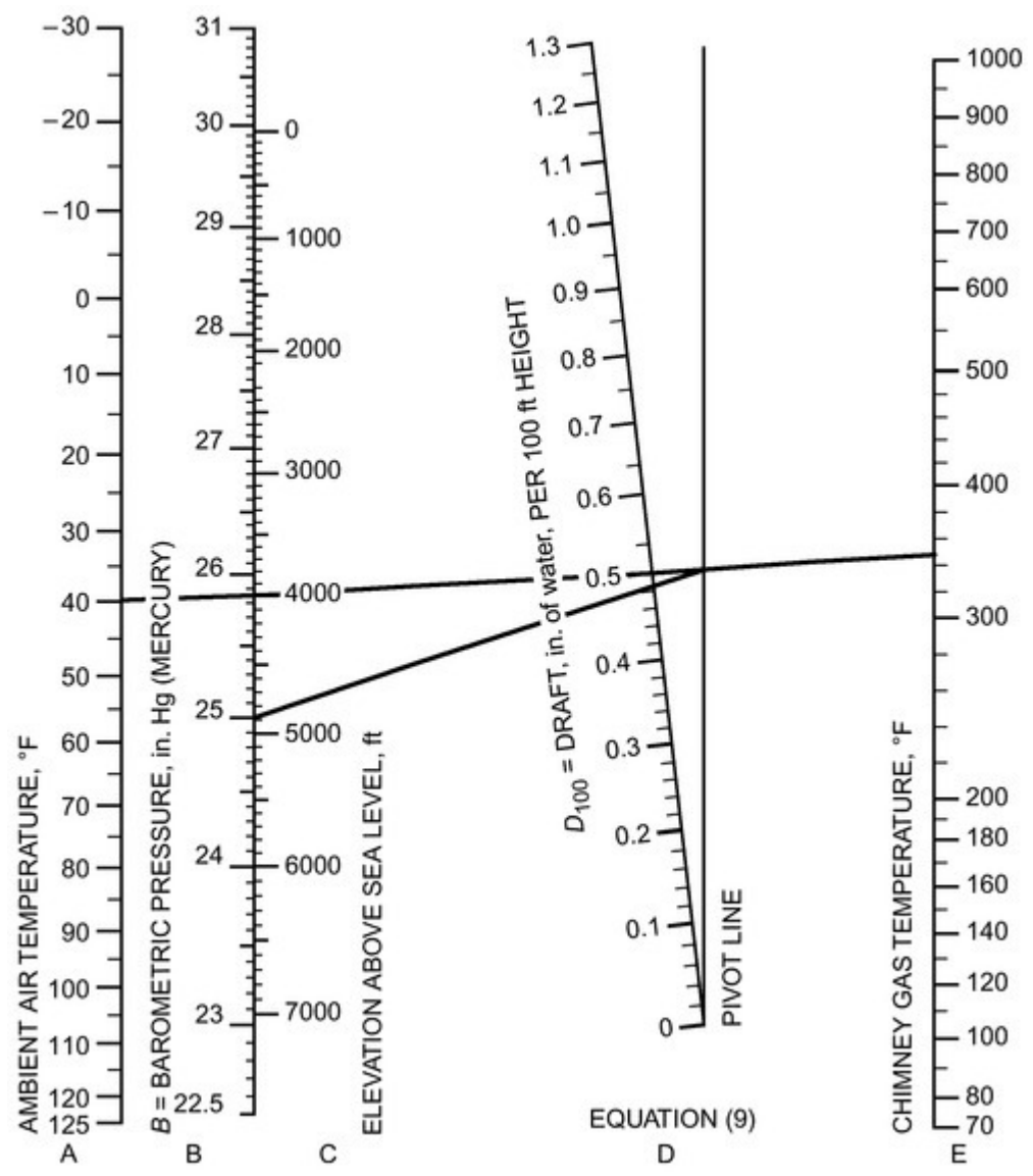
Figure 4. Theoretical Draft Nomograph
