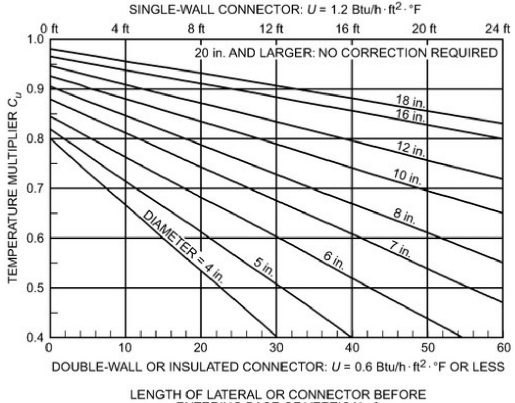
Figure 3. Temperature Multiplier C t for Compensation of Heat Losses in Connector
