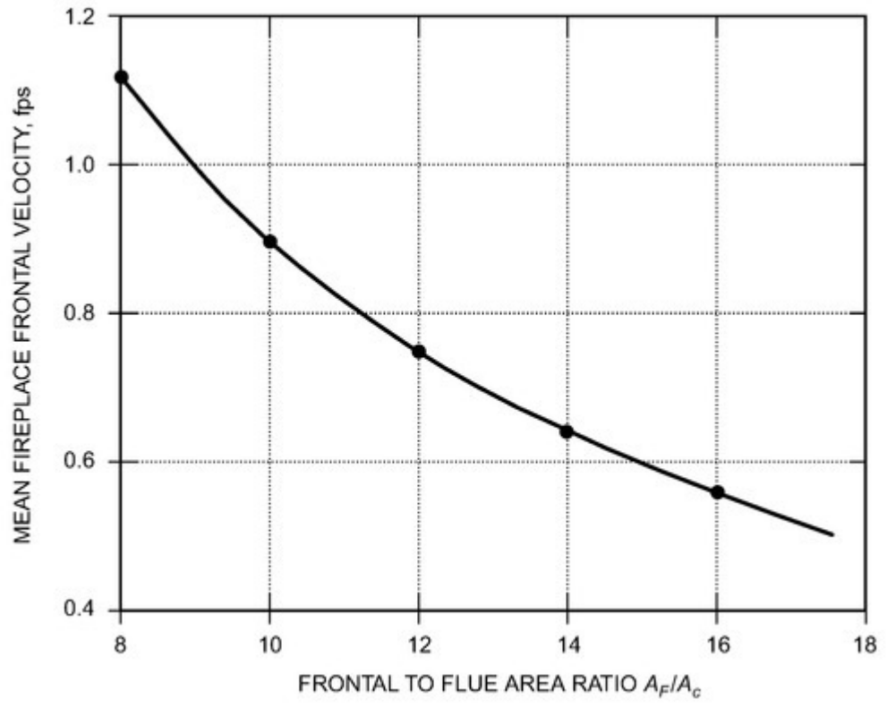
Figure 21. Effect of Area Ratio on Frontal Velocity (for chimney height of 15 ft with 12 in. inside diameter round flue)
