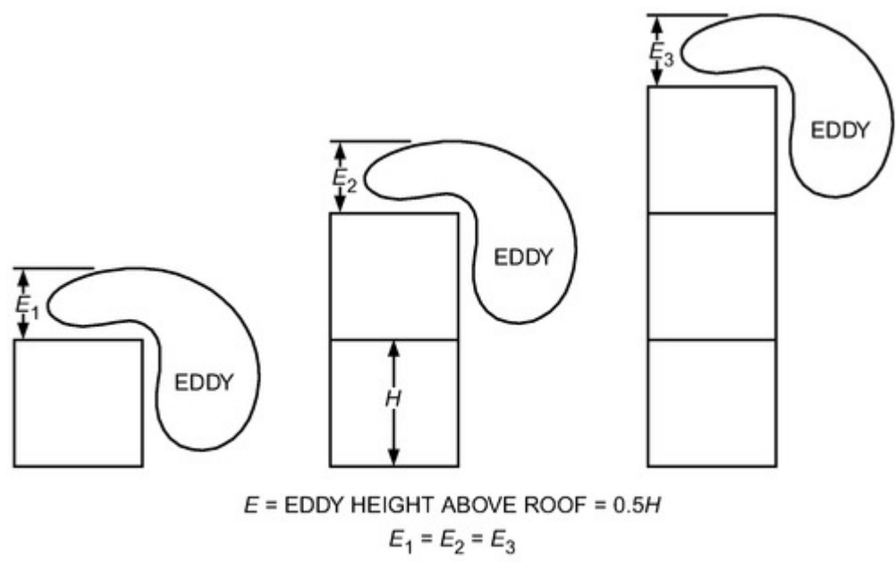
Figure 29. Height of Eddy Currents Around Single High-Rise Buildings
