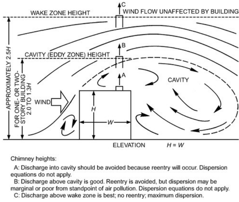
Figure 28. Wind Eddy and Wake Zones for One- or Two-Story Buildings and Their Effect on Chimney Gas Discharge (Clarke 1967)
