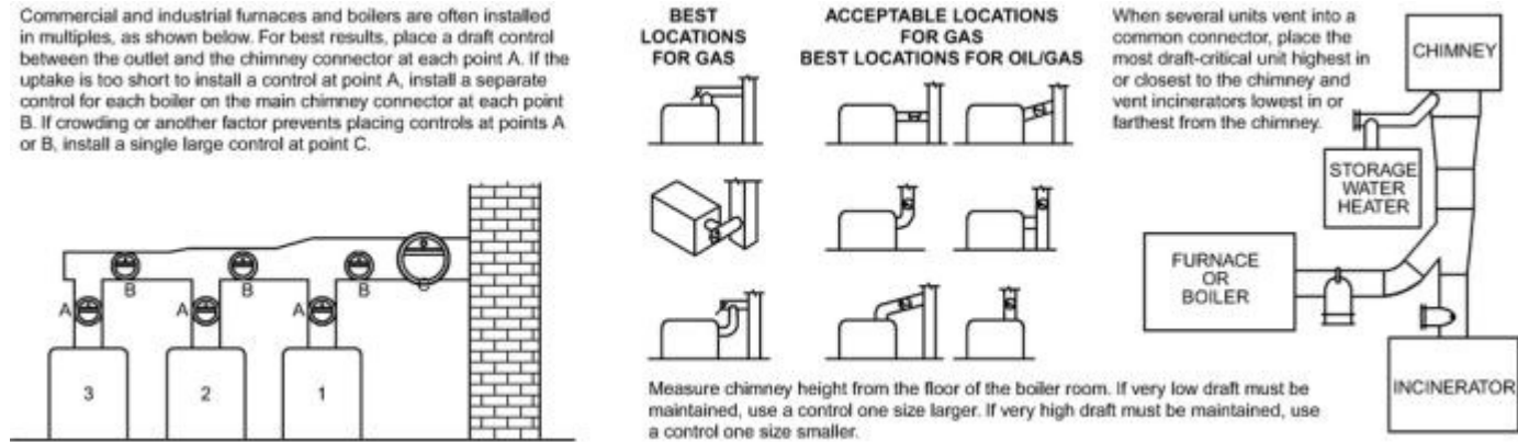
Figure 26. Use of Barometric Draft Regulators
