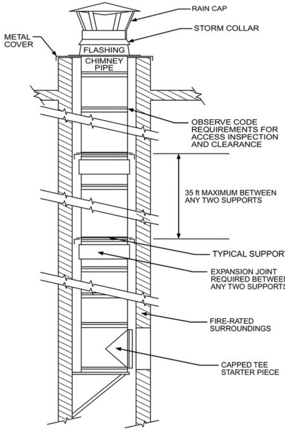
Figure 25. Building Heating Appliance, Medium-Heat Chimney
