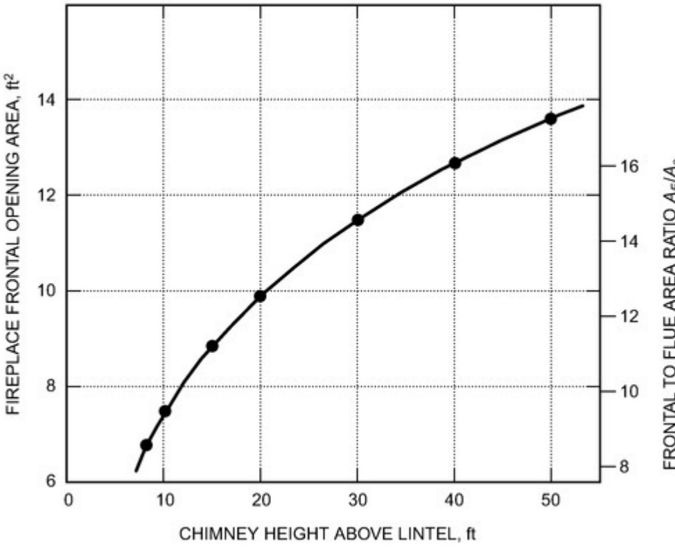
Figure 20. Permissible Fireplace Frontal Opening Area for Design Conditions (0.8 fps mean frontal velocity with 12 in. inside diameter round flue)
