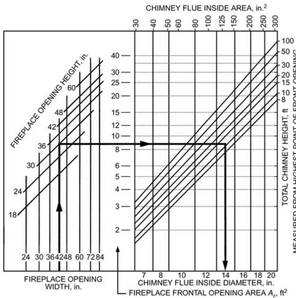
Figure 23. Chimney Sizing Chart for Fireplaces Mean face velocity = 0.8 fps (Stone 2005)
