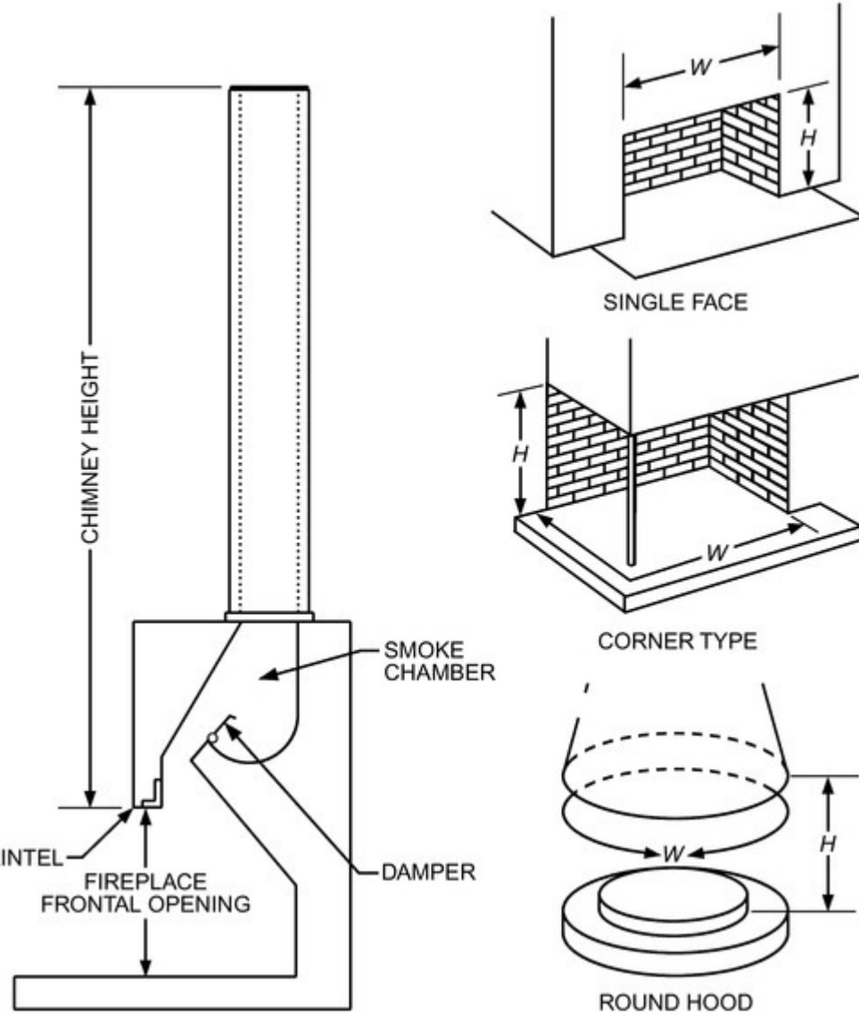
Figure 24. Estimation of Fireplace Frontal Opening Area
