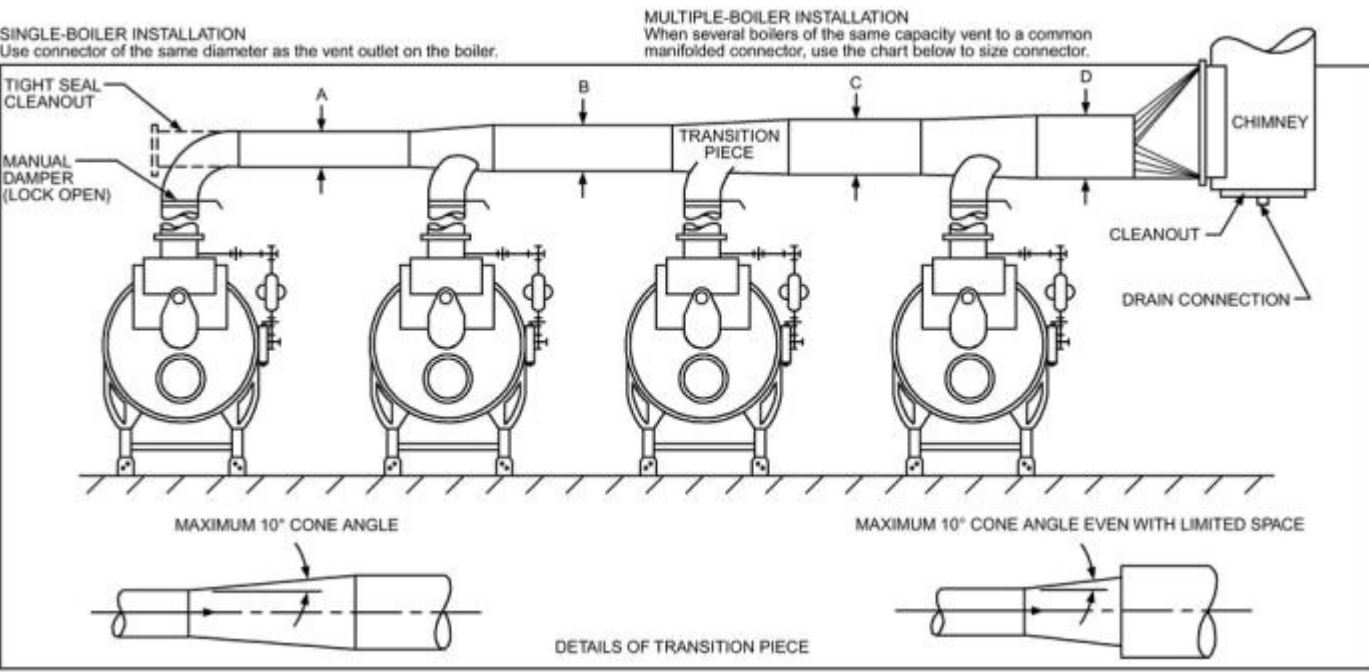
Figure 6. Typical Connector Design
