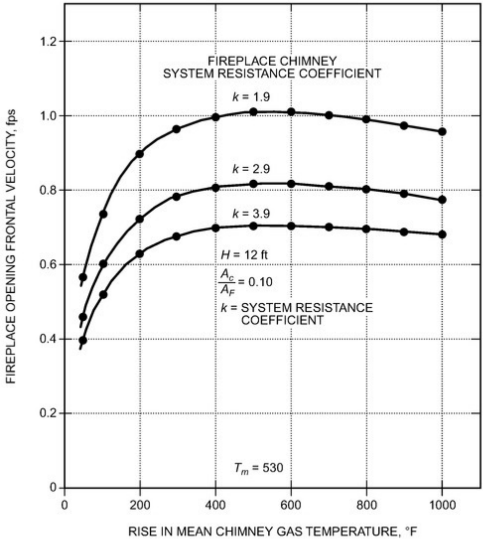
Figure 19. Effect of Chimney Gas (Combustion Products) Temperature on Fireplace Frontal Opening Velocity
