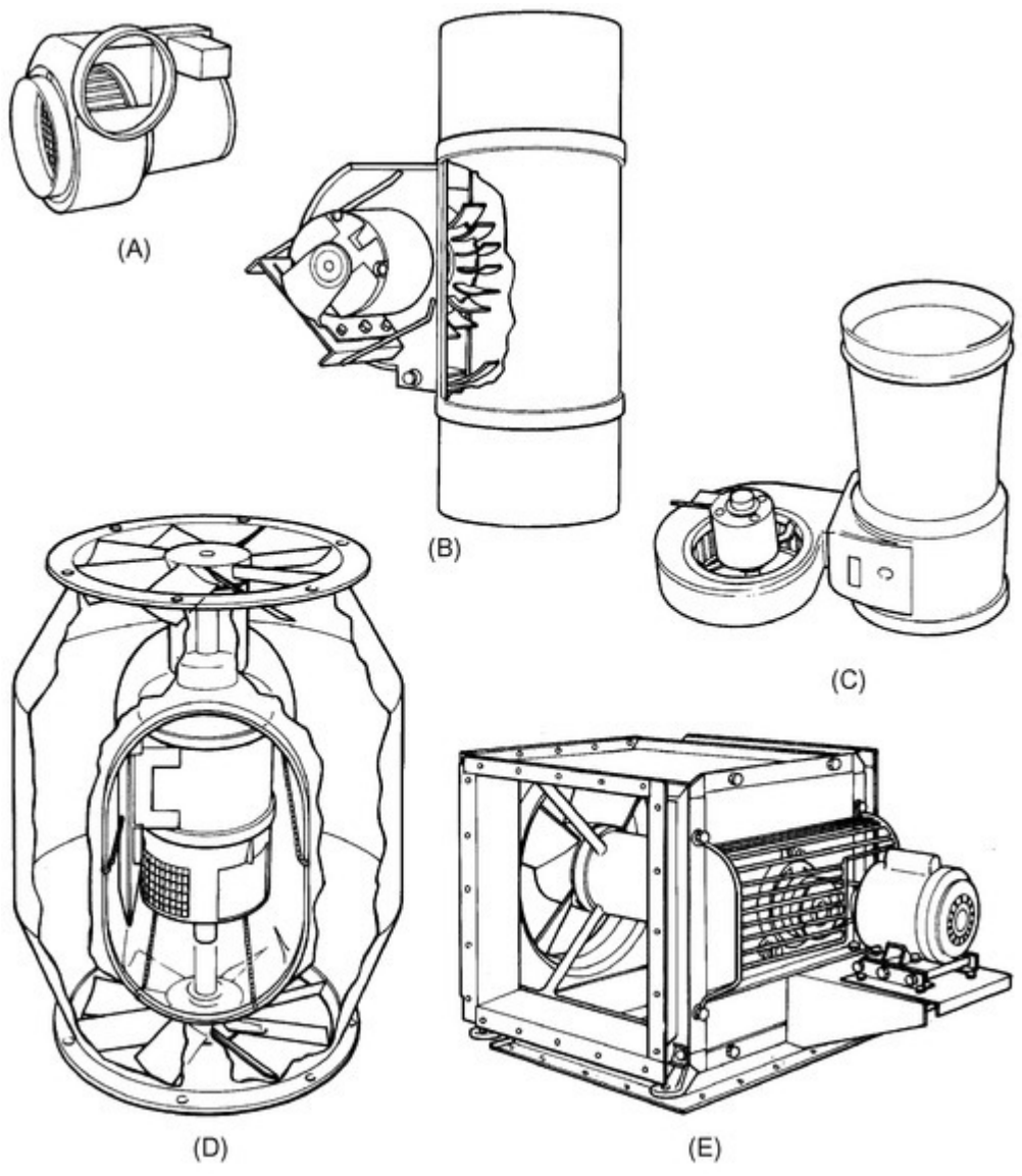
Figure 27. Draft Inducers
