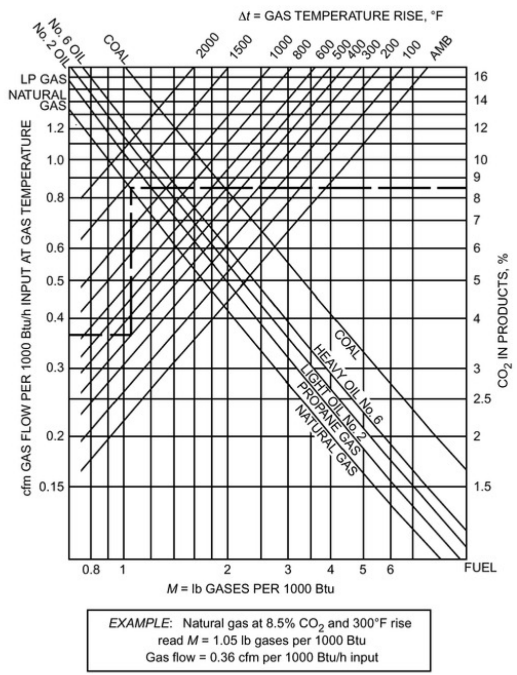
Figure 2. Flue Gas Mass and Volumetric Flow
