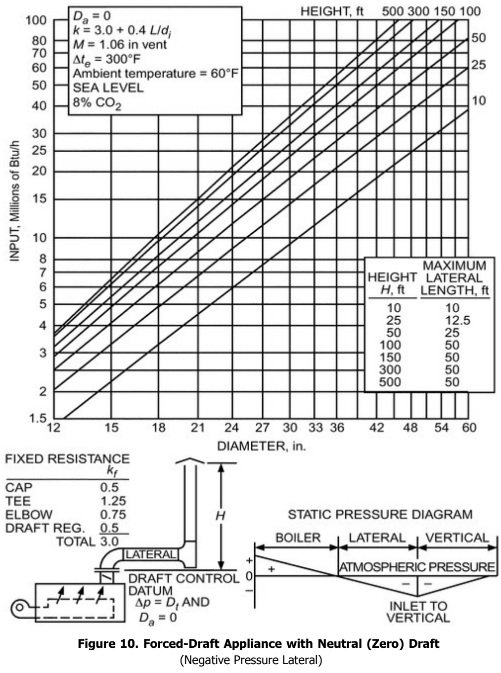
Figure 10. Forced-Draft Appliance with Neutral (Zero) Draft (Negative Pressure Lateral)
