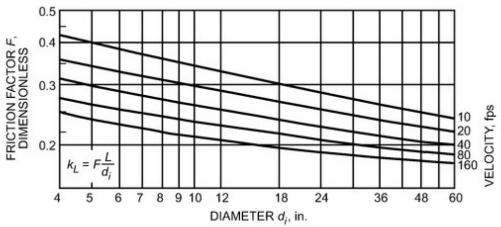
Figure 5. Friction Factor for Commercial Iron and Steel Pipe (Lapple 1949)
