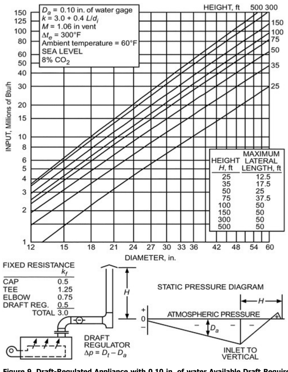
Figure 9. Draft-Regulated Appliance with 0.10 in. of water Available Draft Required
