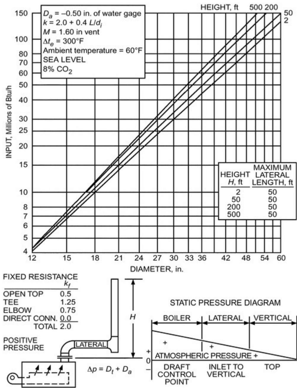
Figure 11. Forced-Draft Appliance with Positive Outlet Pressure (Negative Draft)
