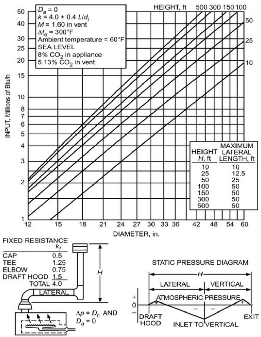
Figure 8. Gas Vent with Lateral
