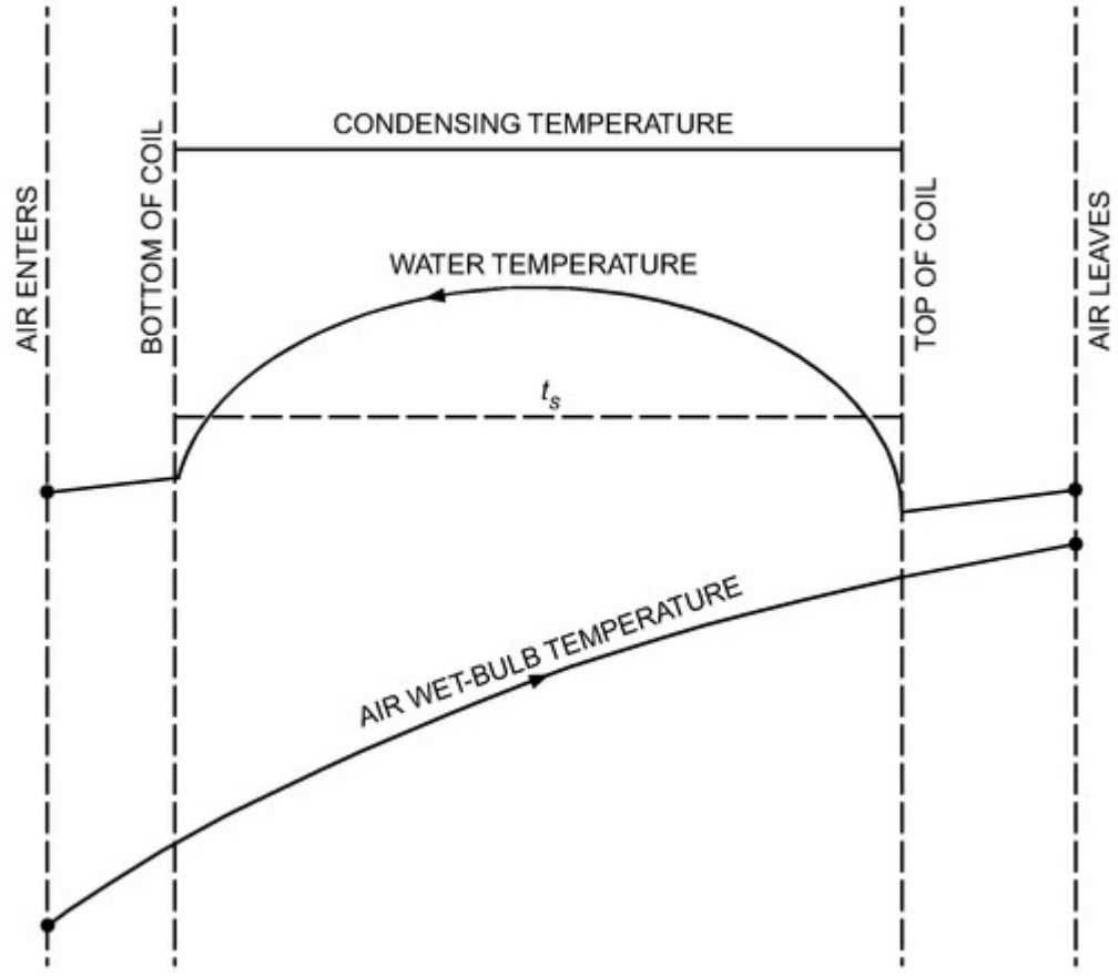
Figure 11. Heat Transfer Diagram for Evaporative Condenser
