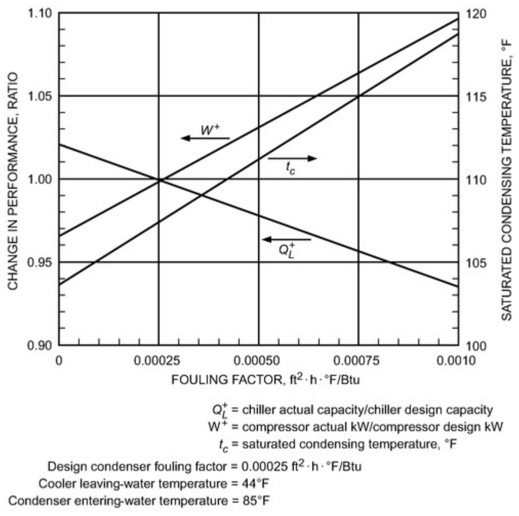
Figure 5. Effect of Fouling on Chiller Performance
