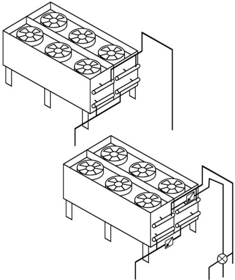
Figure 7. Equal-Sized Condenser Sections Connected in Parallel and for Half-Condenser Operation During Winter
