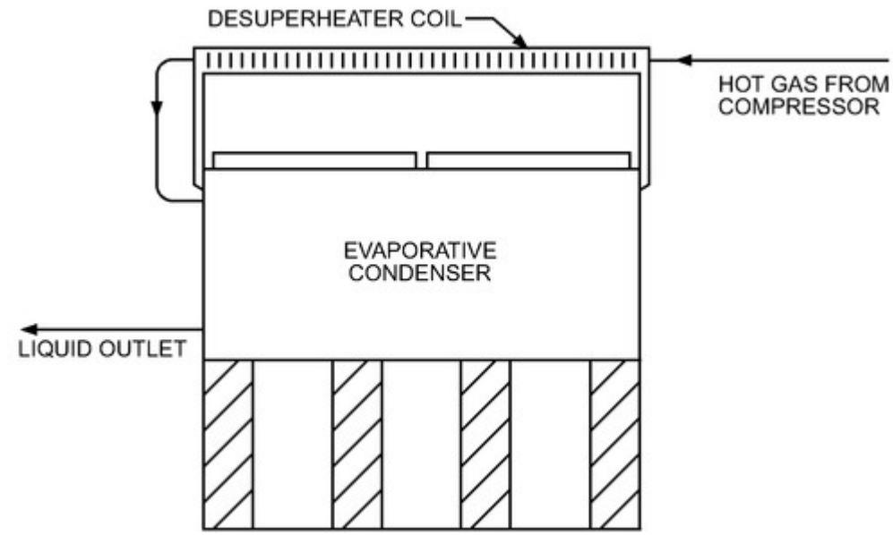
Figure 16. Evaporative Condenser with Desuperheater Coil
