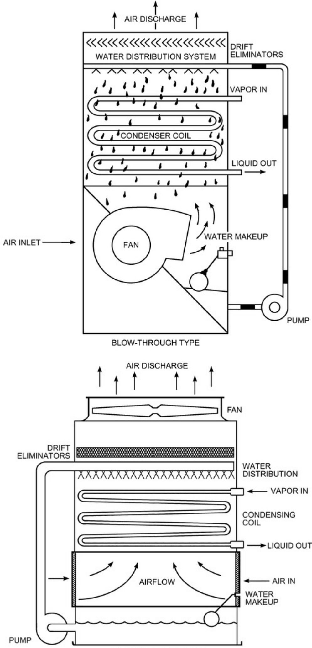
Figure 10. Functional Views of Evaporative Condenser
