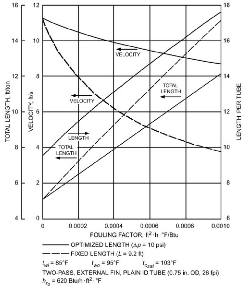
Figure 2. Effect of Fouling on Condenser
