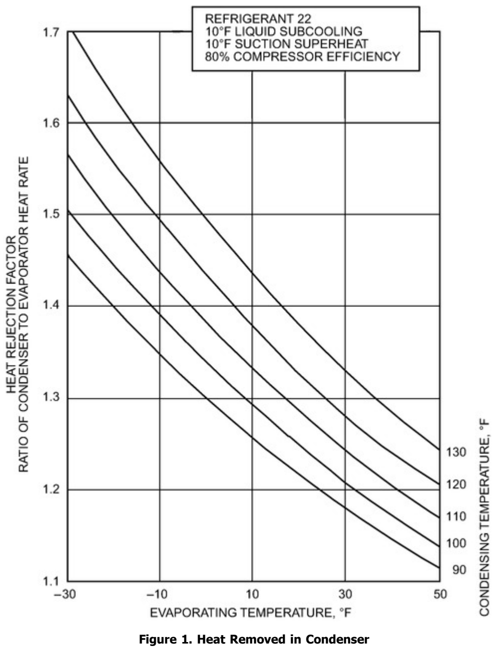
Figure 1. Heat Removed in Condenser
