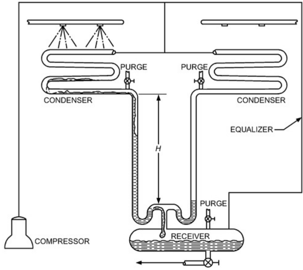
Figure 15. Parallel Operation of Two Evaporative Condensers
