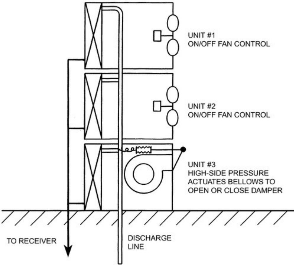
Figure 8. Unit Condensers Installed in Parallel with Combined Fan Cycling and Damper Control
