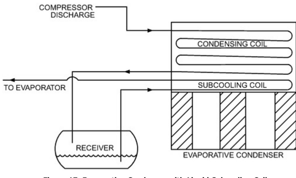
Figure 17. Evaporative Condenser with Liquid Subcooling Coil
