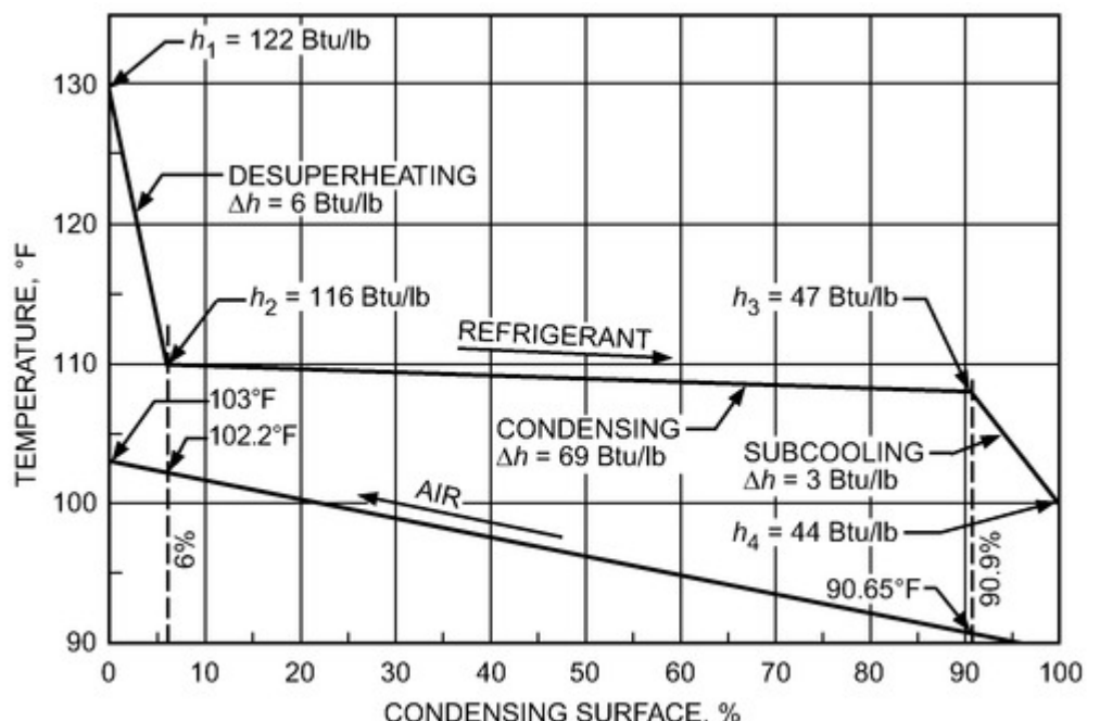
Figure 6. Temperature and Enthalpy Changes in Air-Cooled Condenser with R-134a
