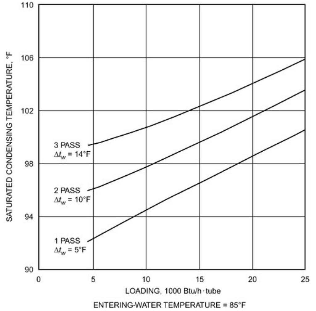
Figure 3. Effect of Condenser Water Circuiting
