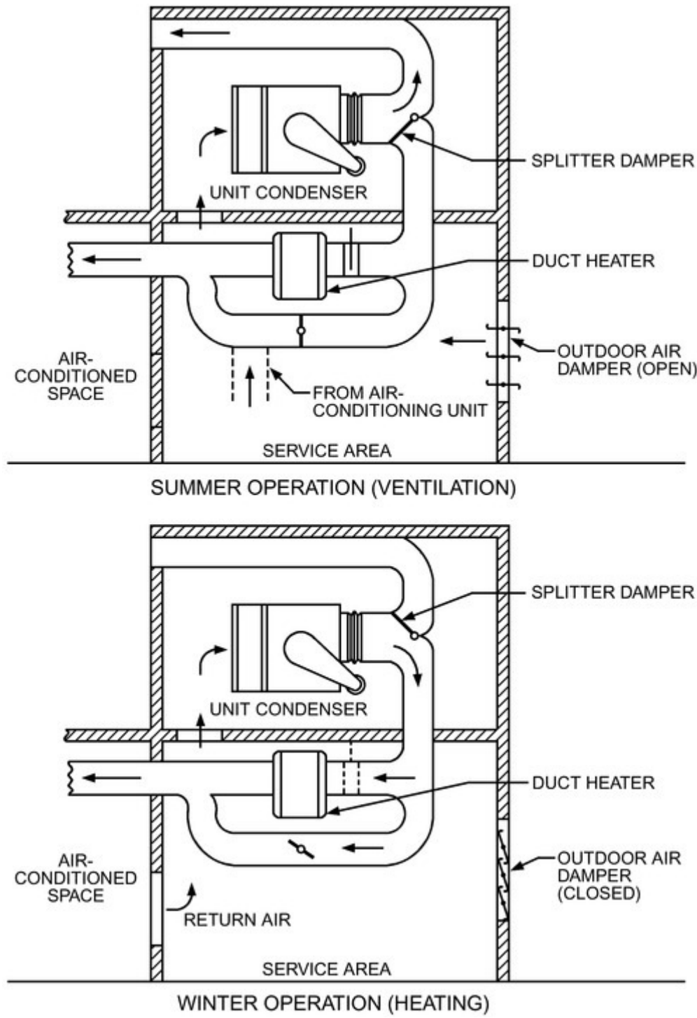
Figure 9. Air-Cooled Unit Condenser for Winter Heating and Summer Ventilation
