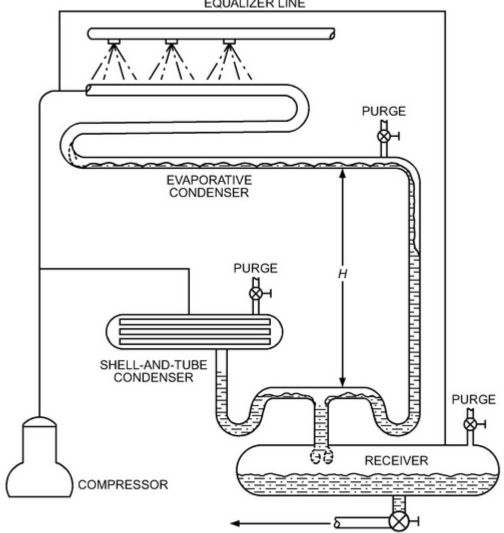
Figure 14. Parallel Operation of Evaporative and Shell-and-Tube Condenser
