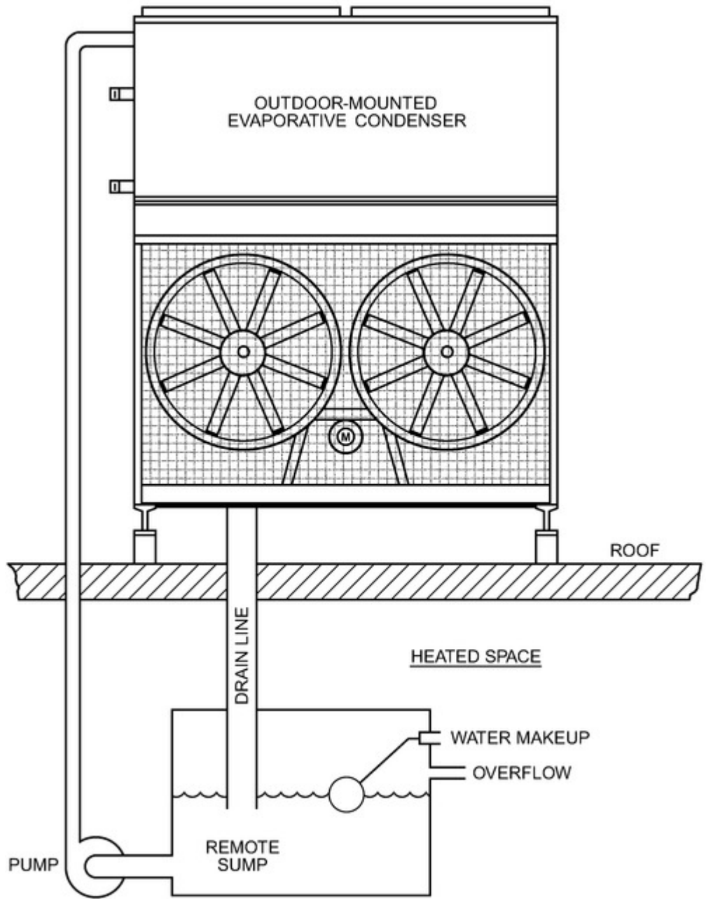
Figure 13. Evaporative Condenser Arranged for Year-Round Operation
