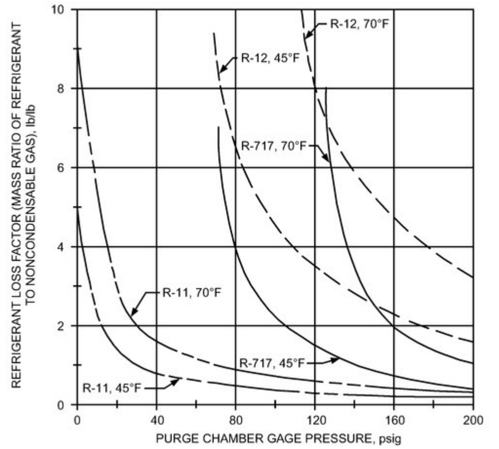
Figure 4. Loss of Refrigerant During Purging at Various Gas Temperatures and Pressures
