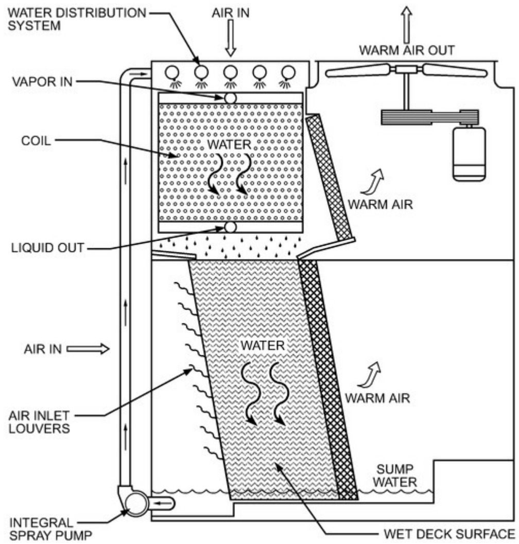
Figure 12. Combined Coil/Fill Evaporative Condenser
