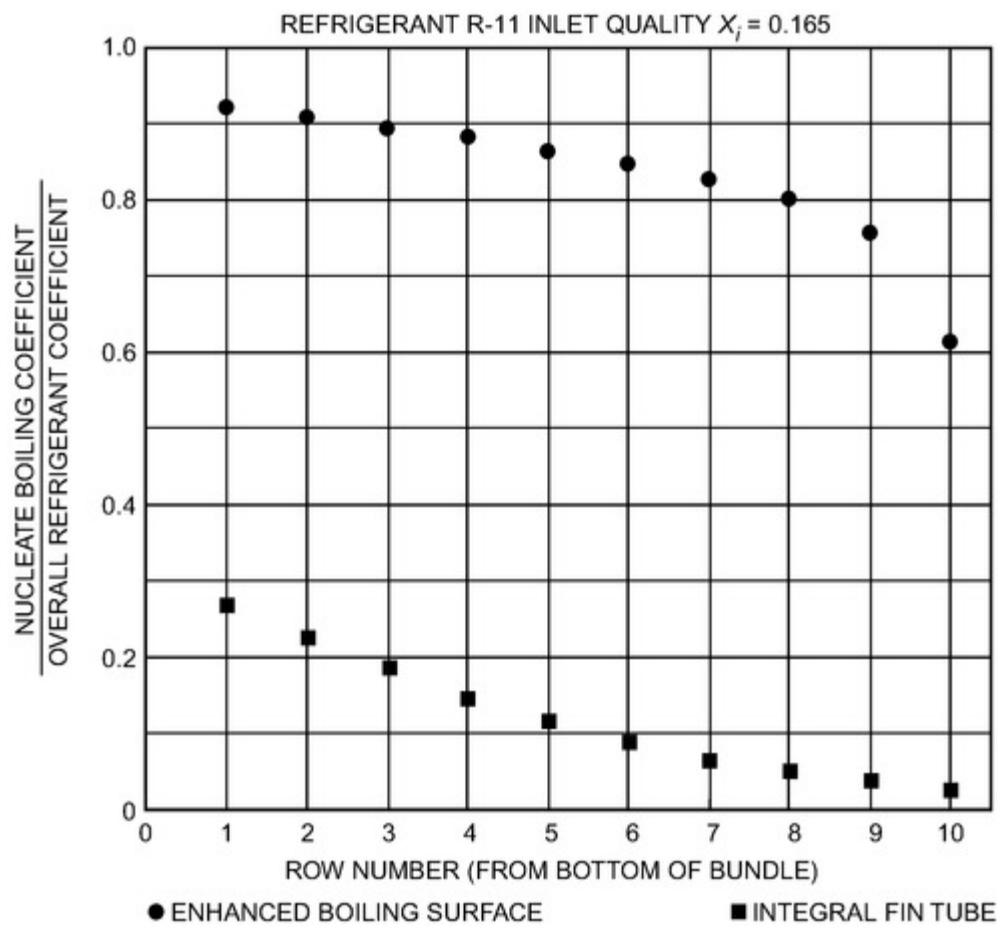
Figure 6. Nucleate Boiling Contribution to Total Refrigerant Heat Transfer
