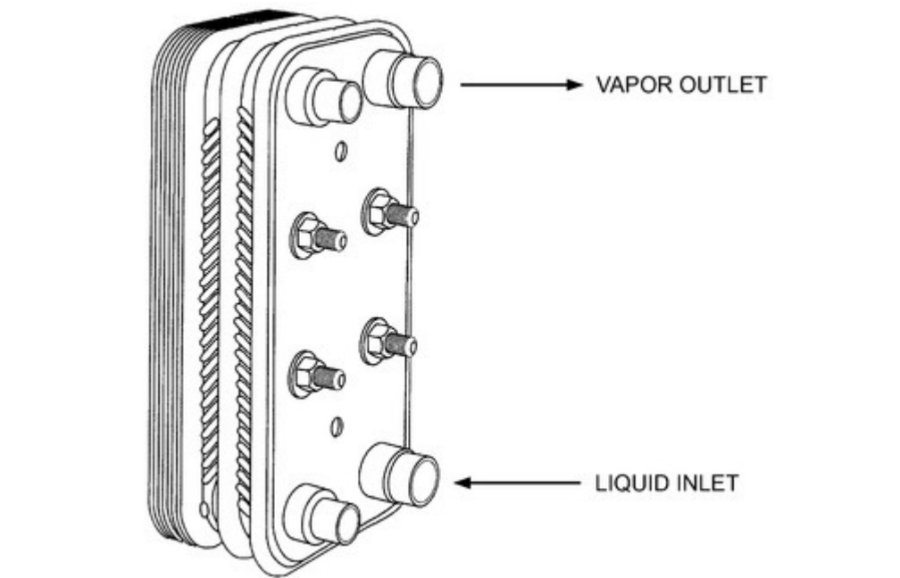
Figure 3. Flooded Plate Cooler
