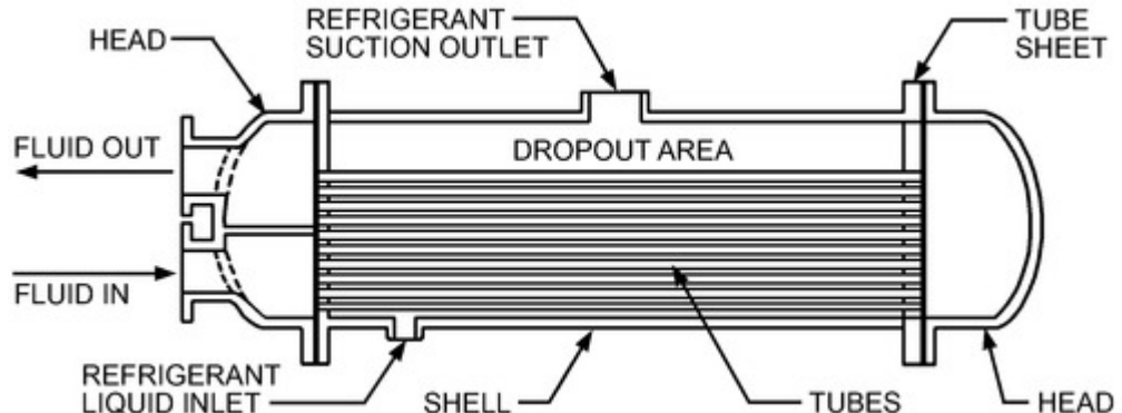
Figure 2. Flooded Shell-and-Tube Cooler
