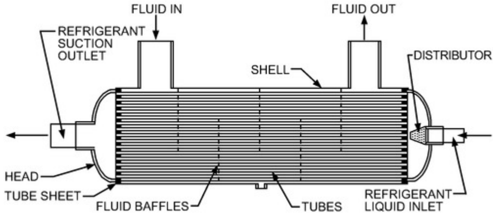
Figure 1. Direct-Expansion Shell-and-Tube Cooler
