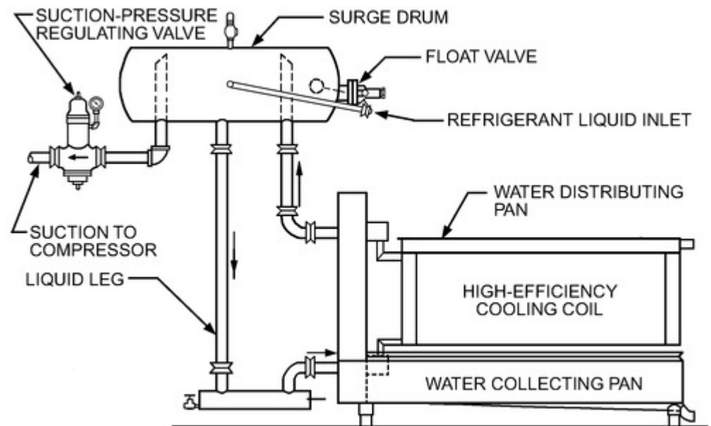
Figure 4. Baudelot Cooler
