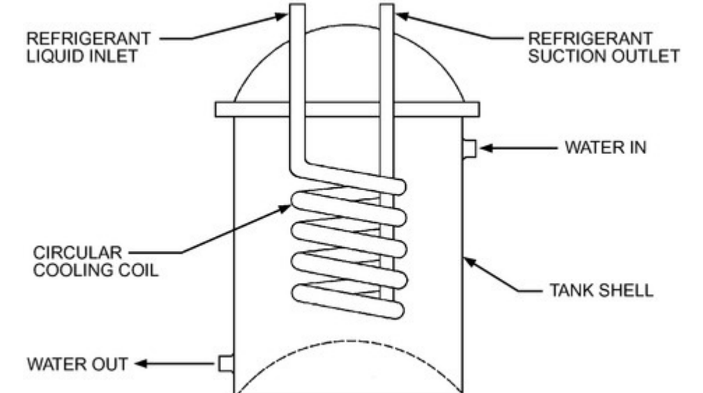
Figure 5. Shell-and-Coil Cooler
