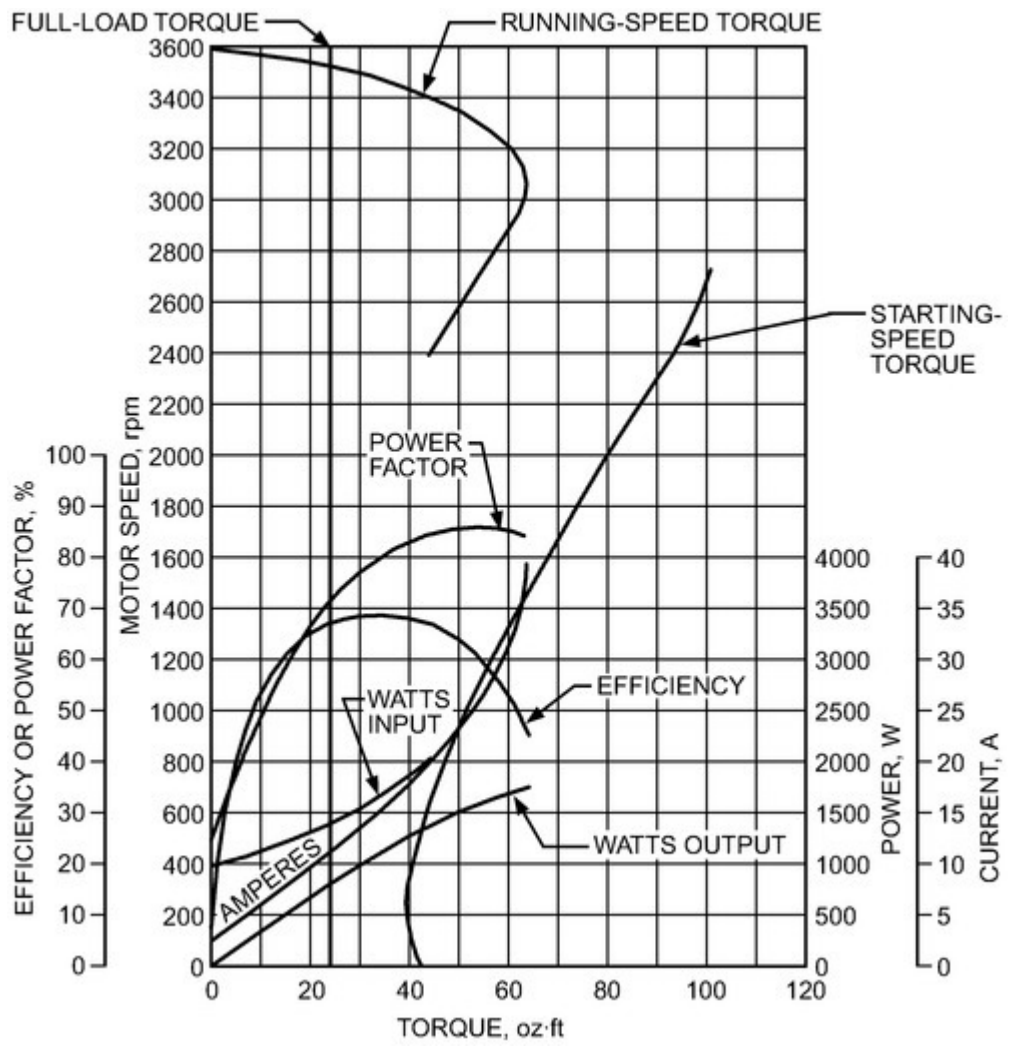
Figure 1. Typical Performance Characteristics of Capacitor-Start/Induction-Run Two-Pole General-Purpose Motor, 1 hp
