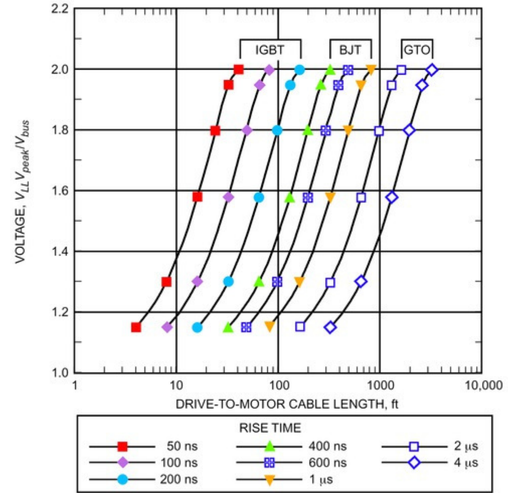
Figure 23. Typical Switching Times, Cable Distance, and Pulse Peak Voltage
