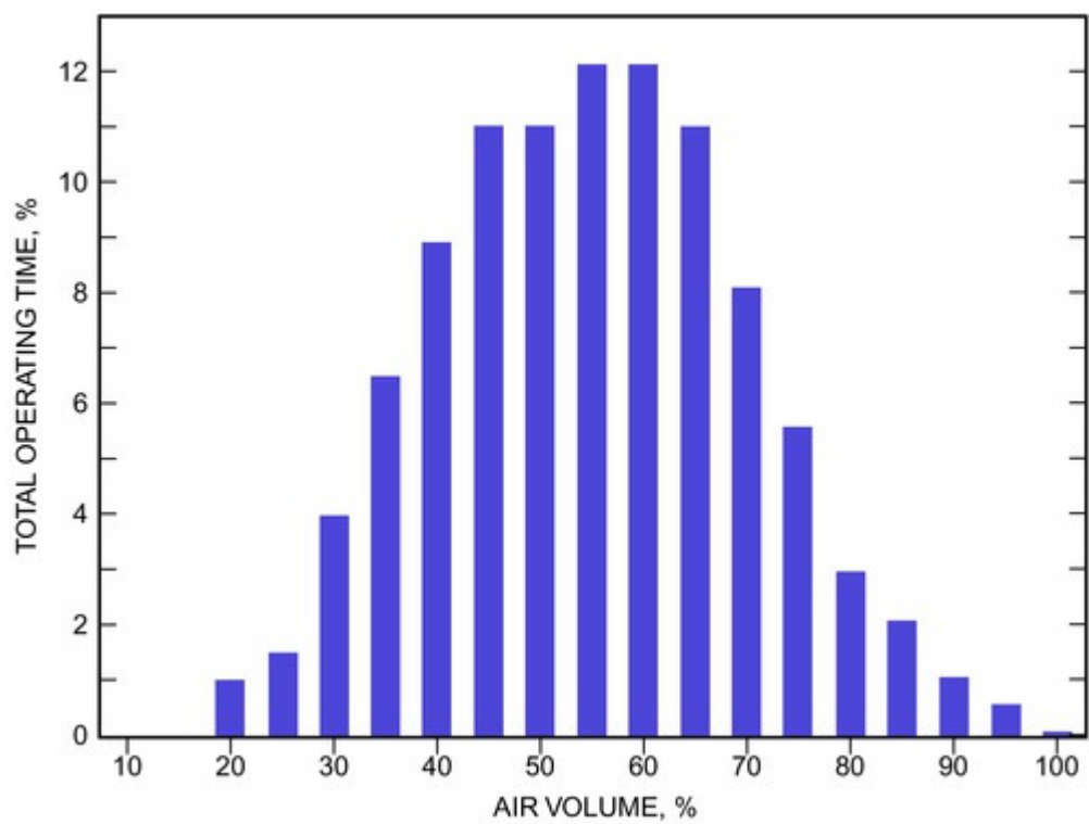
Figure 16. Typical Fan Duty Cycle for VAV System
