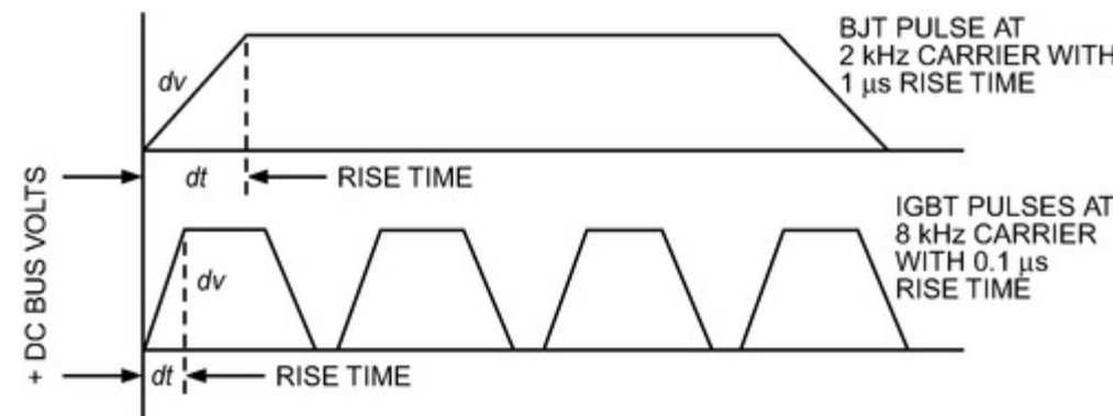
Figure 21. Bipolar Versus IGBT PWM Switching
