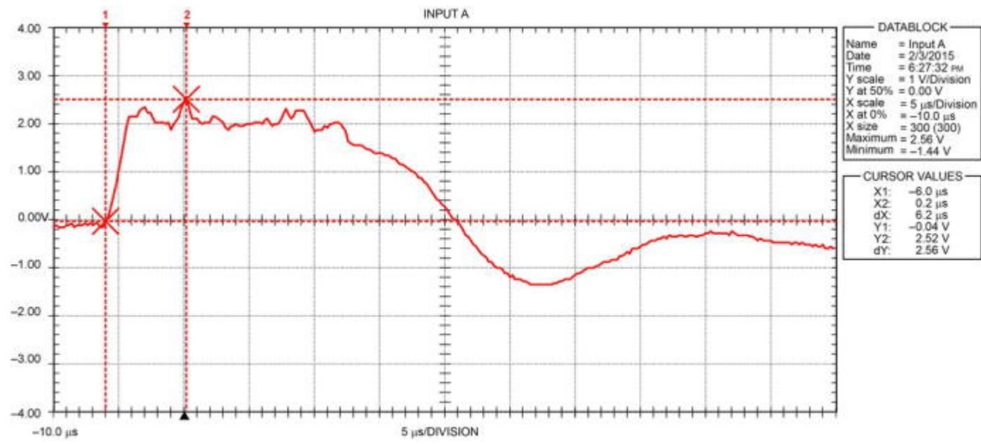
Figure 9. 2.5 V Peak Shaft Voltage, No Discharge
