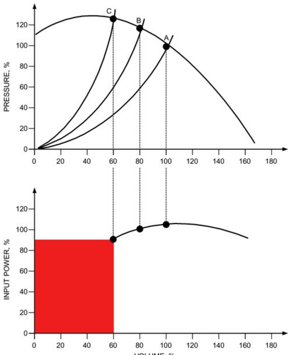
Figure 17. Outlet Damper Control
