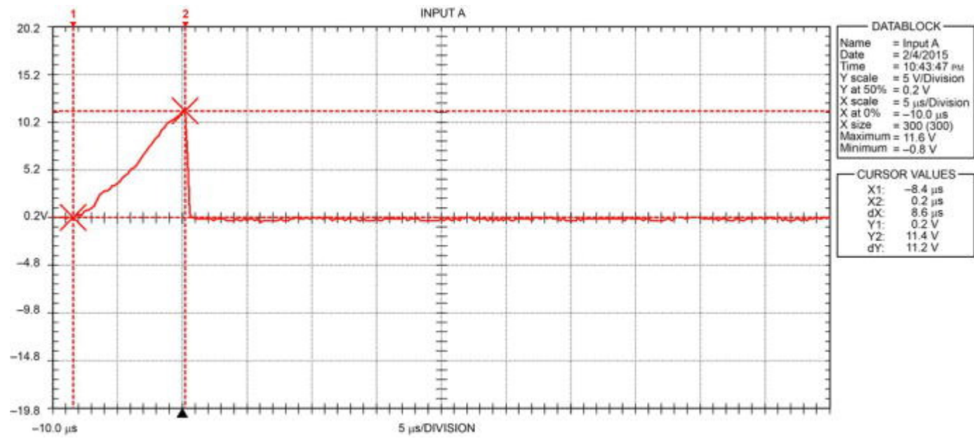
Figure 11. 11.4 V Peak Shaft Voltage, Discharge Detected
