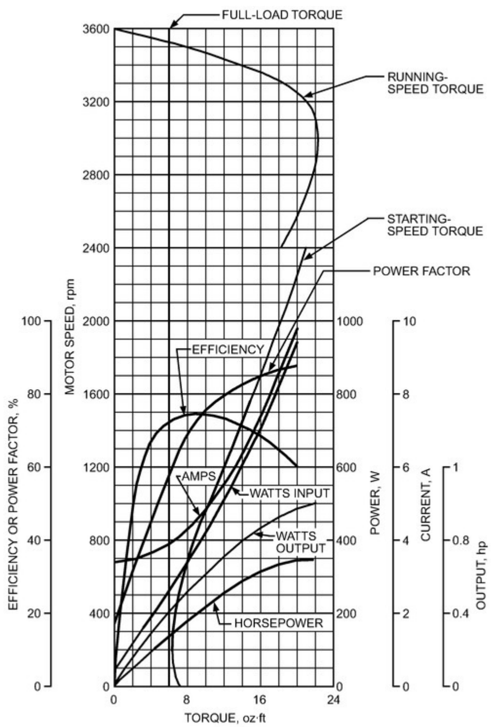
Figure 2. Typical Performance Characteristics of Resistance-Start Split-Phase Two-Pole Hermetic Motor, 0.25 hp
