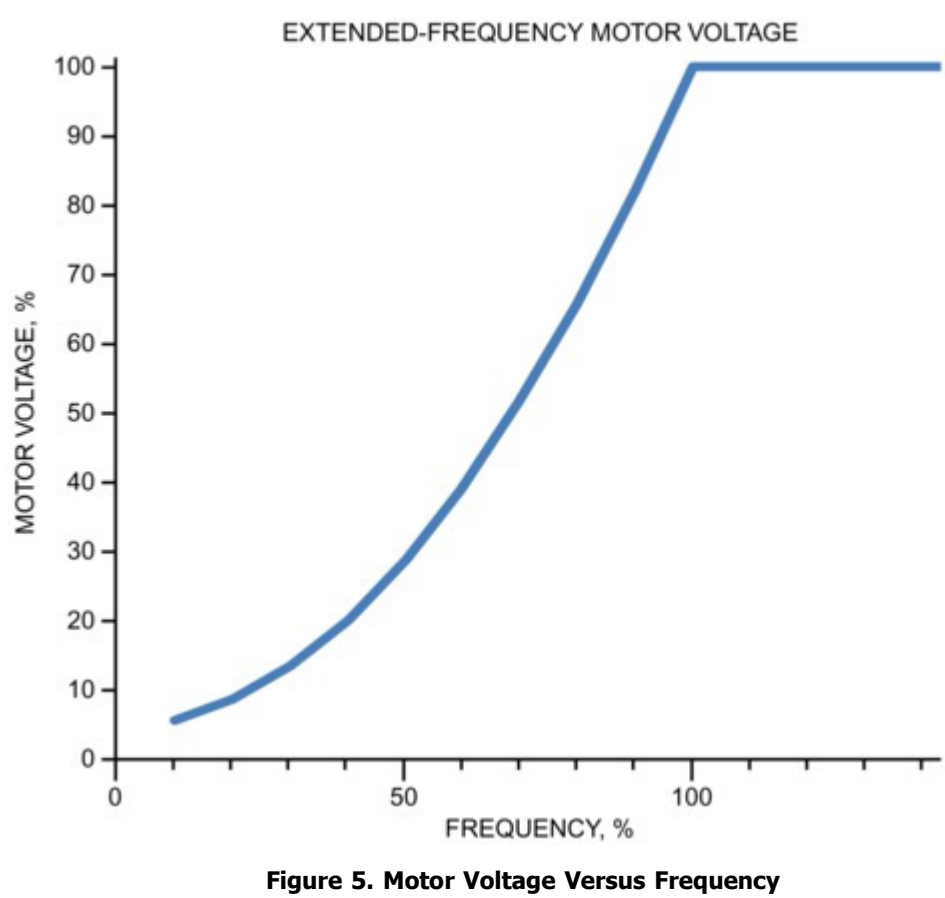
Figure 5. Motor Voltage Versus Frequency
