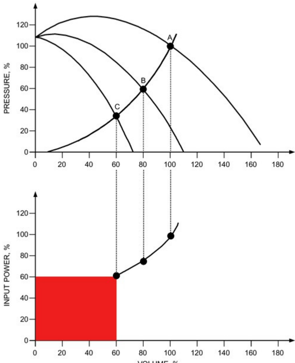
Figure 18. Variable Inlet Vane Control
