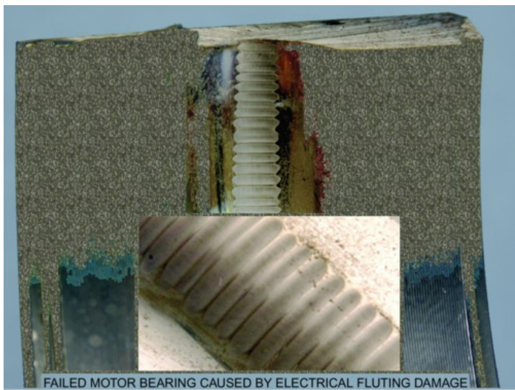
Figure 8. Fluted Bearing from VFD-Induced Electrical Bearing Current Discharges (Oh and Willwerth 2008)
