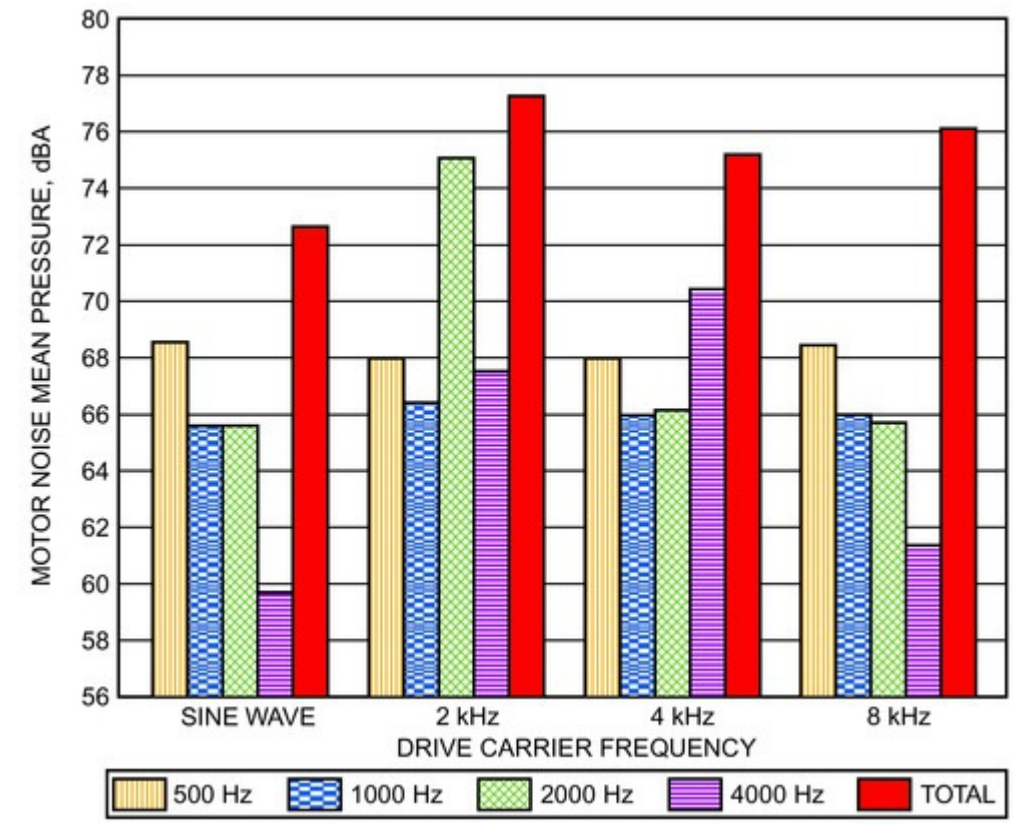
Figure 27. Motor Audible Noise
