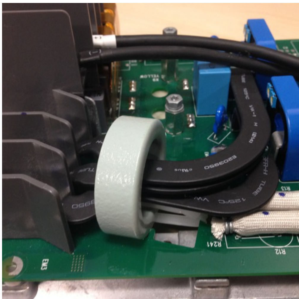
Figure 13. Common Mode Toroid Built into Output of VFD
