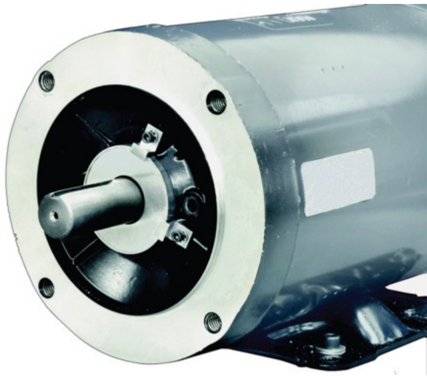
Figure 15. Shaft Grounding Ring Installed on Motor (Oh and Willwerth 2008)
