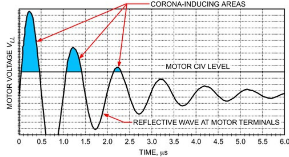
Figure 26. Damaging Reflected Waves above Motor CIV Levels
