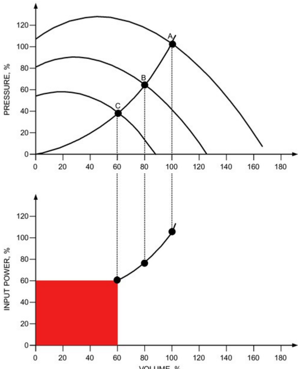
Figure 19. Eddy Current Coupling Control
