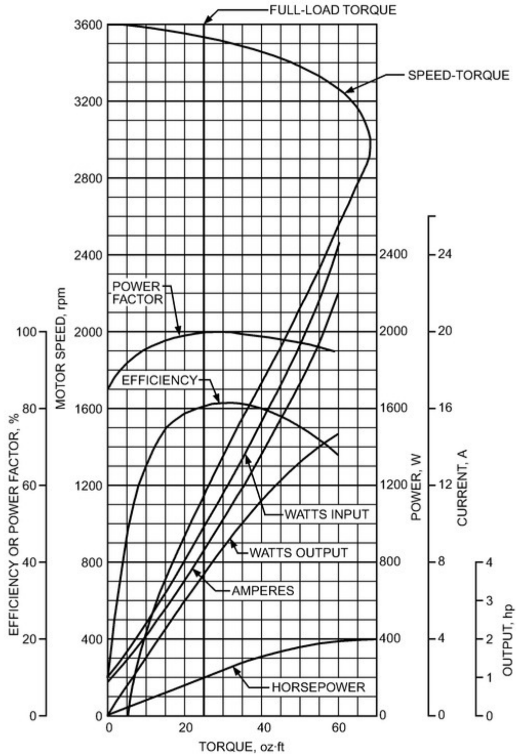
Figure 3. Typical Performance Characteristics of Permanent Split-Capacitor Two-Pole Motor, 1 hp
