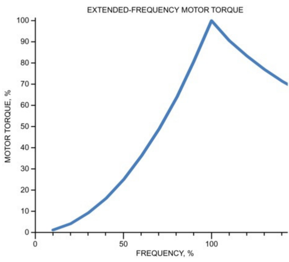
Figure 6. Motor Torque Limits Versus Frequency
