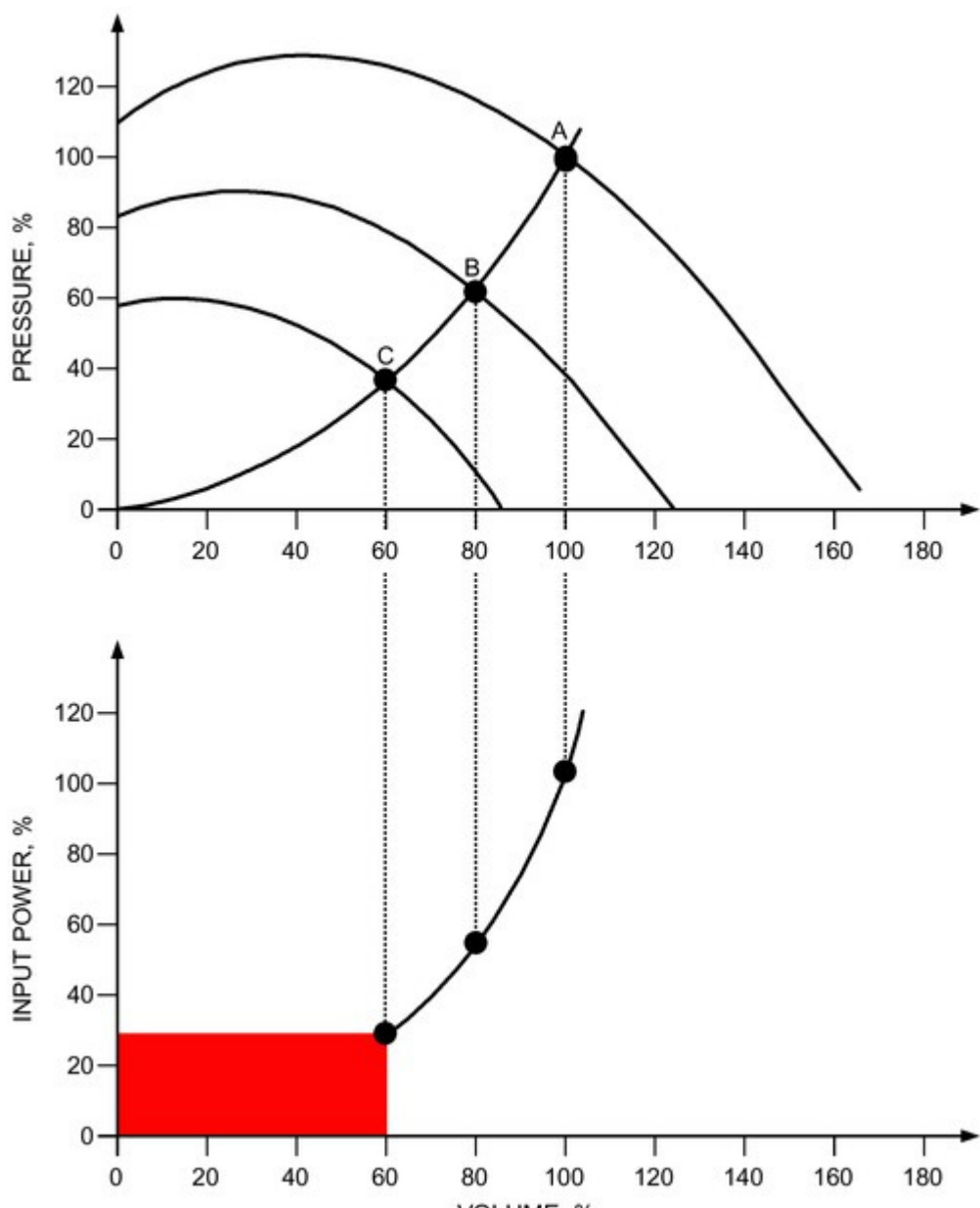
Figure 20. AC Drive Control
