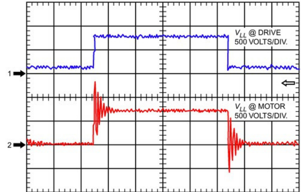
Figure 24. Typical Reflected Wave Voltage Levels at Drive and Motor Insulation
