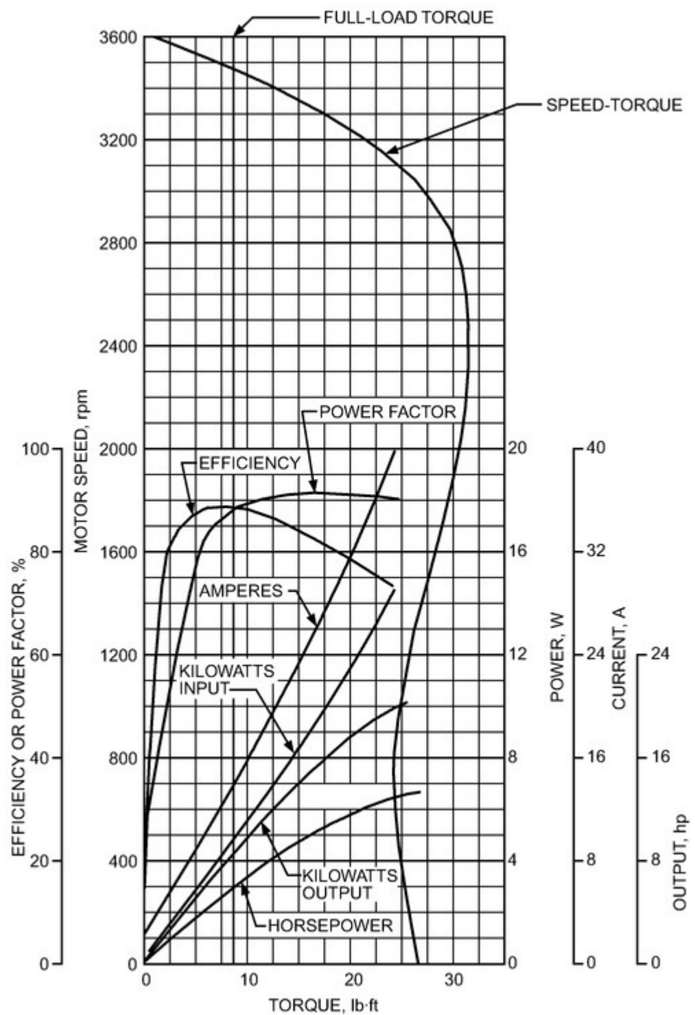
Figure 4. Typical Performance Characteristics of Three-Phase Two-Pole Motor, 5 hp
