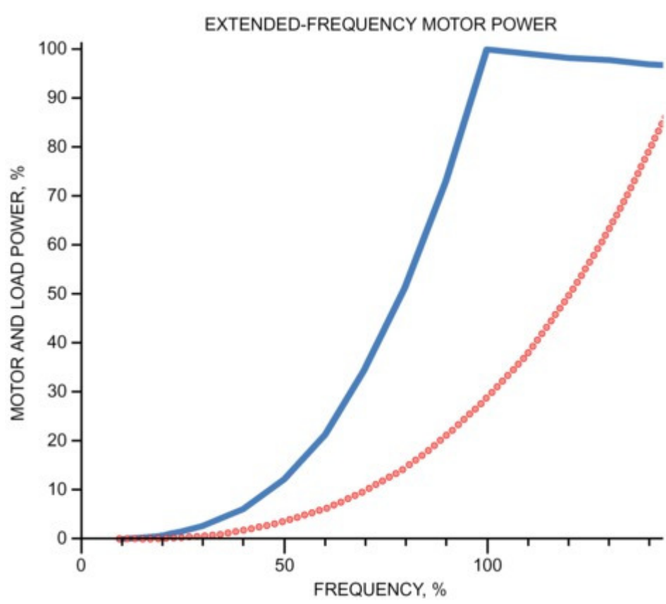
Figure 7. Motor Power Capacity at Maximum Extended Frequency
