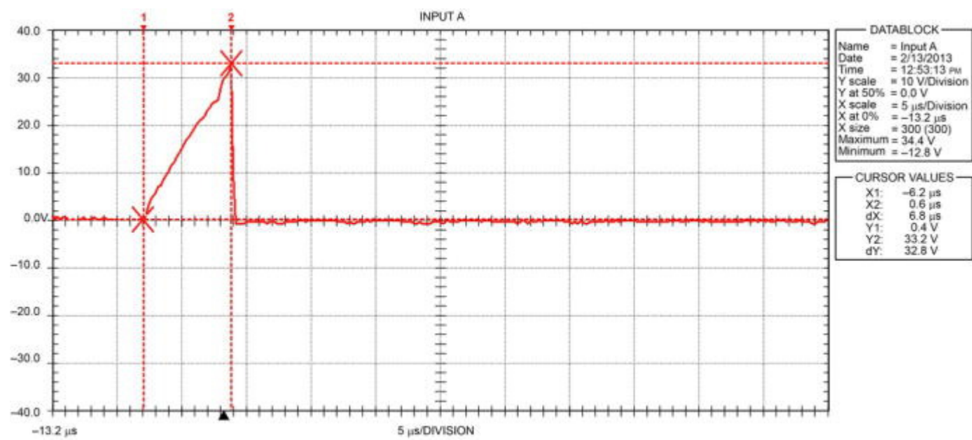
Figure 12. 32.2 V Peak Shaft Voltage, Discharge Detected
