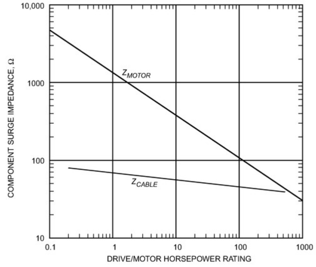
Figure 22. Motor and Drive Relative Impedance
