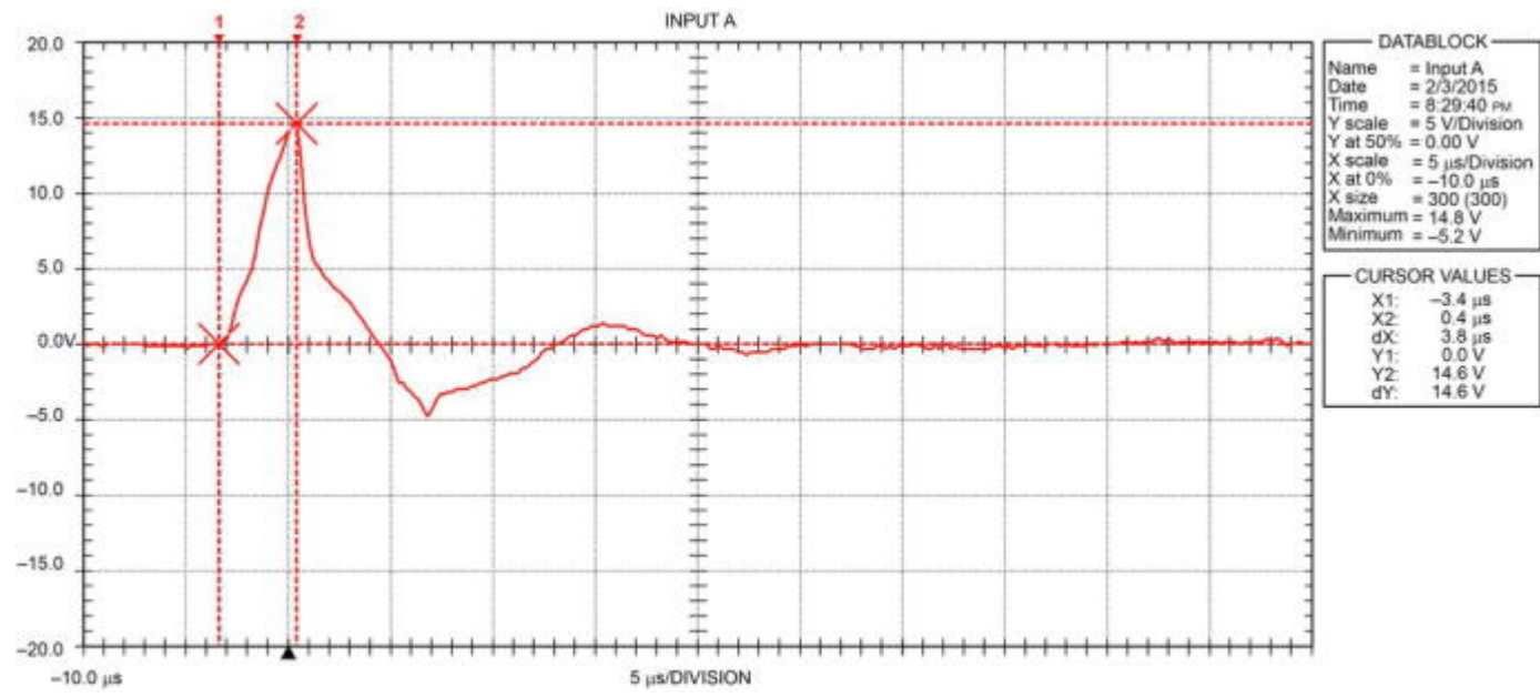
Figure 10. 14.6 V Peak Shaft Voltage, No Discharge
