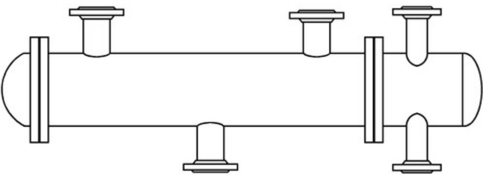
Figure 6. Straight-Tube Fixed Tubesheet Shell-and-Tube Heat Exchanger with Fabricated Bonnet Heads and Split-Shell Flow Design
