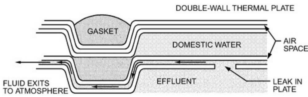
Figure 12. Double-Wall Plate Cassette for Gasketed Plate and Frame Exchanger
