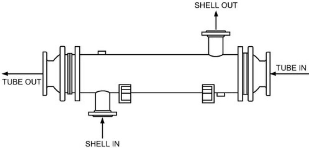
Figure 2. Counterflow Path in Shell-and-Tube Heat Exchanger
