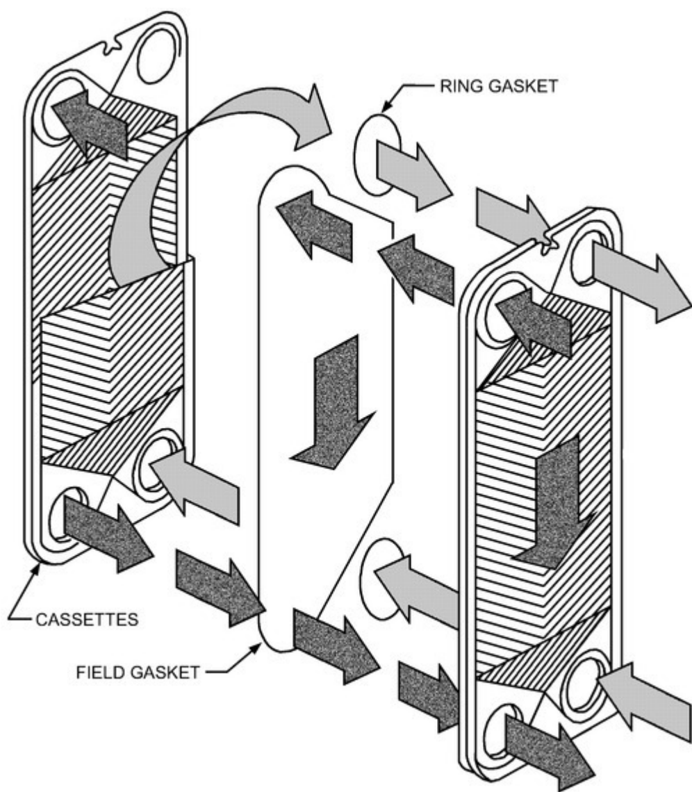
Figure 8. Flow Path of Gasketed-Plate Heat Exchanger
