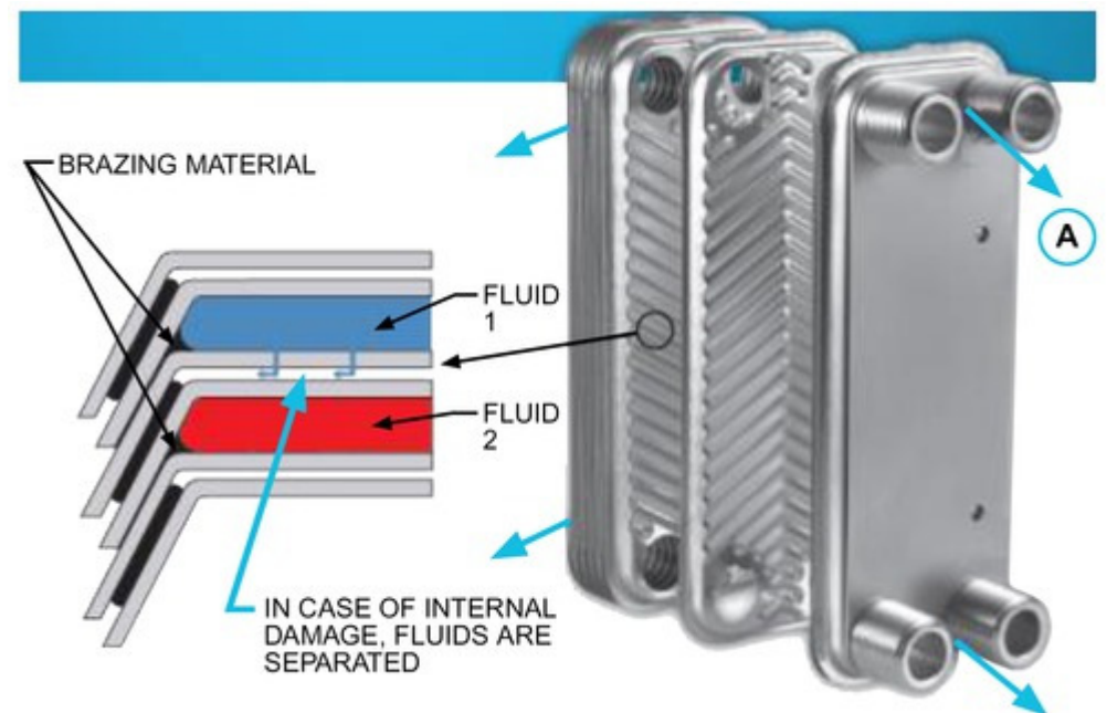
Figure 13. Double-Wall Plate Assembly with Brazed-Plate Exchanger (Courtesy Bell & Gossett)
