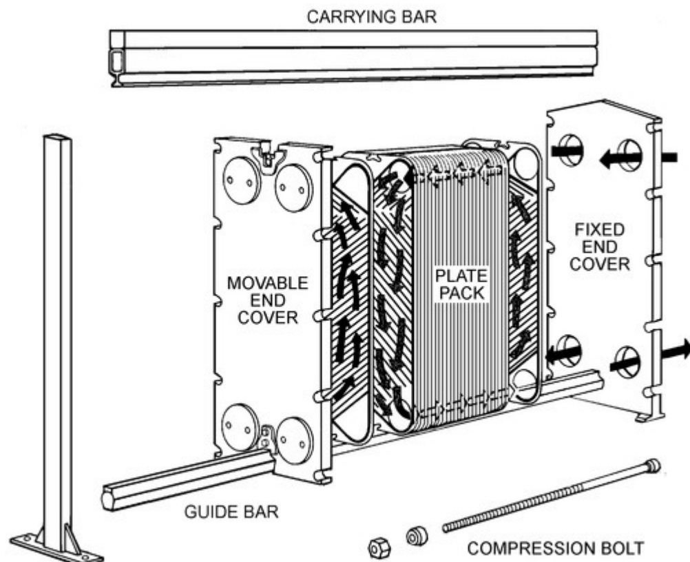
Figure 15. Components of a Gasketed Plate Heat Exchanger
