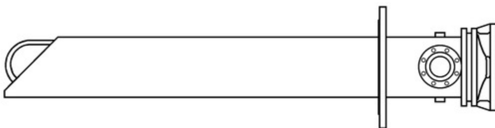
Figure 5. U-Tube Tank Suction Heater with Removable Bundle Assembly and Cast Flanged Head
