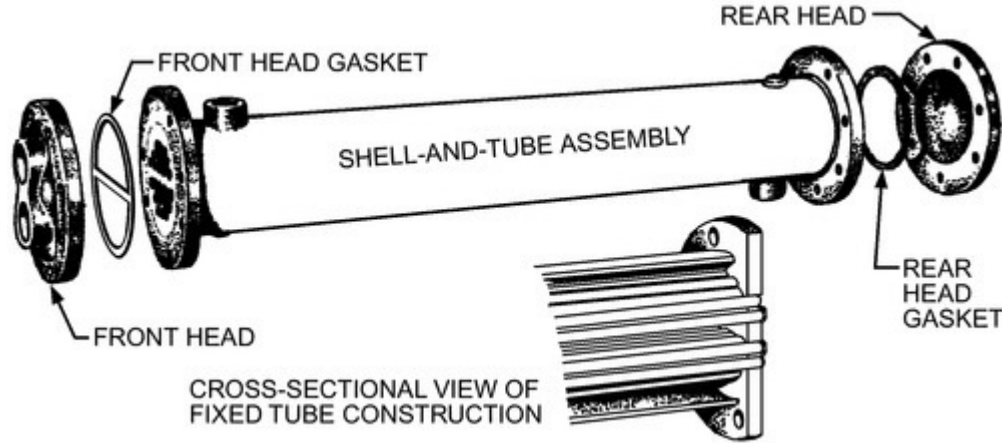
Figure 14. Exploded View of Straight-Tube Heat Exchanger
