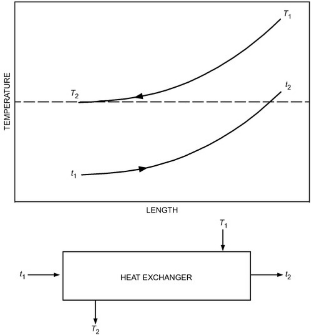
Figure 1. Temperature Distribution in Counterflow Heat Exchanger
