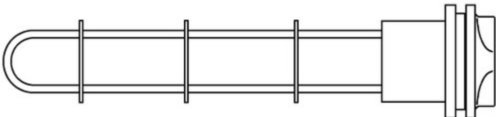
Figure 4. U-Tube Tank Heater with Removable Bundle Assembly and Cast Bonnet Head
