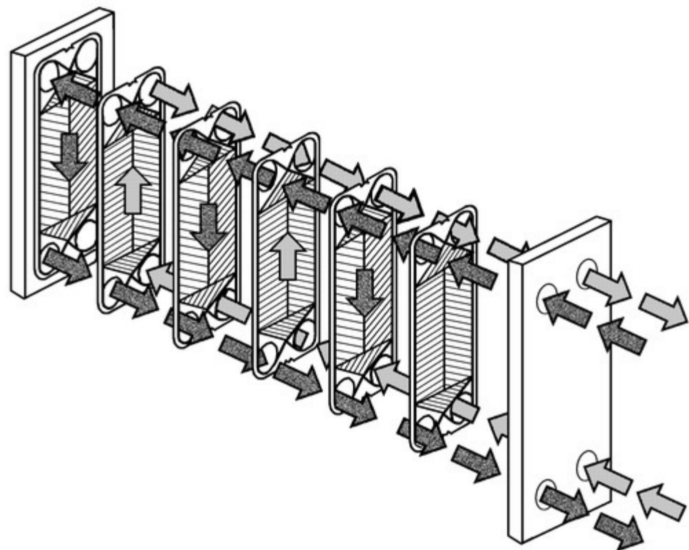
Figure 9. Flow Path of Welded-Plate Heat Exchanger
