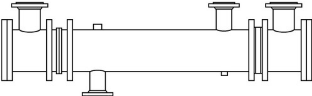
Figure 7. Straight-Tube Floating Tubesheet Shell-and-Tube Heat Exchanger with Removable Bundle Assembly and Fabricated Channel Heads
