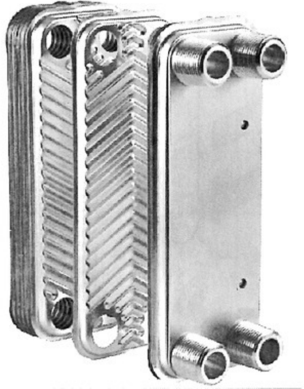
Figure 10. Brazed-Plate Heat Exchanger
