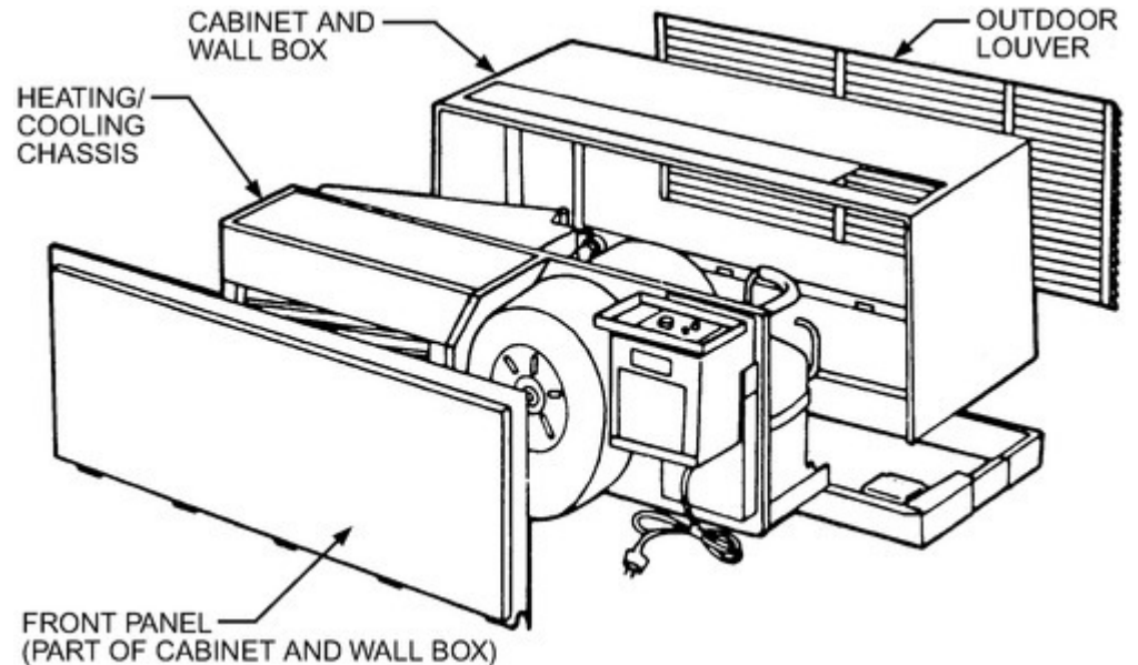
Figure 3. Integrated Packaged Terminal Air Conditioner
