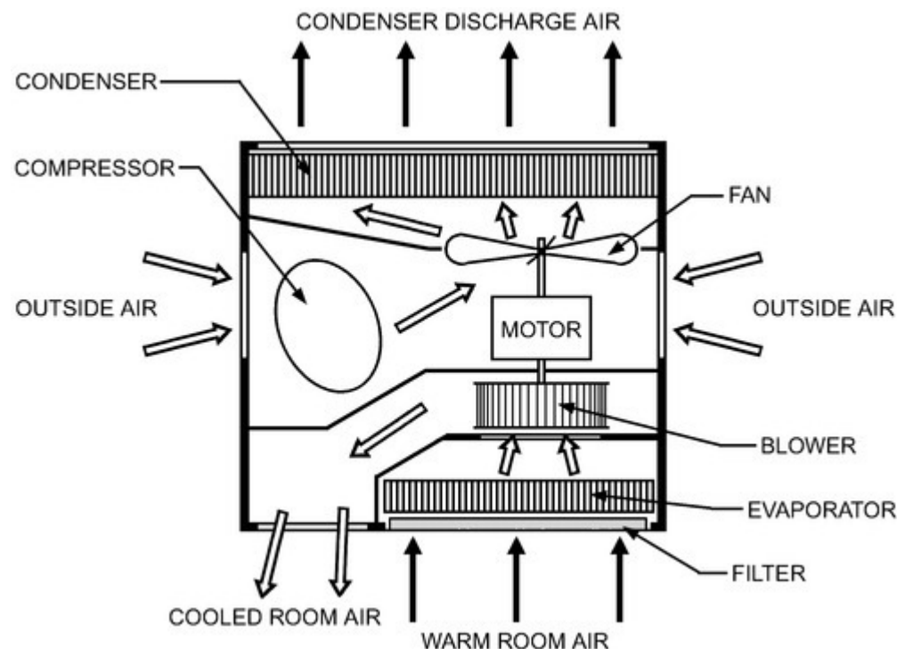
Figure 1. Schematic View of Typical Room Air Conditioner
