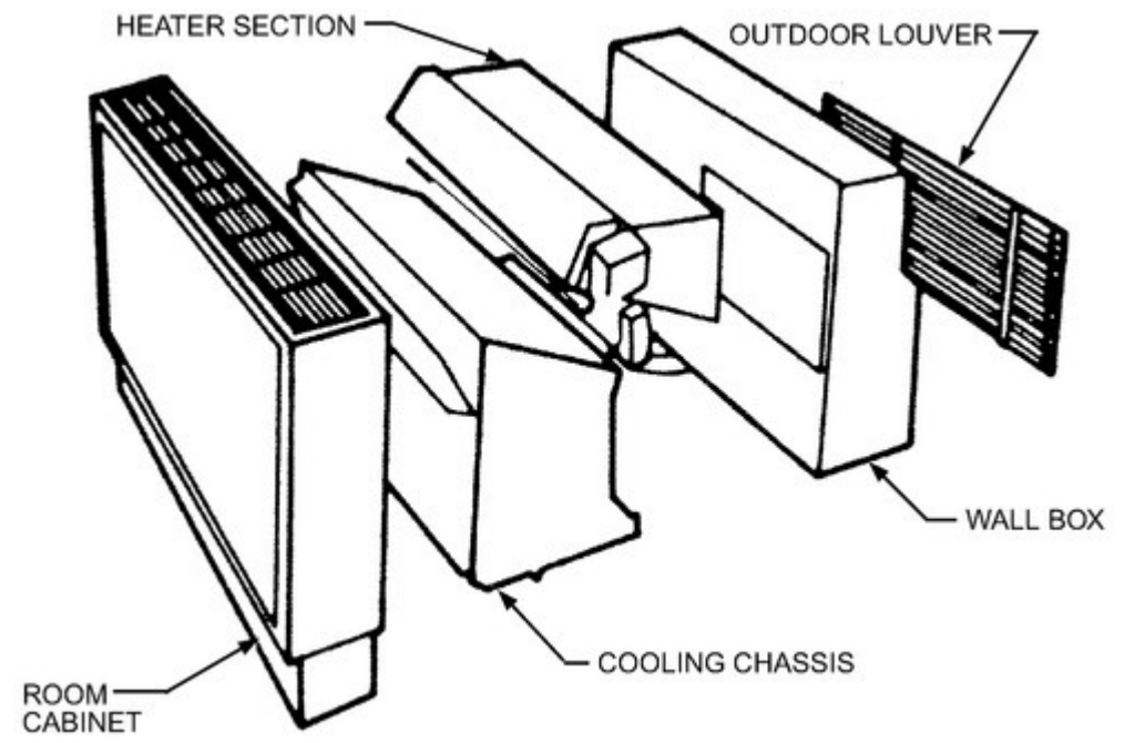
Figure 2. Sectional Packaged Terminal Air Conditioner
