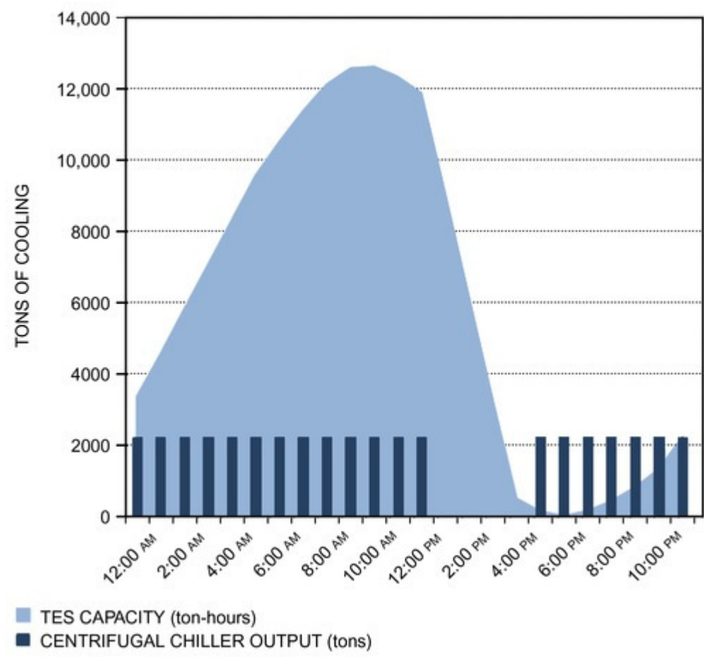
Figure 6. TES Tank Full-Storage Capacity (ton-hours) and Chiller Operation Output (tons)
