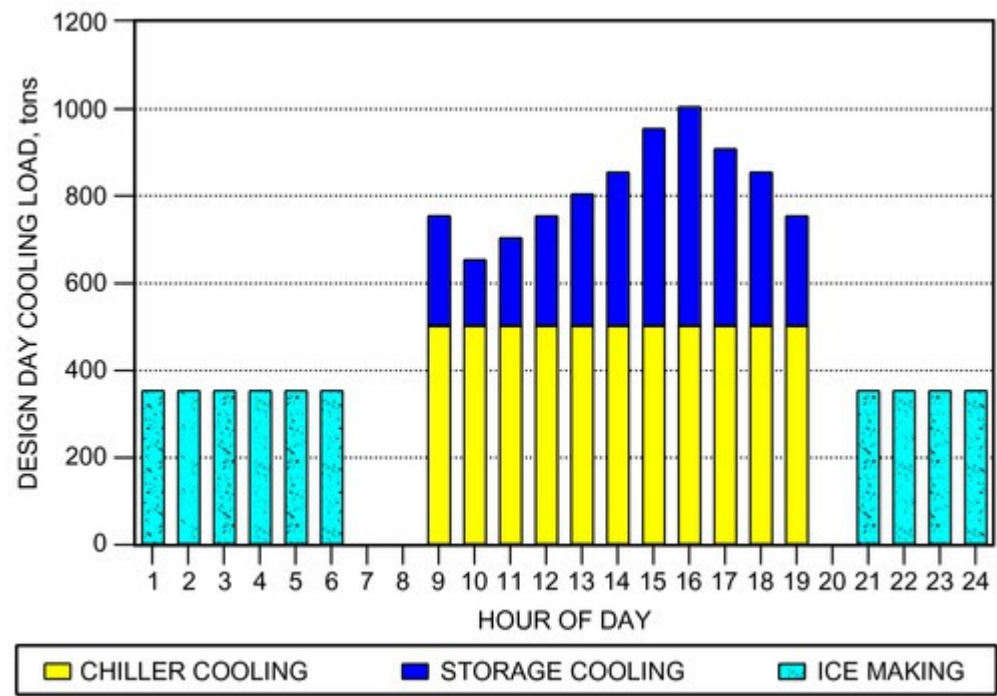
Figure 11. Minimum-Sized Chilled and Storage Contribution to Cooling Load
