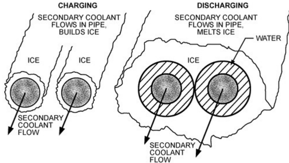
Figure 9. Charge and Discharge of Internal-Melt Ice Storage
