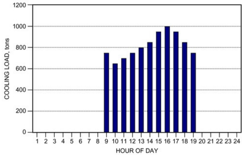
Figure 10. Design-Day Cooling Load
