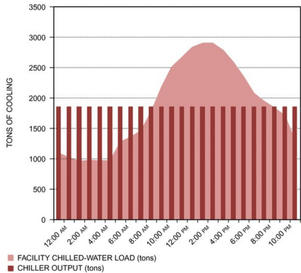
Figure 7. Cooling Load (tons) and Chiller Load (tons) with Partial-Storage TES Tank
