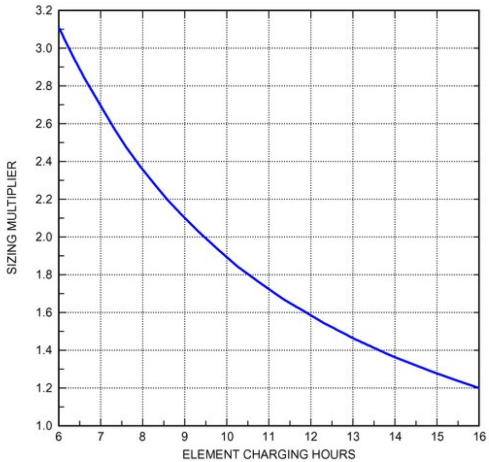
Figure 16. Representative Sizing Factor Selection Graph for Residential Storage Heaters
