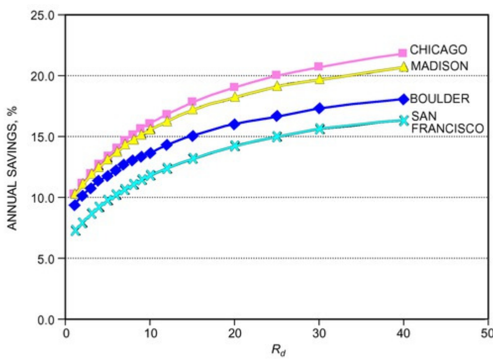
Figure 24. Annual Energy Cost Savings from Precooling, Relative to Conventional Controls, as Function of R_e
