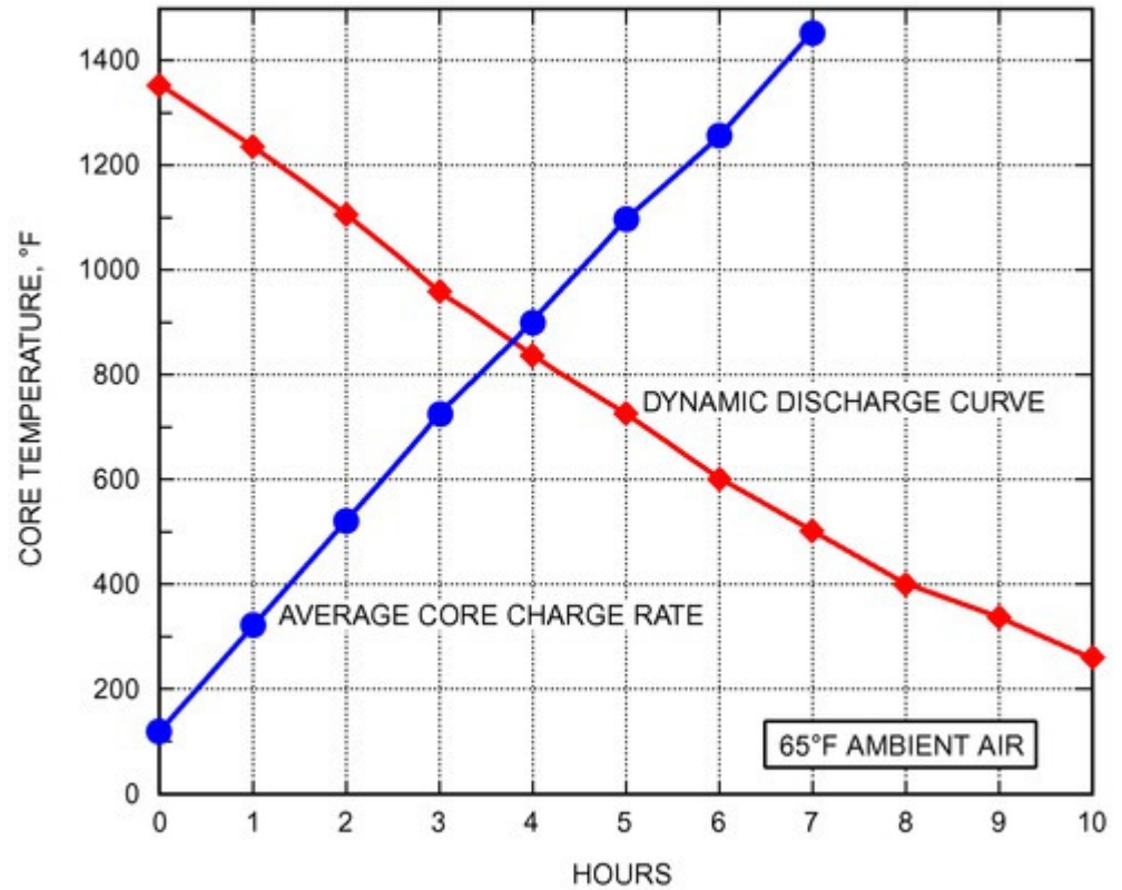
Figure 19. Room Storage Heater Dynamic Discharge and Charge Curves
