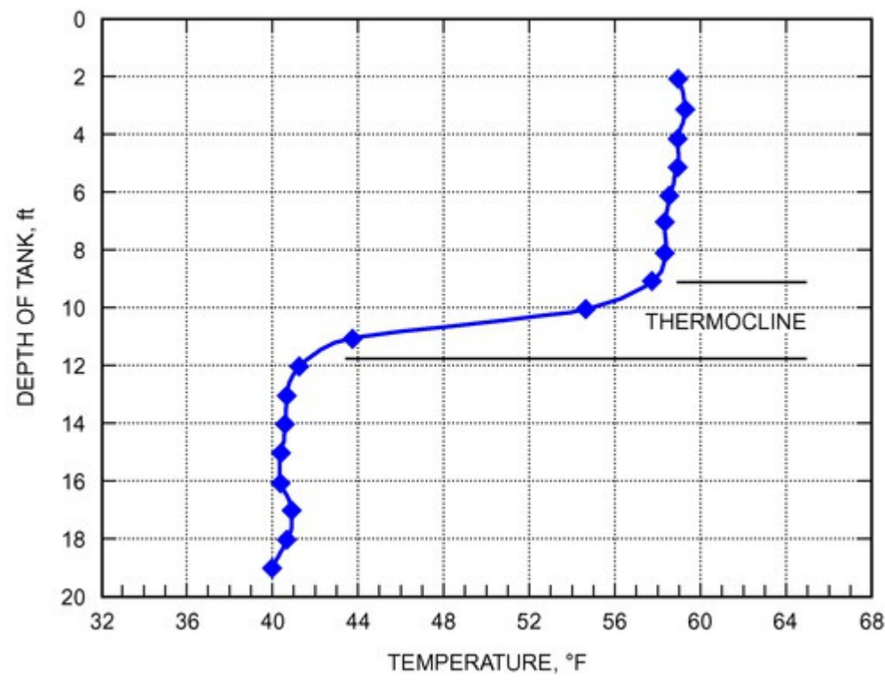
Figure 2. Typical Temperature Stratification Profile in Storage Tank
