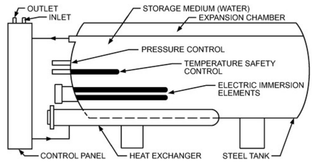
Figure 21. Pressurized Water Heater
