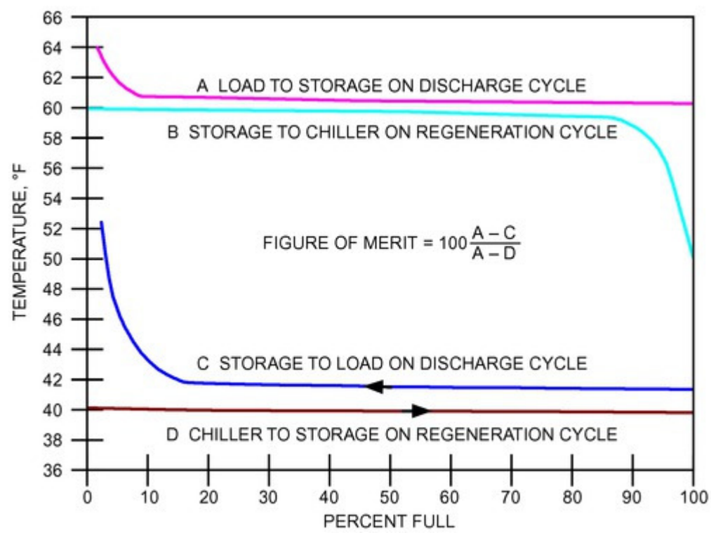
Figure 3. Typical Chilled-Water Storage Profiles
