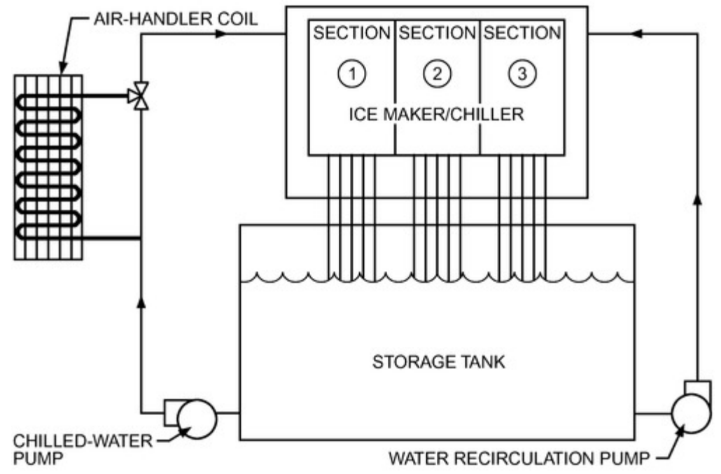
Figure 15. Ice-Harvesting Schematic (Courtesy Paul Mueller Company)
