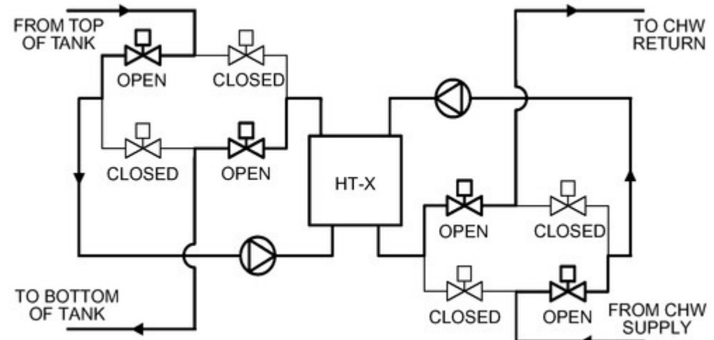
Figure 29. Charge Mode Status of Indirect Transfer Pumping Interface
