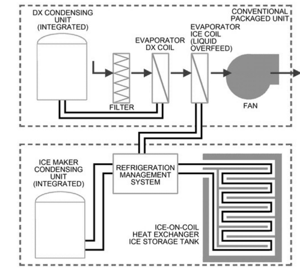
Figure 34. Typical UTSS with Packaged DX Equipment (Willis and Parsonnet 2010)
