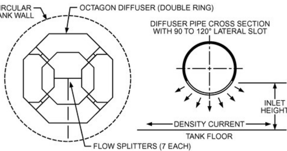
Figure 1. Typical Two-Ring Octagonal Slotted Pipe Diffuser
