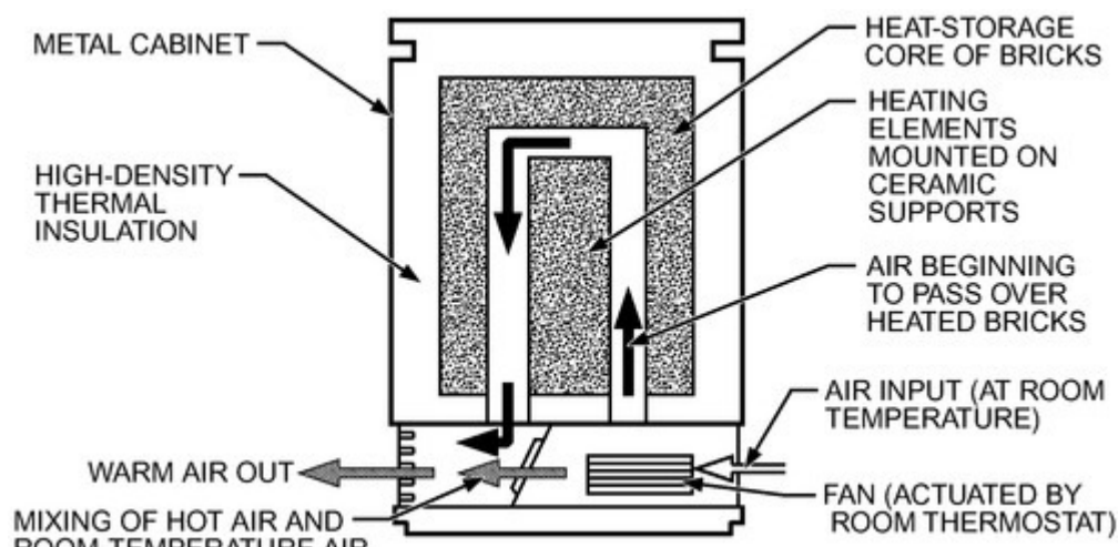
Figure 18. Room Storage Heater (Courtesy Steffes Corporation)
