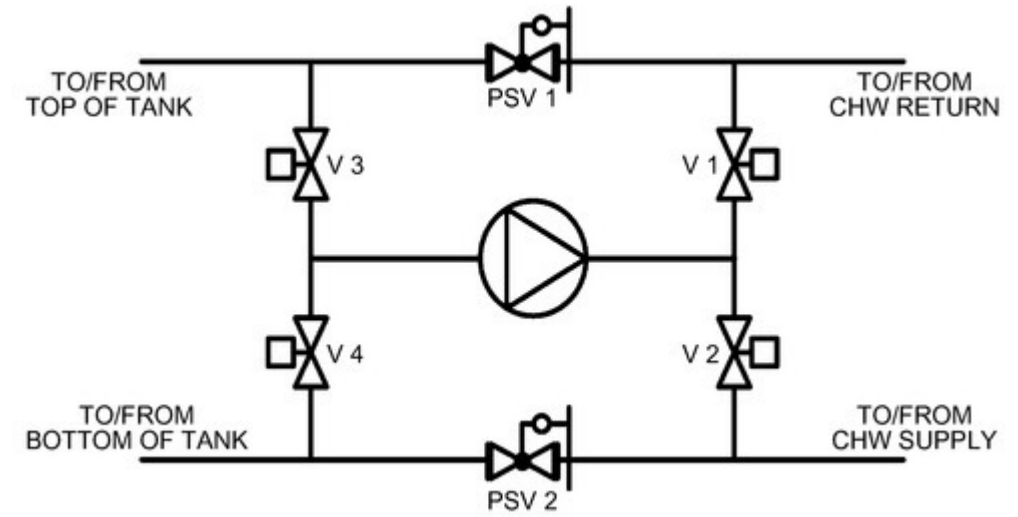
Figure 26. Direct Transfer Pumping Interface
