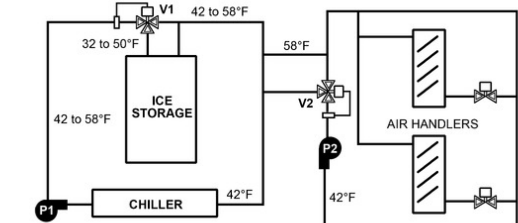
Figure 32. Series Flow, Chiller Downstream
