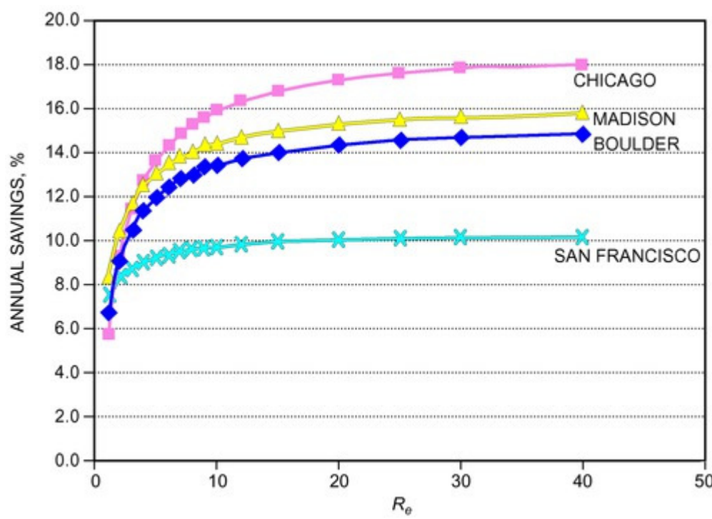
Figure 23. Annual Energy Cost Savings from Precooling, Relative to Conventional Controls, as Function of R_d
