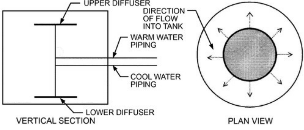
Figure 4. Radial Disk Diffuser
