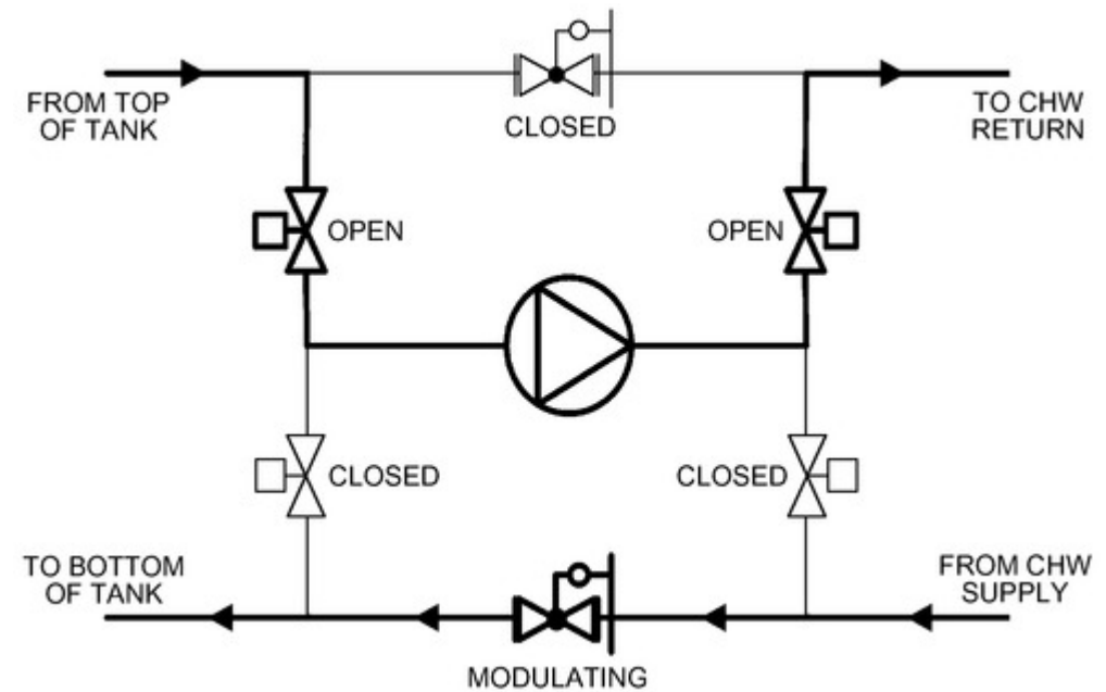
Figure 27. Charge Mode Status of Direct Transfer Pumping Interface
