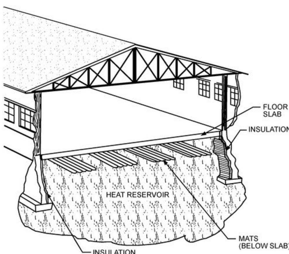
Figure 22. Underfloor Heat Storage
