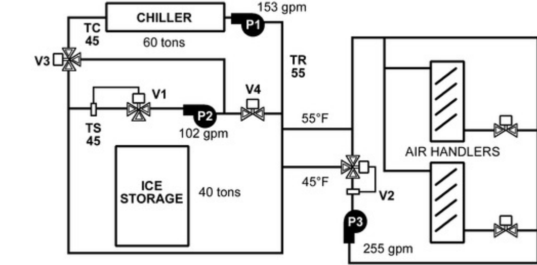
Figure 33. Parallel Flow for Chiller and Storage
