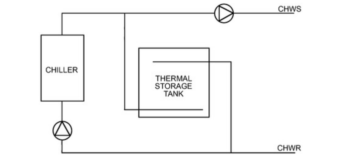
Figure 30. Primary/Secondary Chilled-Water Plant with Stratified Storage Tank as Decoupler
