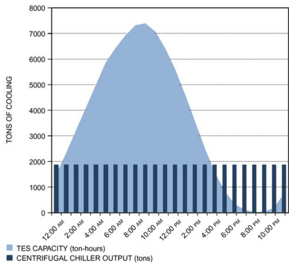
Figure 8. TES Tank Partial-Storage Capacity (ton-hours) and Chiller Operation Output (tons)
