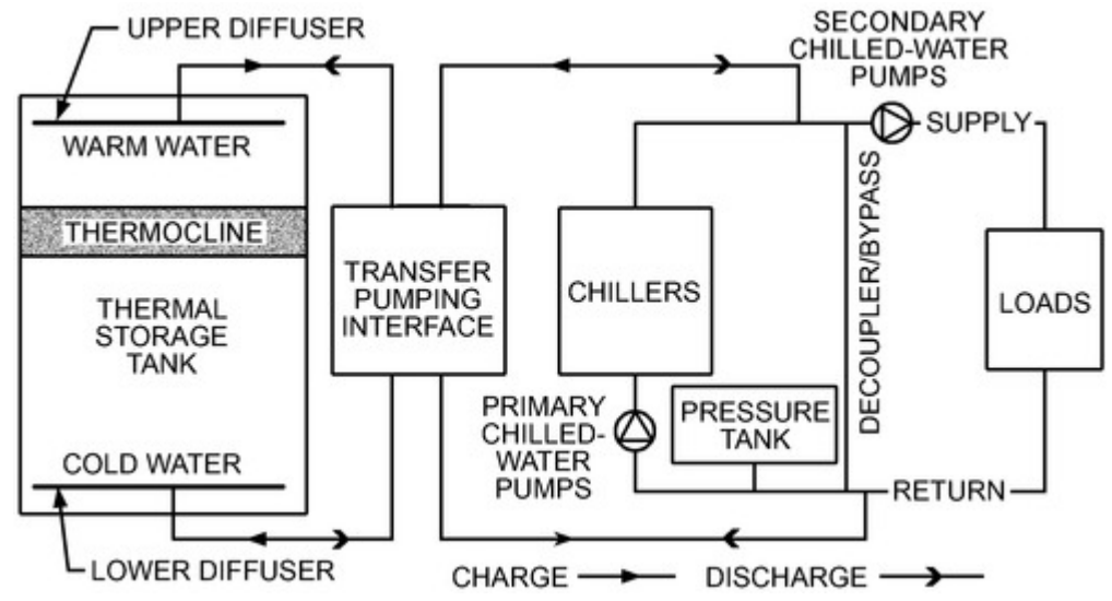
Figure 25. Typical Sensible Storage Connection Scheme
