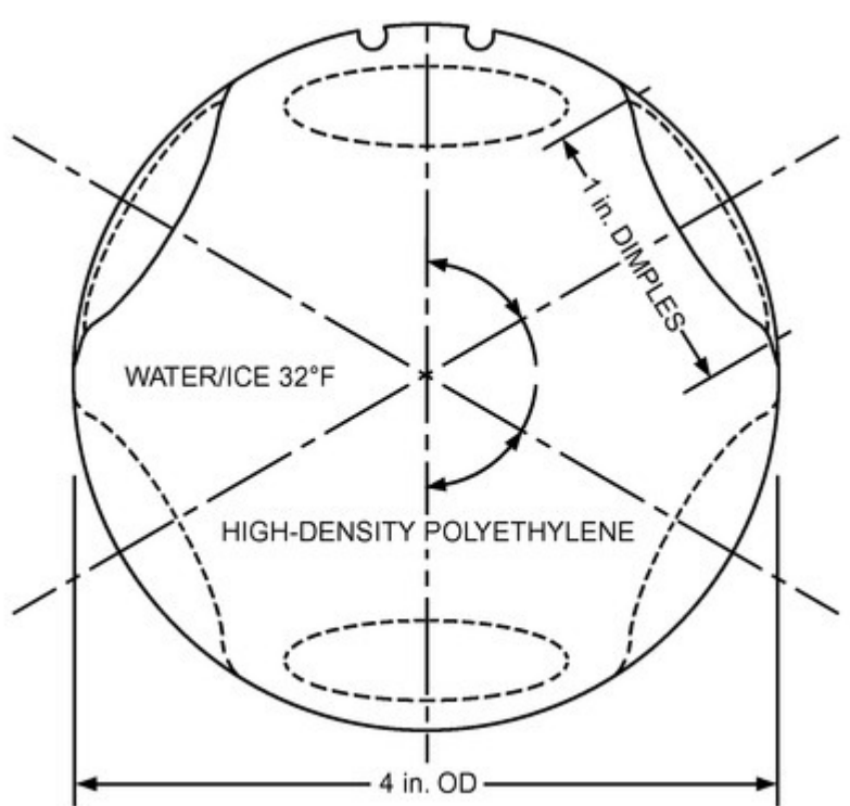
Figure 14. Encapsulated Ice: Spherical Container (Courtesy Cryogel)
