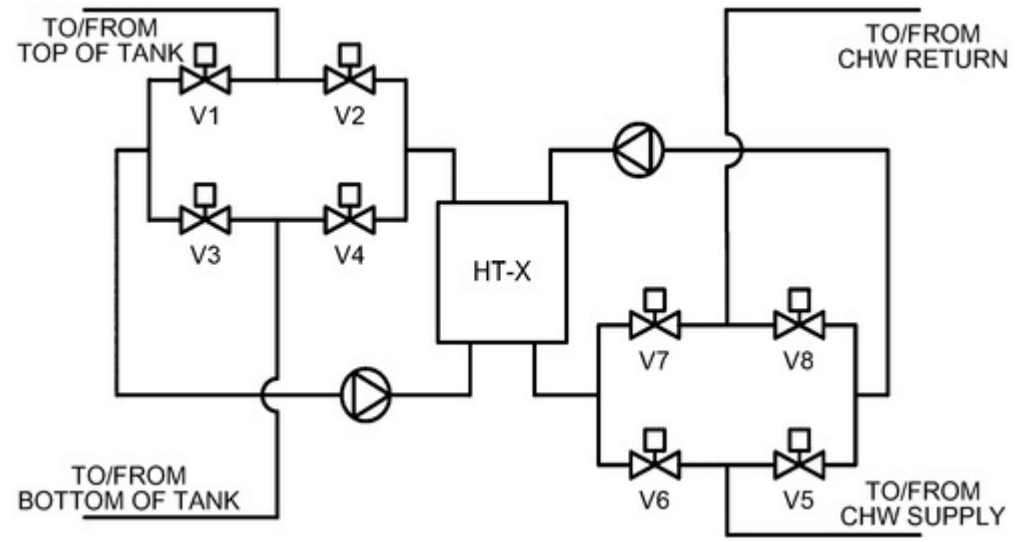
Figure 28. Indirect Transfer Pumping Interface
