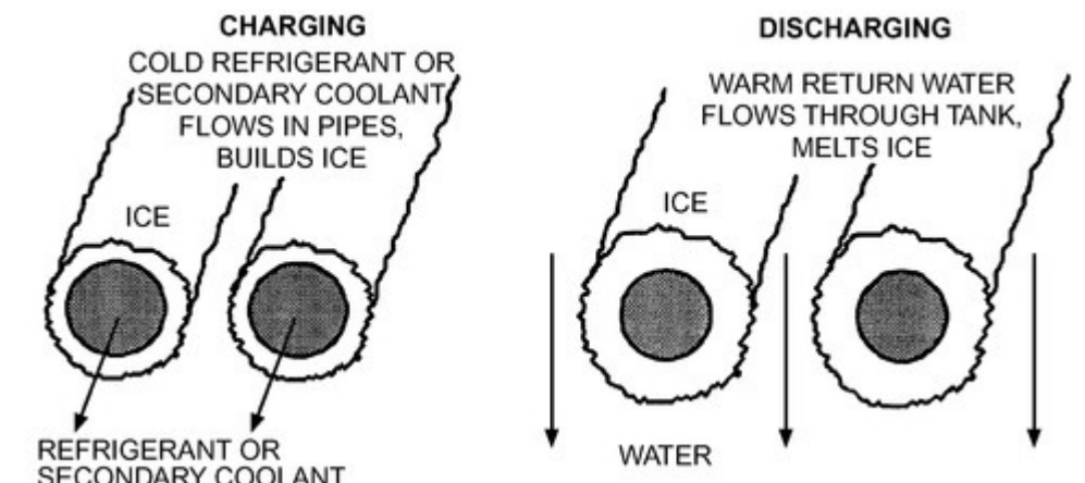
Figure 13. Charge and Discharge of External-Melt Ice Storage
