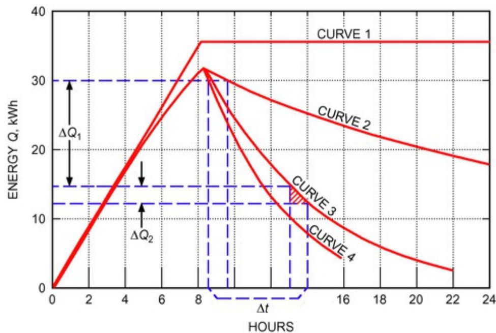
Figure 17. Typical Storage Heater Performance Characteristics (Hersh et al. 1982)
