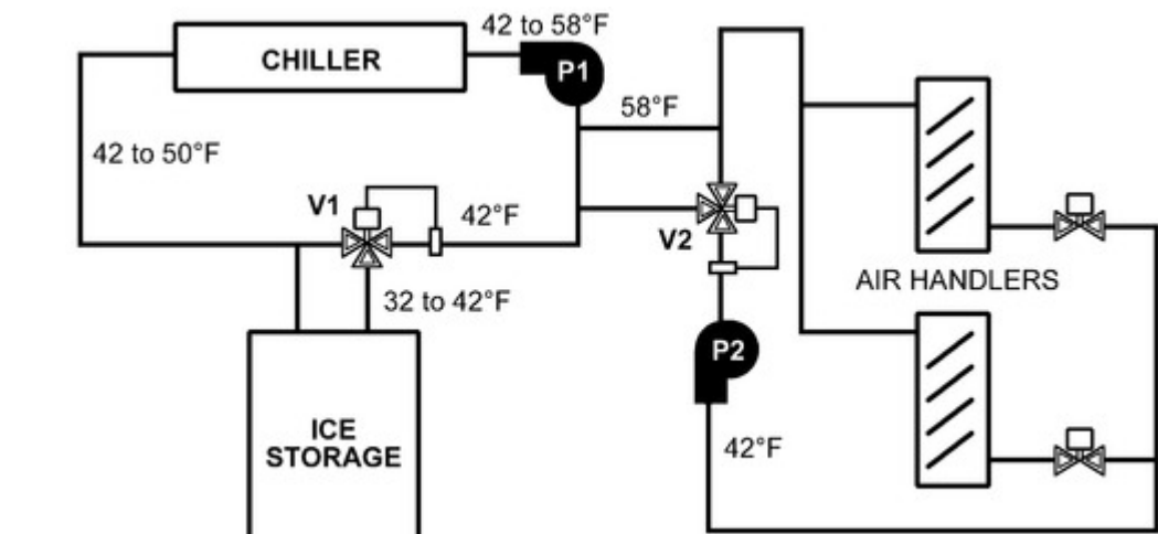
Figure 31. Series Flow, Chiller Upstream
