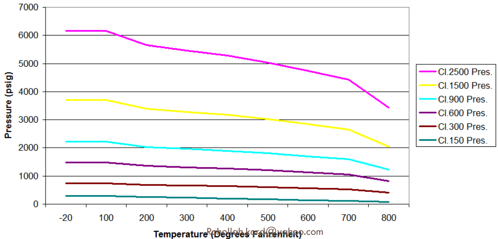
Pressure & Temperature ratings for Group 1.1 Material ASTM A105, A350 LF2 acc. to ASME B16.34
