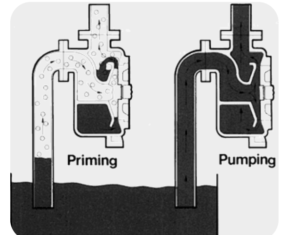
Self Priming Pump
