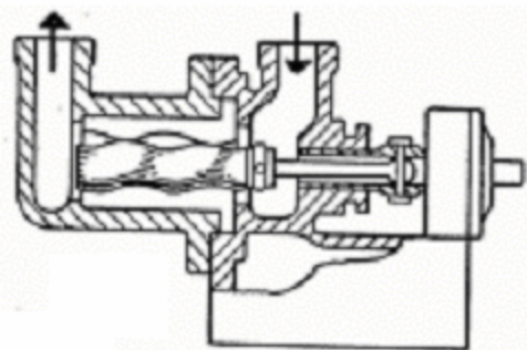
Single-screw pump.
