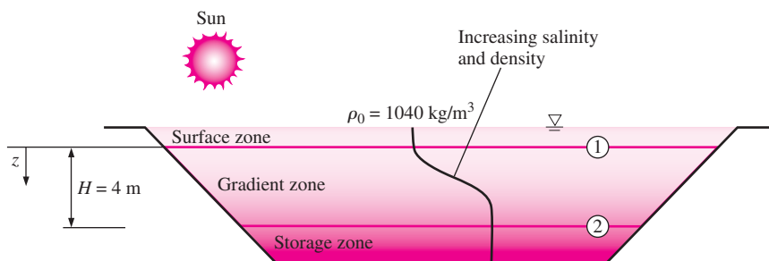
FIGURE 1-55 Schematic for Example 1-10.
