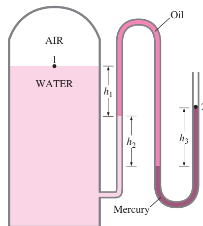
FIGURE 1-61 Schematic for Example 1-12.
