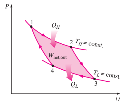
FIGURE 6–38 P - V diagram of the Carnot cycle.
