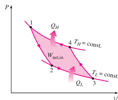
FIGURE 6–39 P - V diagram of the reversed Carnot cycle.
