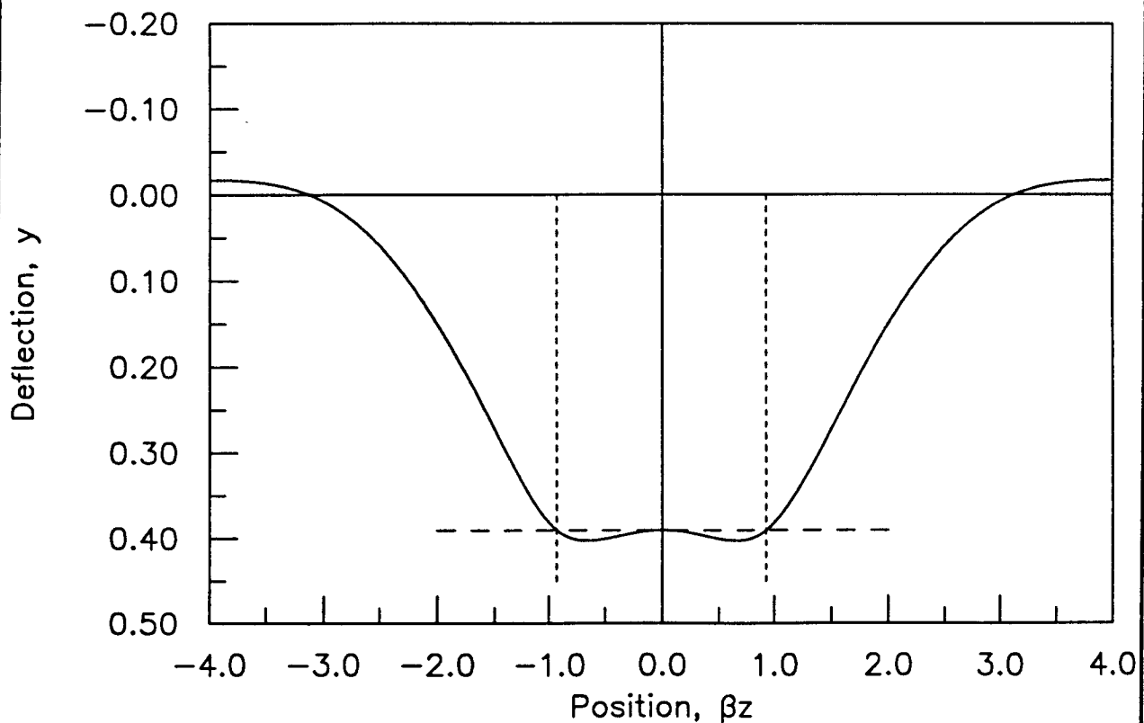
c) Deflection Plot, Problem 10.9
