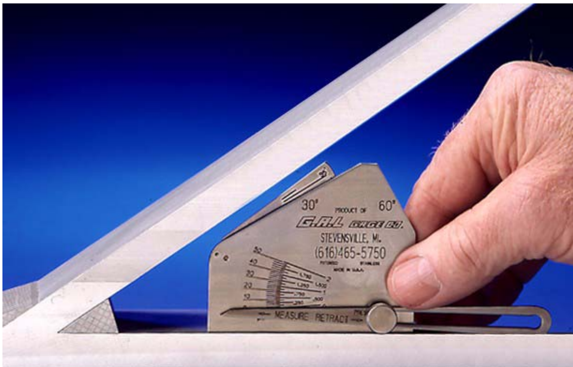
Figure 16—Skew—T Fillet Weld Gauge
