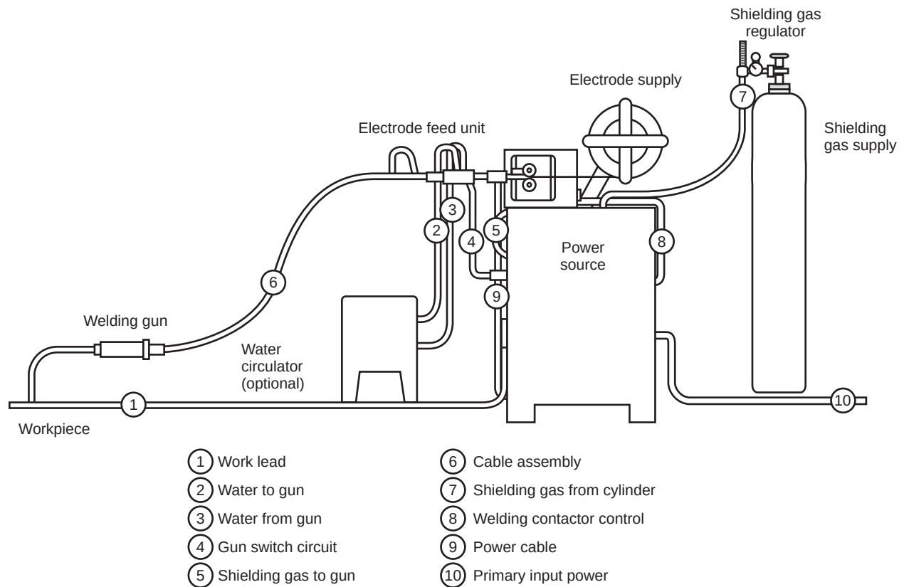
Figure 5—GMAW Equipment
