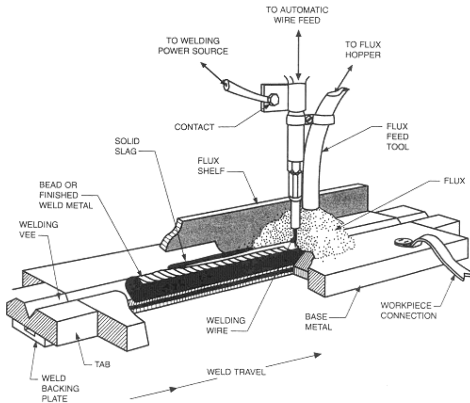
Figure 10—SAW Welding
