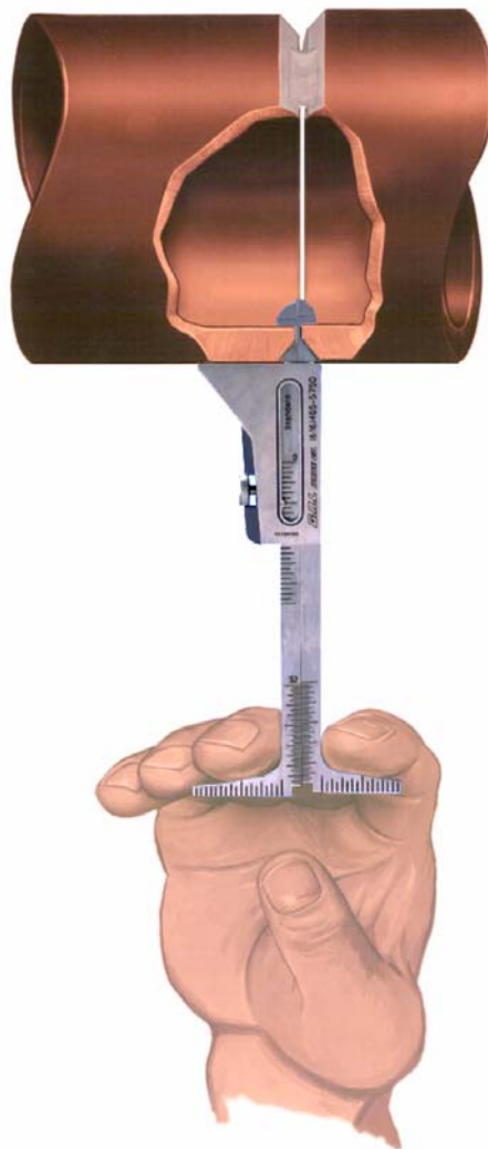
Figure 20—Hi-lo Gauge
