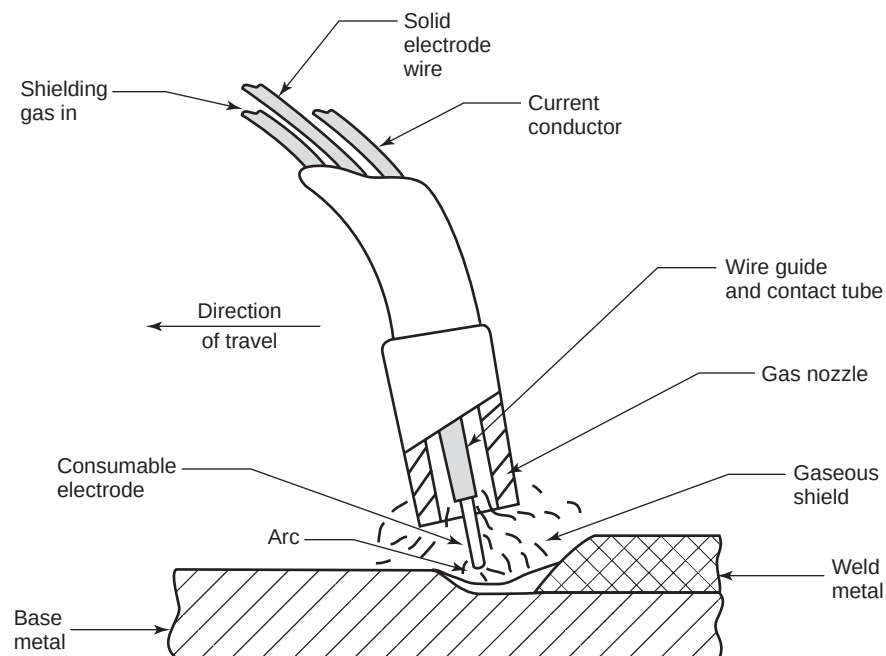
Figure 6—GMAW Welding
