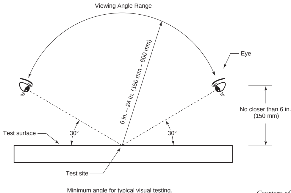
Figure 12—Direct Visual Examination Requirements
