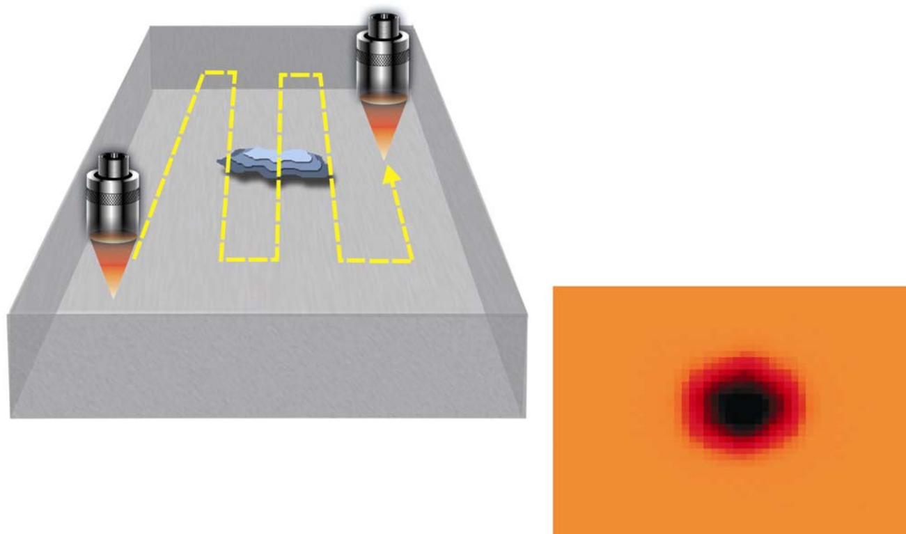
Figure 47—C-scan
