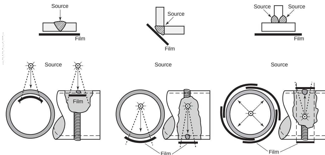
Figure 31—Single-wall Techniques
