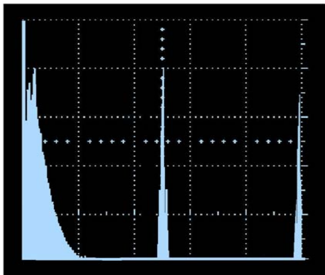
Figure 45—A-scan
