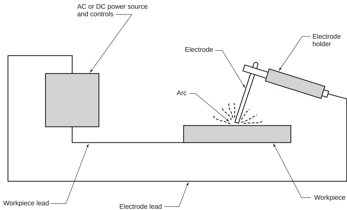
Figure 1—SMAW Welding
