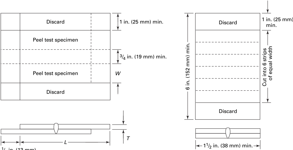
(b) Metallurgical Examination Coupon and Transverse Specimens
