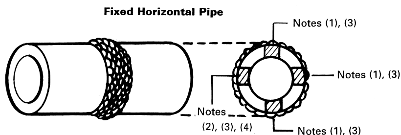
Test Specimen Location for 5G Overlay Qualification (Specimens Required From a Minimum of Three Locations)
