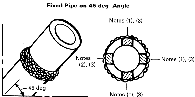
Test Specimen Location for 6G Overlay Qualification (Specimens Required From a Minimum of Three Locations)
