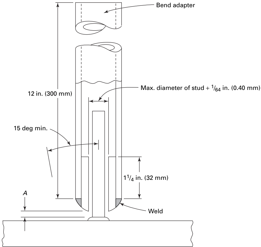
QW-466.4 STUD-WELD BEND JIG
