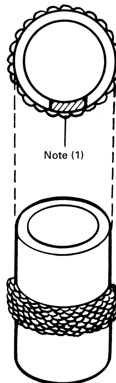
Test Specimen Location for 2G and 1G Rotated Overlay Qualification (Specimens Required From One Location)
