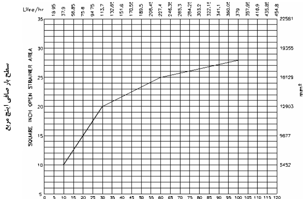
Fig. 11-STRAINER AREA FOR* NOS. 4, 5, 6 FUEL OIL
