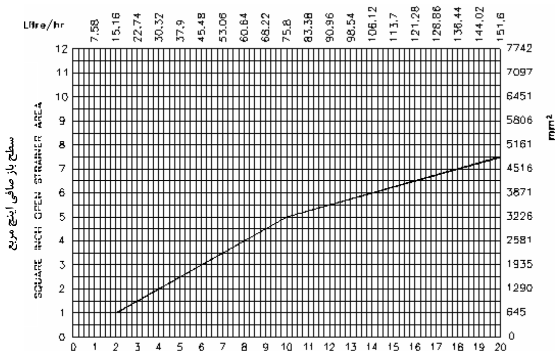
Fig. 9-STRAINER AREA FOR* No. 1 FUEL OIL
