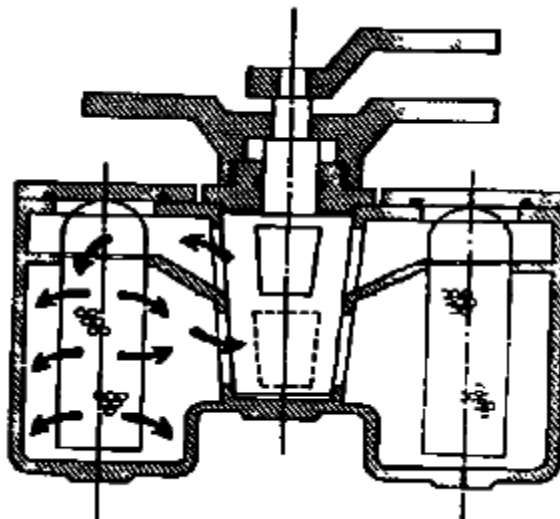
Fig. 5-DUAL IN-LINE STRAINER (SCHEMATIC)
