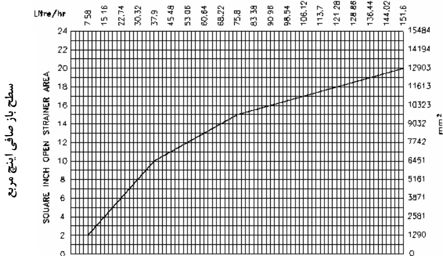
Fig. 10-STRAINER AREA FOR* No. 2 FUEL OIL
