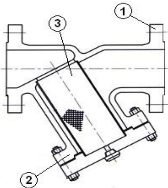
FLANGED STRAINER
