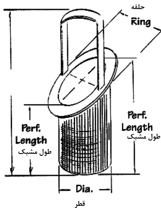
Fig. 3-FILTER DETAIL
