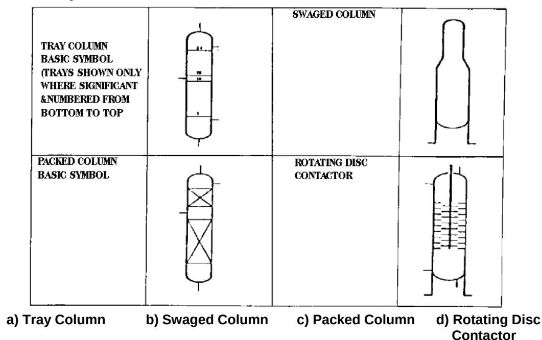
COLUMN SYMBOLS
