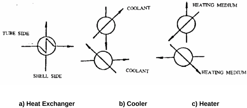
SHELL AND TUBE TYPE HEAT EXCHANGER SYMBOLS
