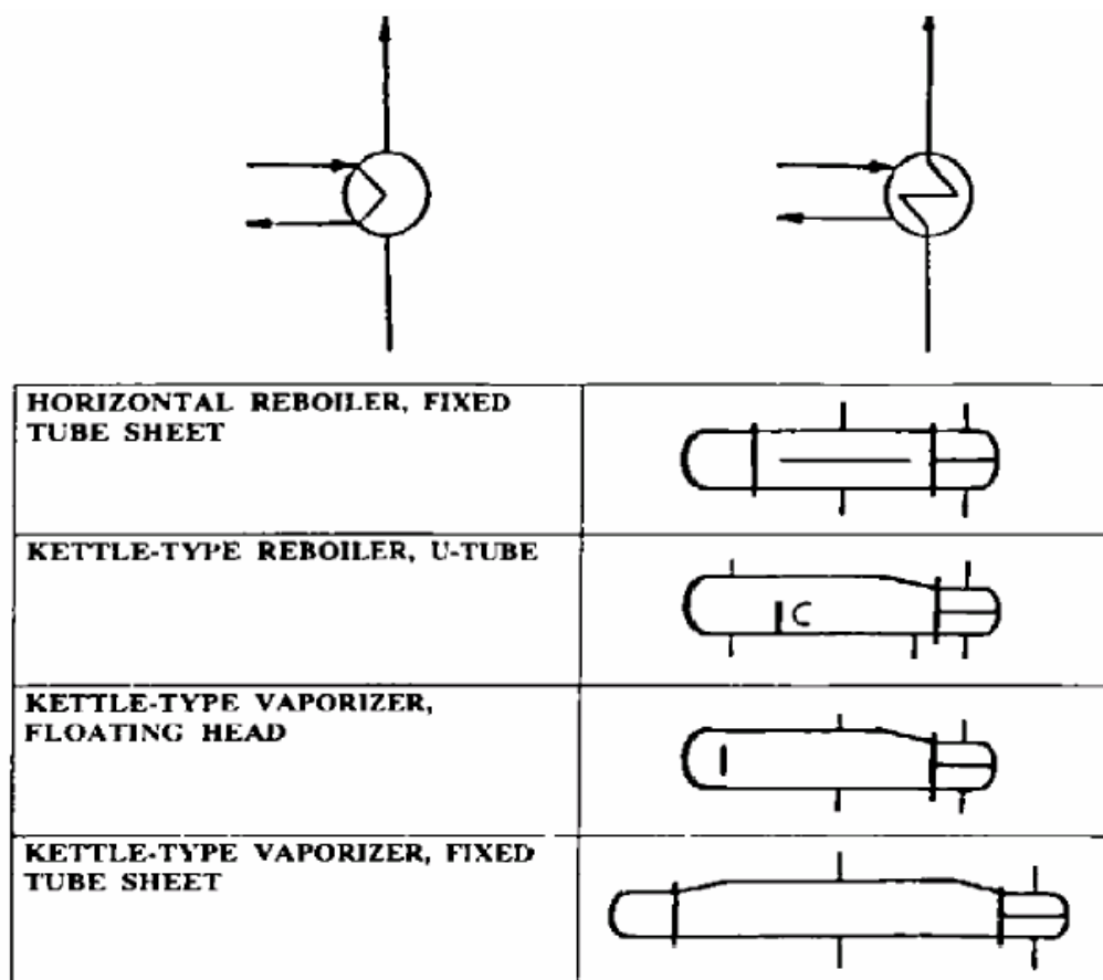
REBOILER SYMBOLS
