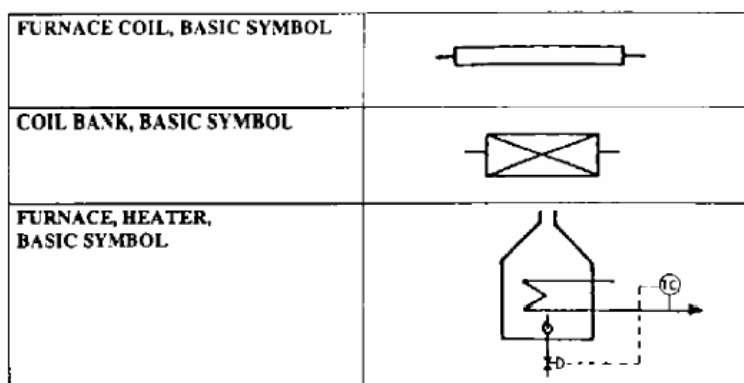
FURNACE SYMBOLS
