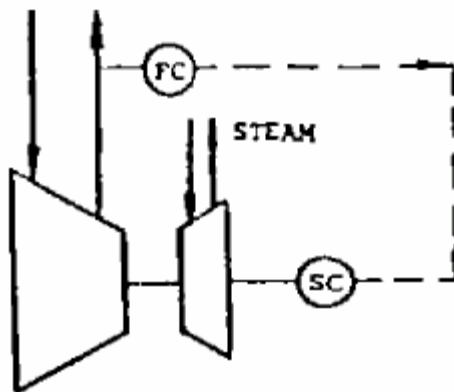
Compressor Turbine
