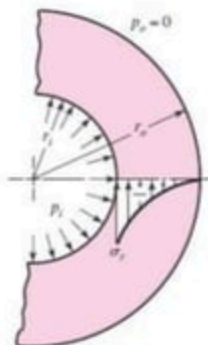
(b) Radial stress distribution
