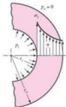
(a) Tangential stress distribution
