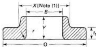
Lapped
