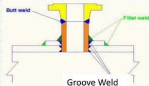
Figure 1 Butt weld with full penetration
