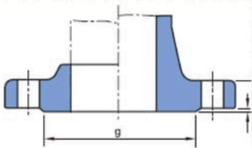
RAISED FACE (LARGE)
