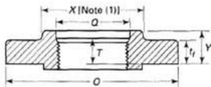
Threaded (NPS 1/2 to 2 1/2 Only)
