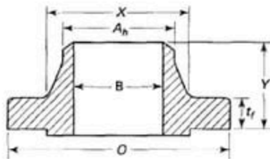
Welding Neck
