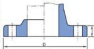
FLAT FACE
