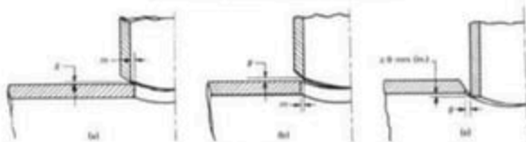
Fig. 328.A.4 Preparation for Branch Connections
