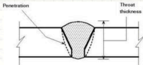
Figure 1 Butt weld with full penetration
