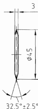
Figure 3 — Circular blade specifications
