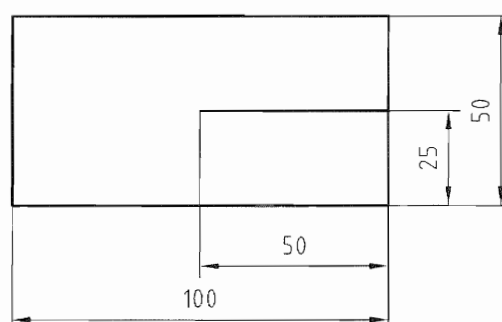
Figure 4 — Test piece
